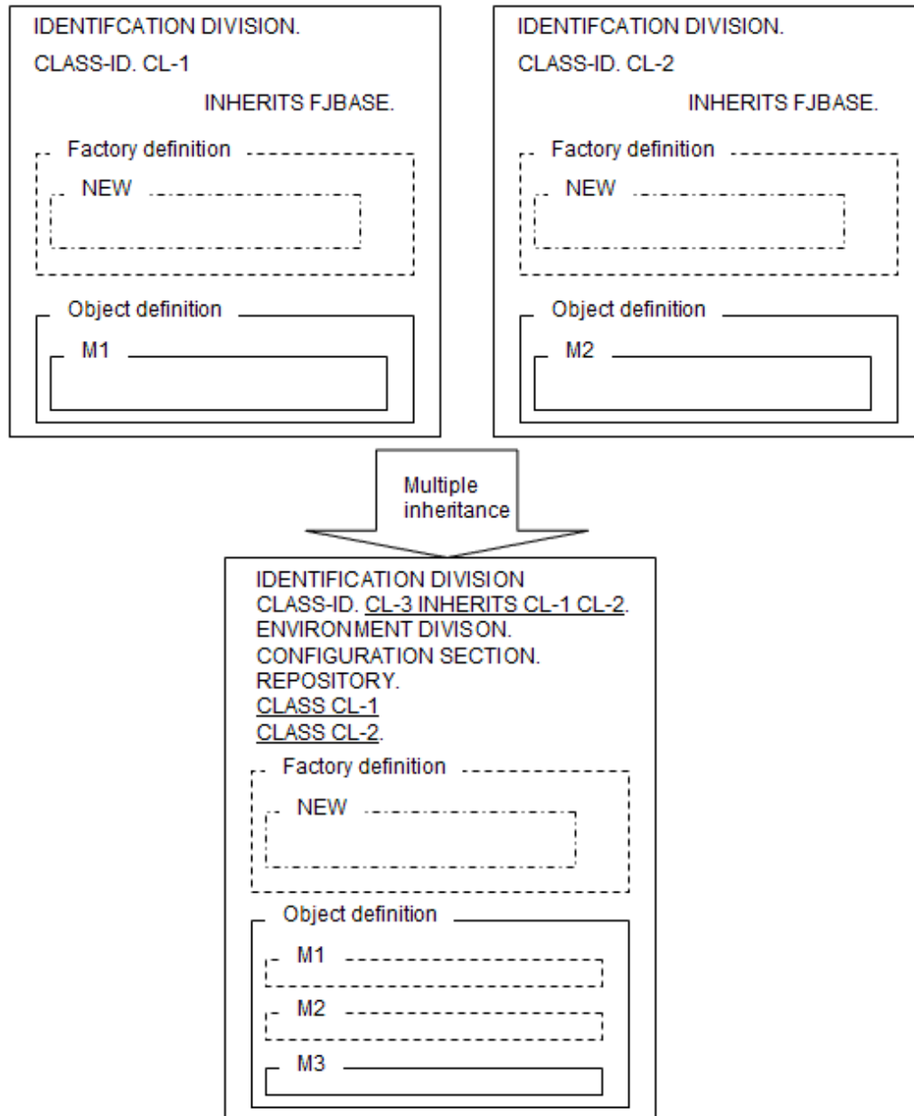
Figure 14.26 Multiple inheritance
