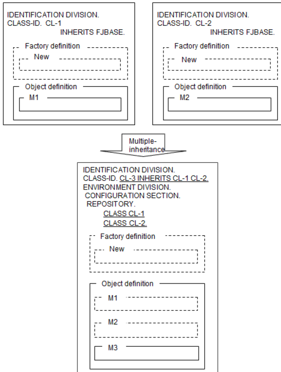
Figure 14.19 Multiple Inheritance
