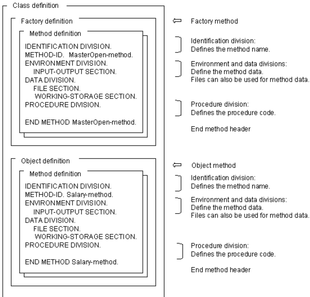
Figure 14.8 Method definitions
