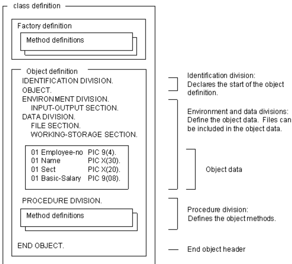
Figure 14.6 Object source structure
