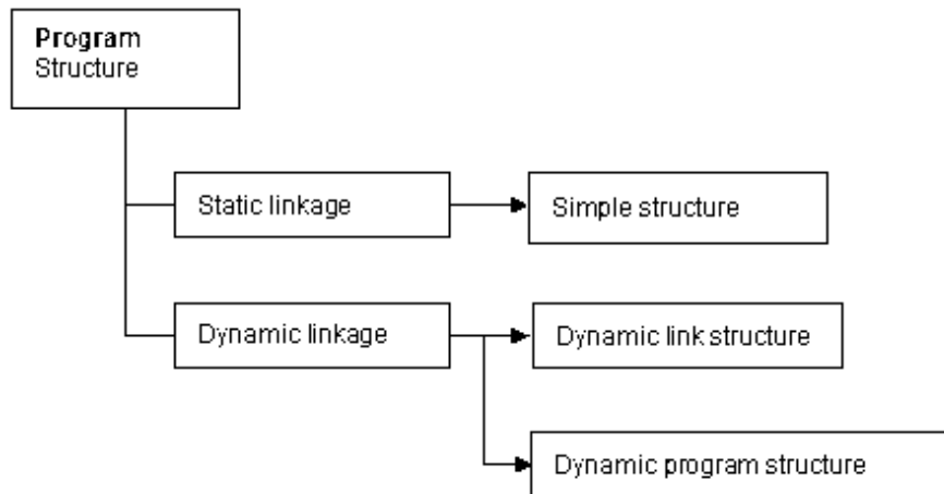
Figure 4.1 Program Structure
