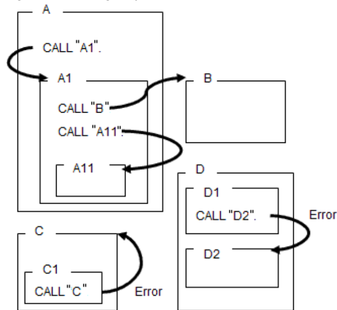
Figure 9.9 Calling sequence
