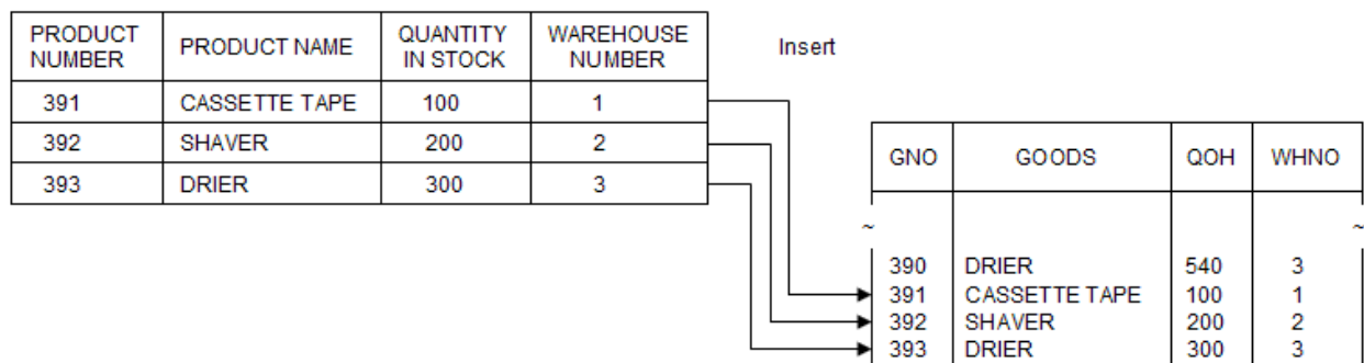
Figure 17.2 STOCK TABLE
