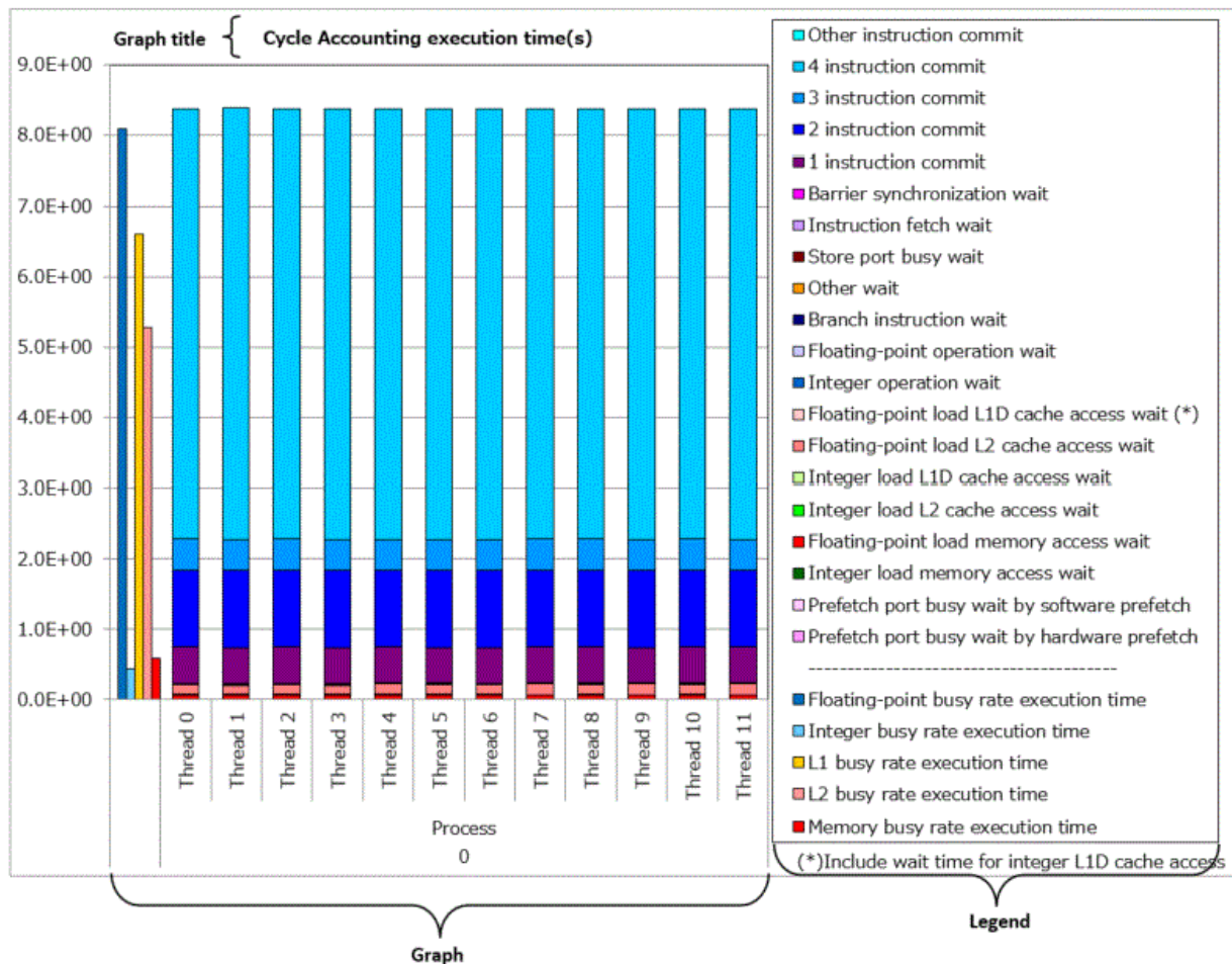
Figure 4.7 Graph structure
