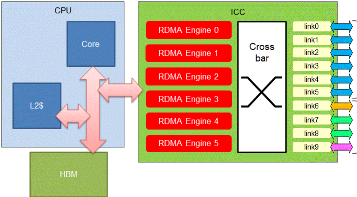
Figure 6.4 ICC configuration
