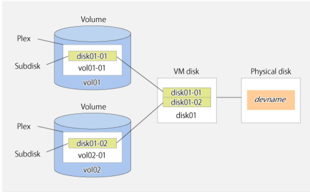
Figure 1.3 Relationships Between Volumes, VM Disks and Physical Disks (2)
