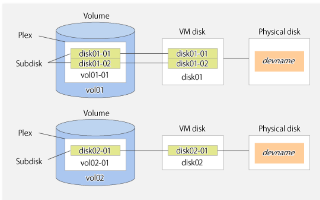
Figure 1.2 Relationships Between Volumes, VM Disks and Physical Disks (1)
