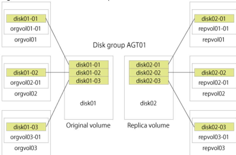
Figure 6.53 Volume Structure Example
