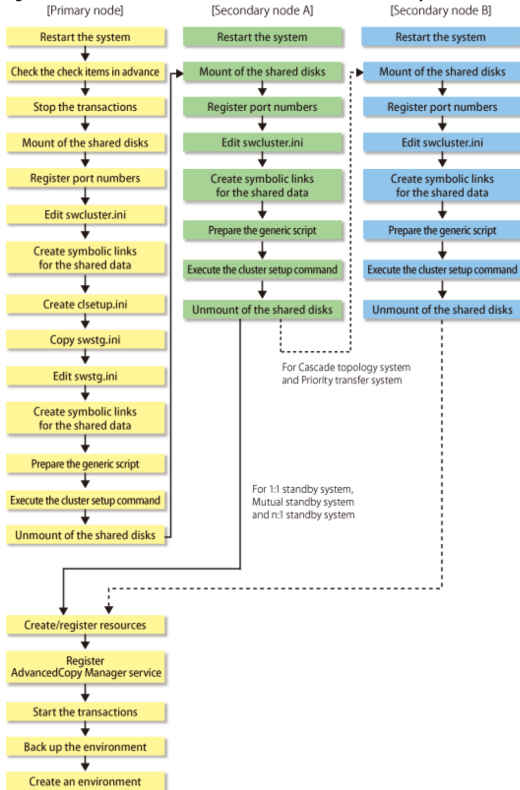
Figure 8.2 Customization Flow for Solaris/Linux/HP-UX Clustered System
