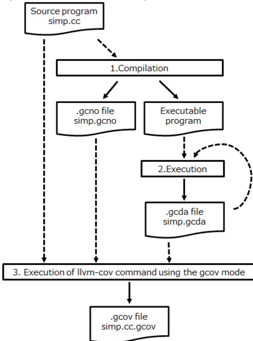
Figure E.1 Procedure of the code coverage
