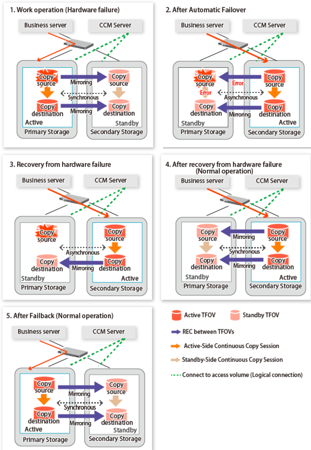
Figure 3.26 When Automatic Failover Is Performed Due to Hardware Failure Occuring on Primary Storage Where TFO Status Is "Active"
