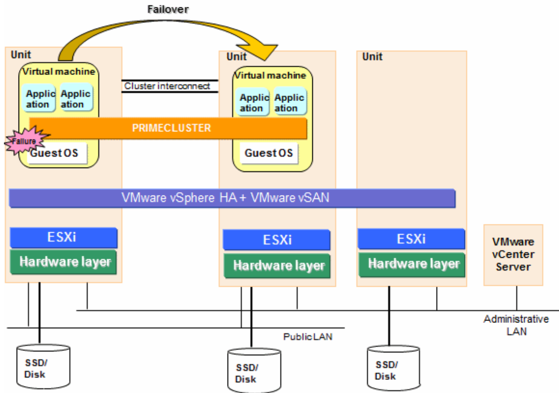
Figure G.2 Cluster Systems in a VMware Environment (VMware vCenter Server functional cooperation + VMware vSphere HA + vSAN)
