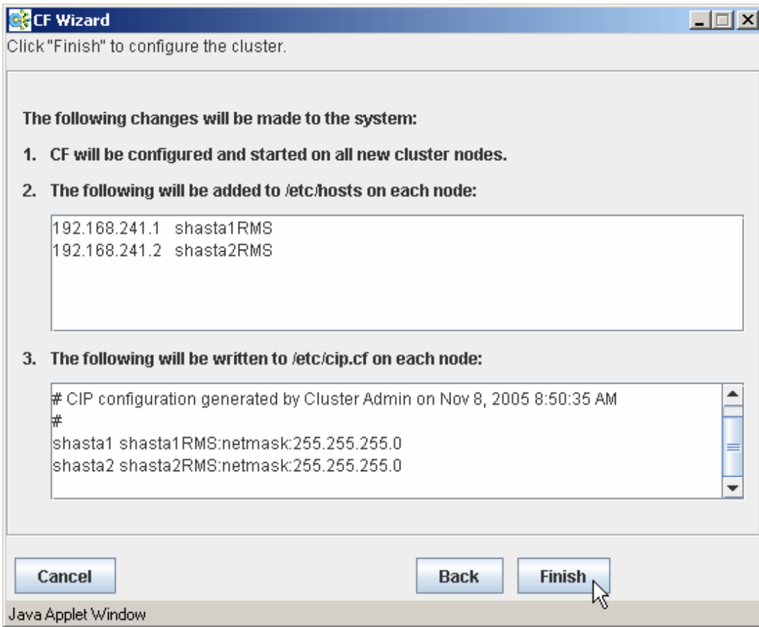
Figure 1.22 Summary window
