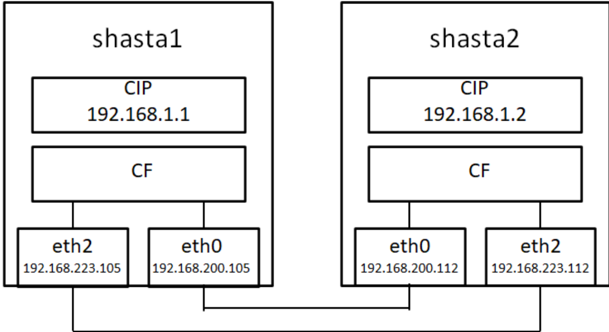
Figure 1.2 CIP diagram (CF over IP)
