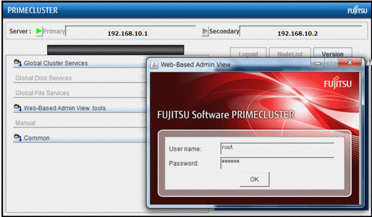
Figure 1.3 Login pop-up
