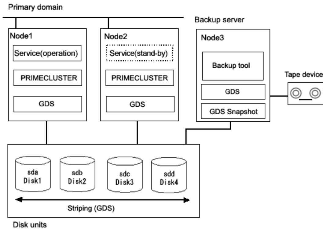
Figure 7.70 System Configuration
