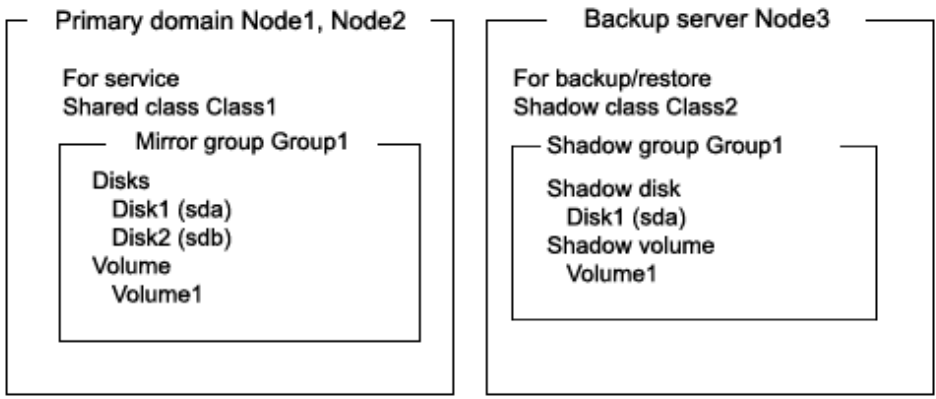
Figure 7.84 Object Configuration When Backing Up
