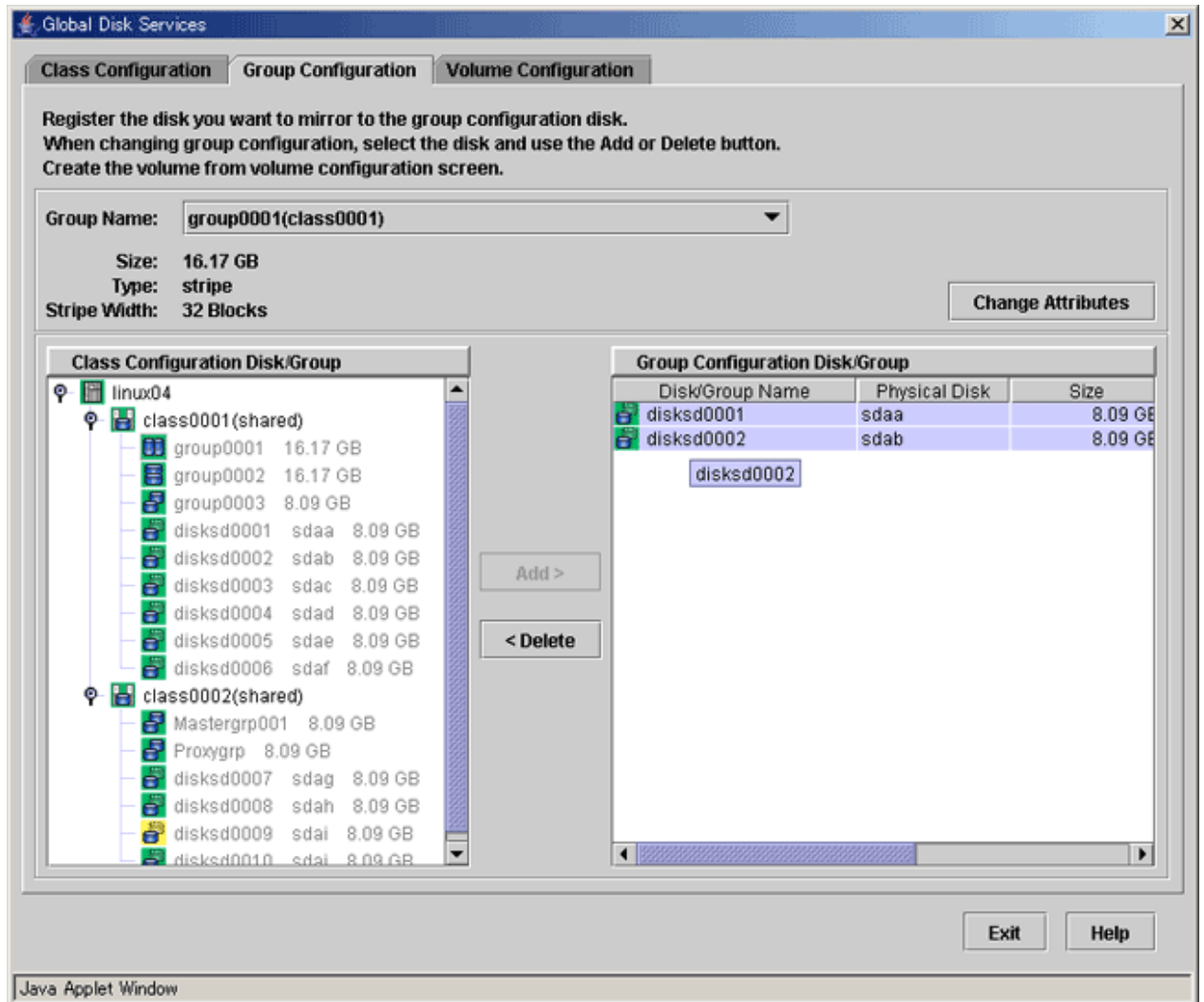
Figure 9.7 Disconnecting Disk/Lower level group
