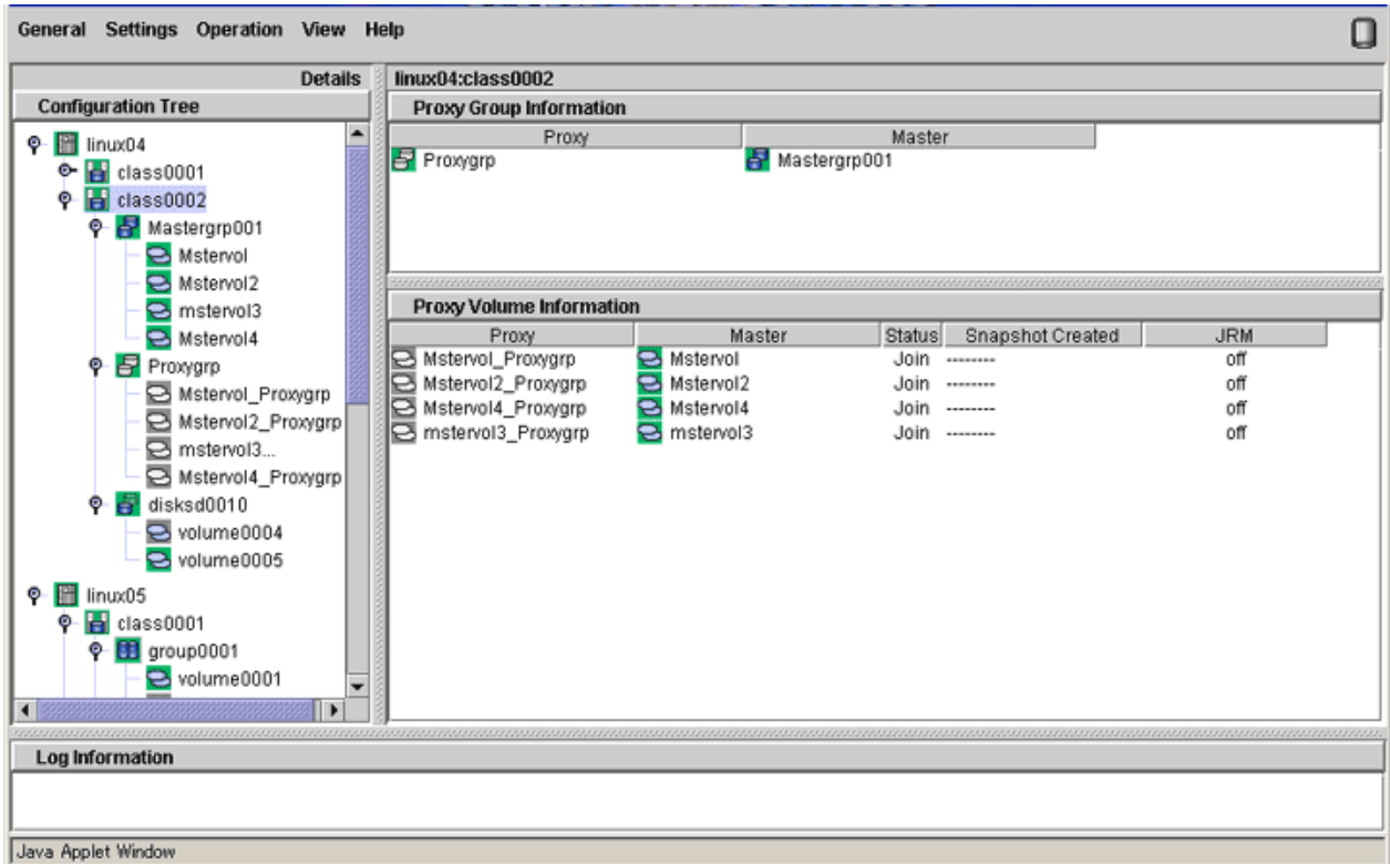
Figure 7.8 Main Screen (for Proxy Objects of a Class)
