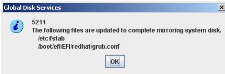
Figure 6.8 Setting System Disk Mirroring Complete
