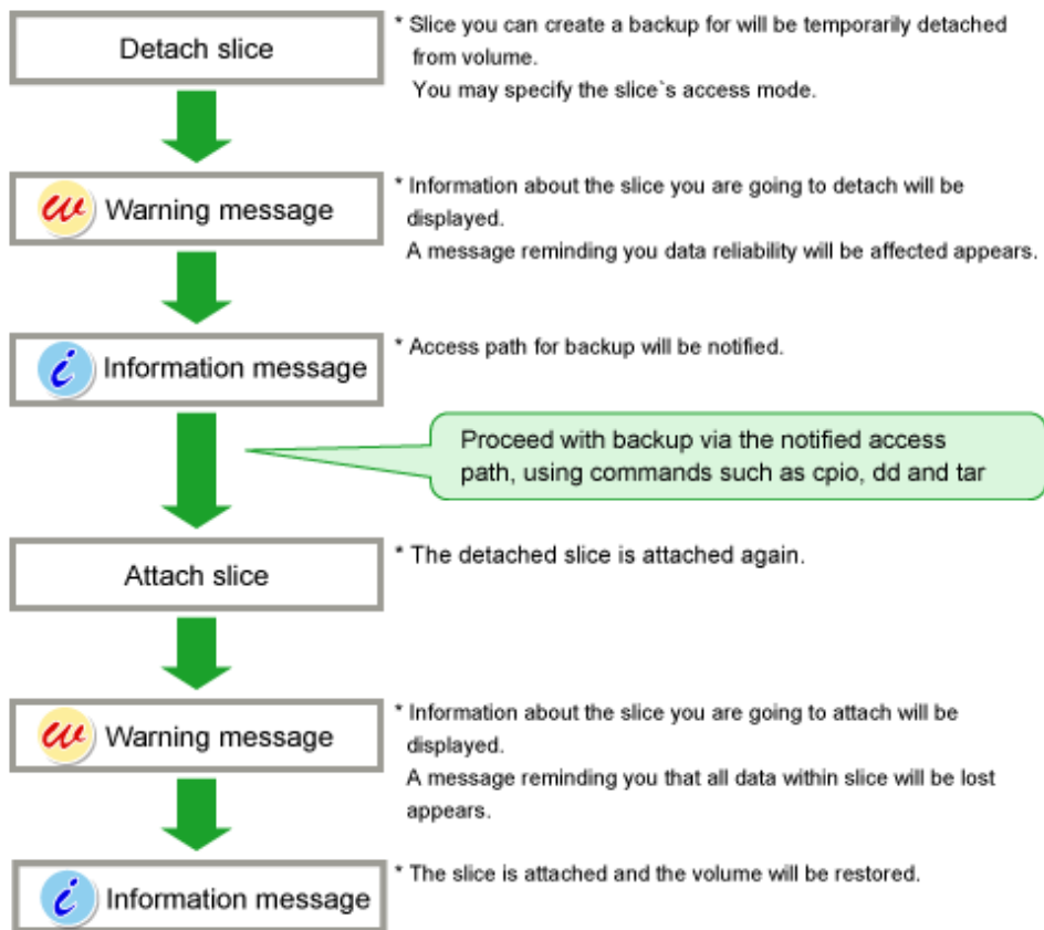
Figure 7.38 Backup Operation (by Slice Detachment)
