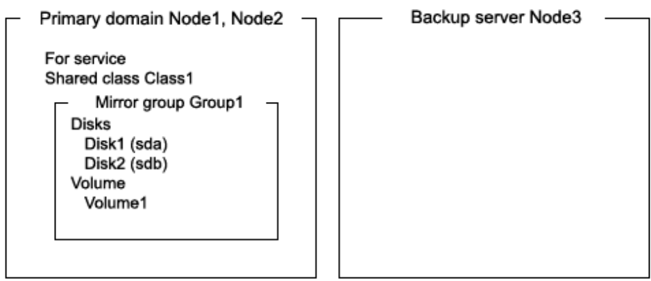
Figure 7.82 Object Configuration in Normal Operation
