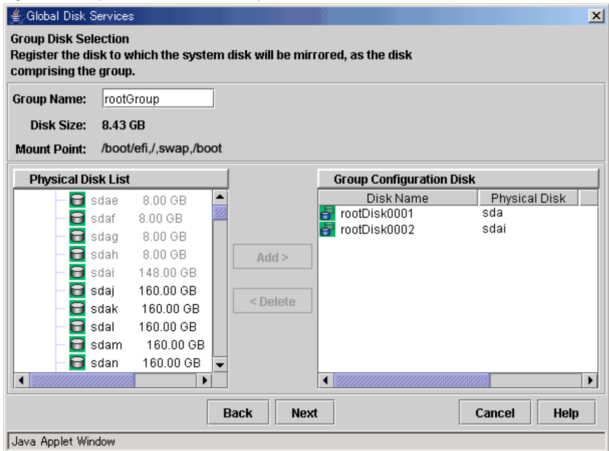
Figure 6.5 Group Disk Selection: rootGroup
