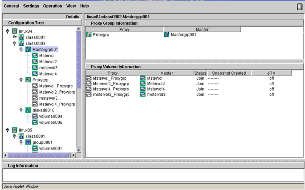
Figure 7.9 Main Screen (for Proxy Objects of a Group)
