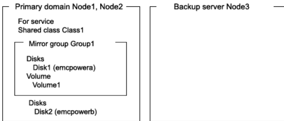
Figure 7.113 Object Configuration When Backing Up from BCV
