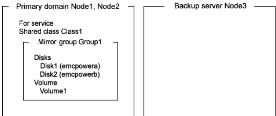
Figure 7.108 Object Configuration in Normal Operation
