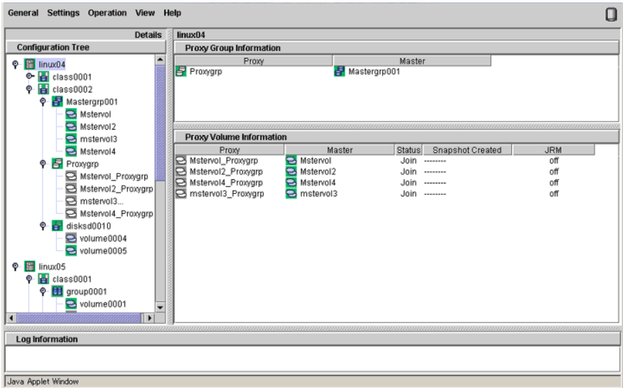
Figure 7.7 Main Screen (for Proxy Objects of a Node)
