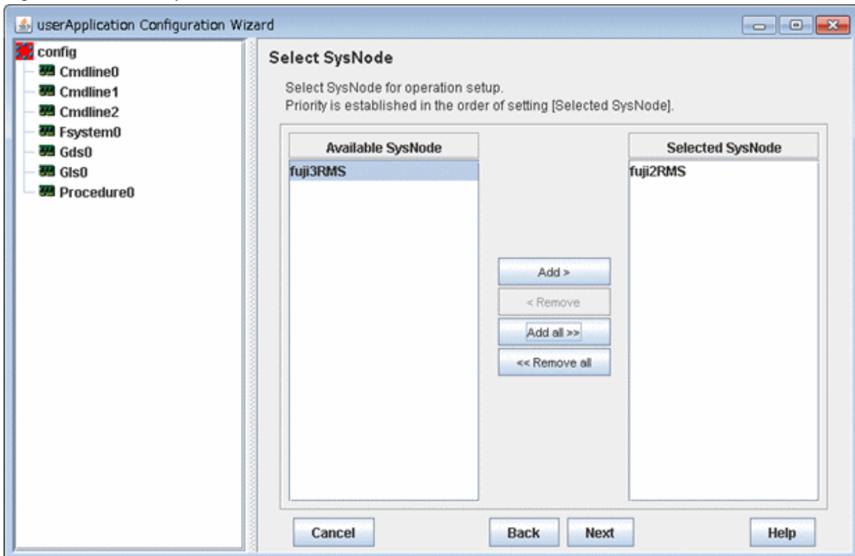
Figure 6.51 Select SysNode
