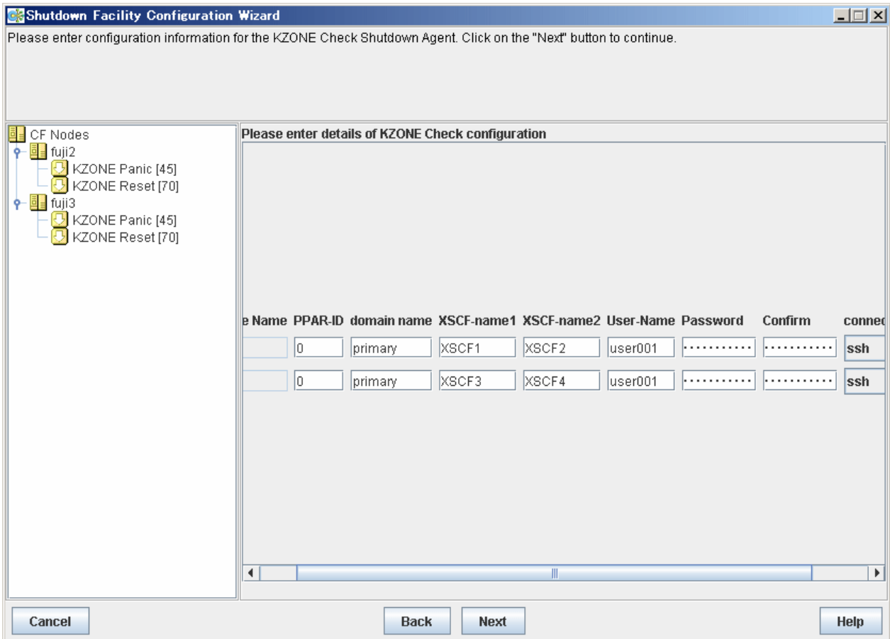
Figure 5.21 Configuring XSCF
