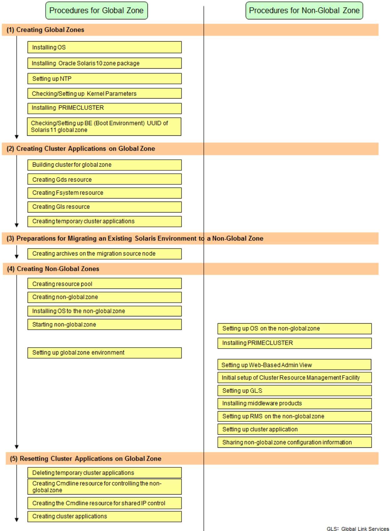
Figure 16.13 Flow for Building PRIMECLUSTER
