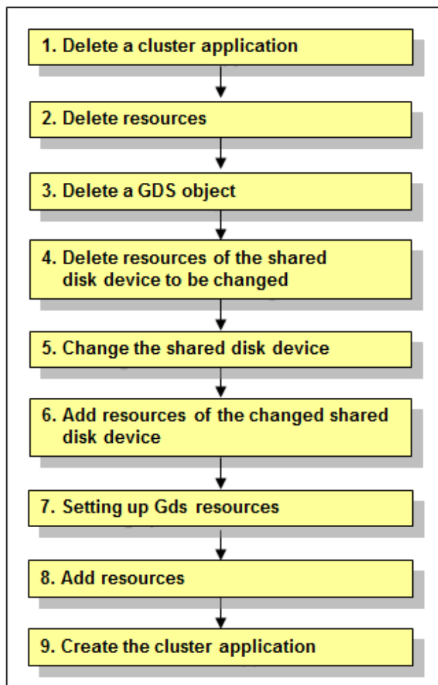
Figure 8.5 Procedure to change a shared disk device
