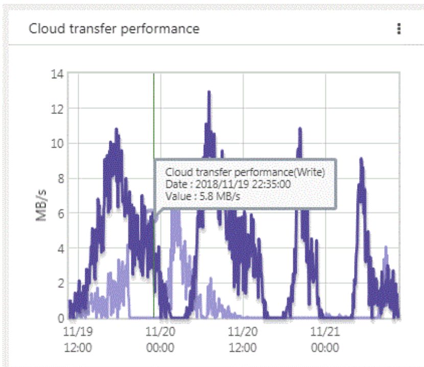
Figure 4.8 Example of Information Displayed on the Cloud Transfer Performance Panel
