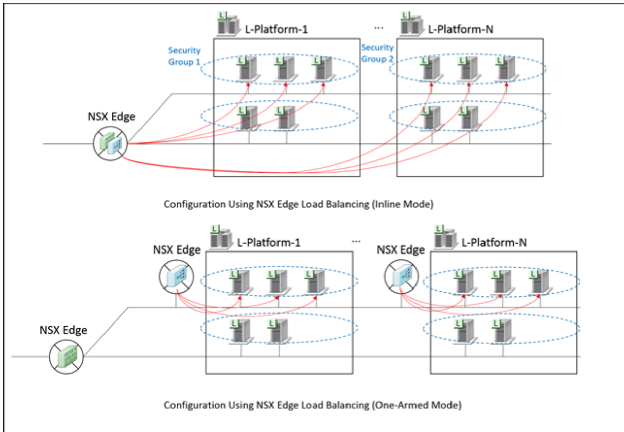
Figure 2.2 L-Platform Configuration
