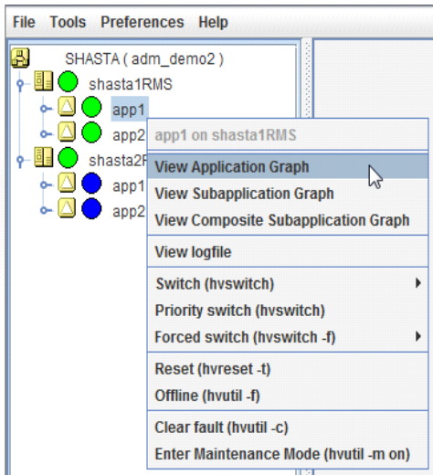
Figure 124: Viewing an RMS application graph
