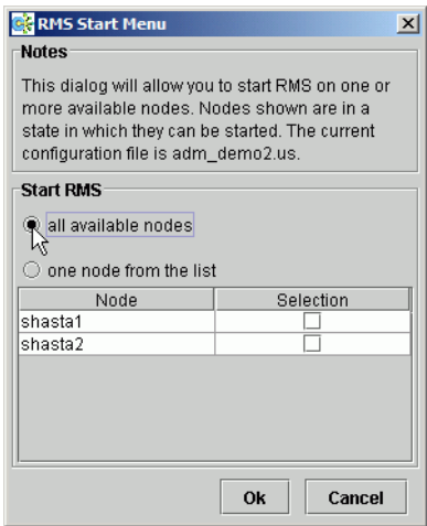
Figure 155: RMS Start Menu for all the nodes
