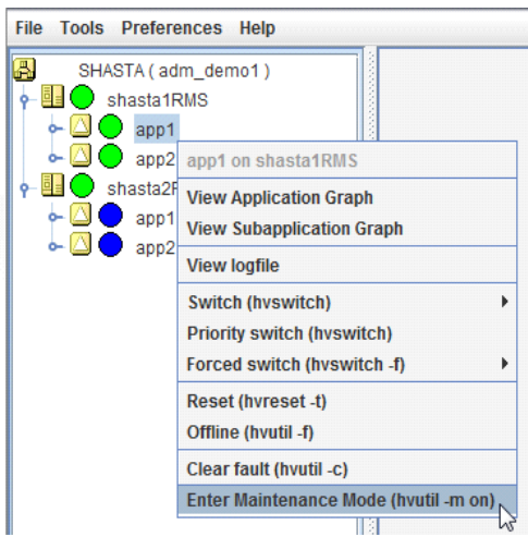
Figure 188: Starting maintenance mode for a single application
