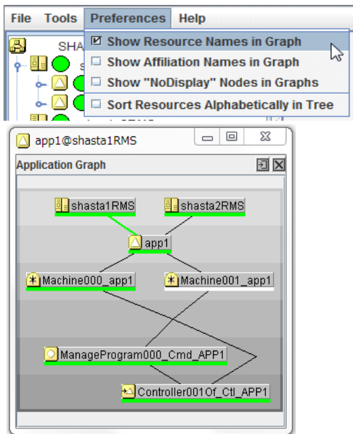
Figure 132: Displaying an RMS graph with affiliation names
