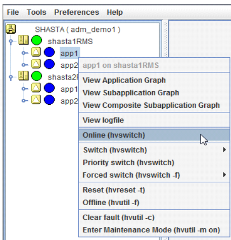
Figure 171: Starting an application
