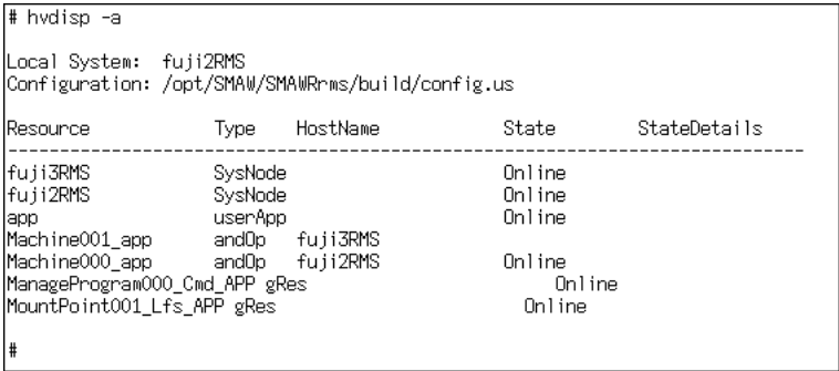
Figure 12: hvdisp output for initializing examples—RMS Wizard Tools
