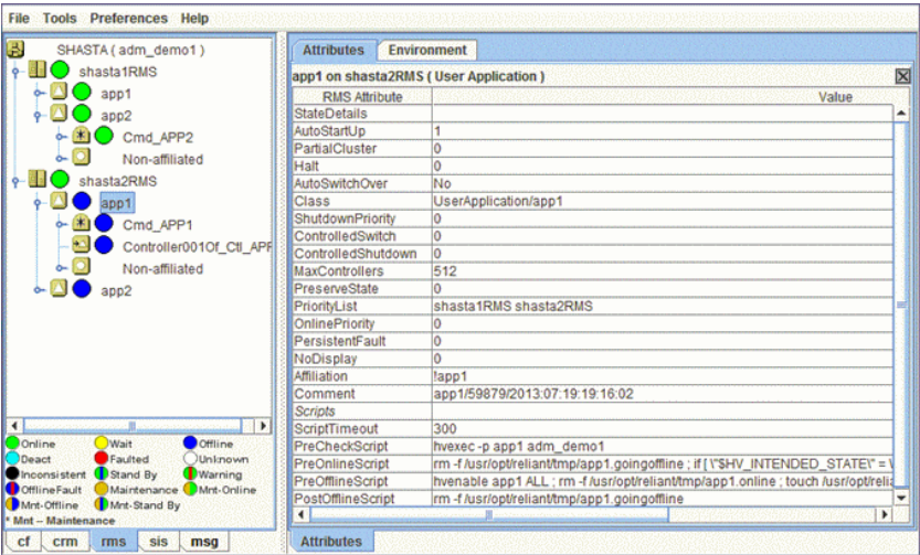
Figure 107: Displaying application and object states
