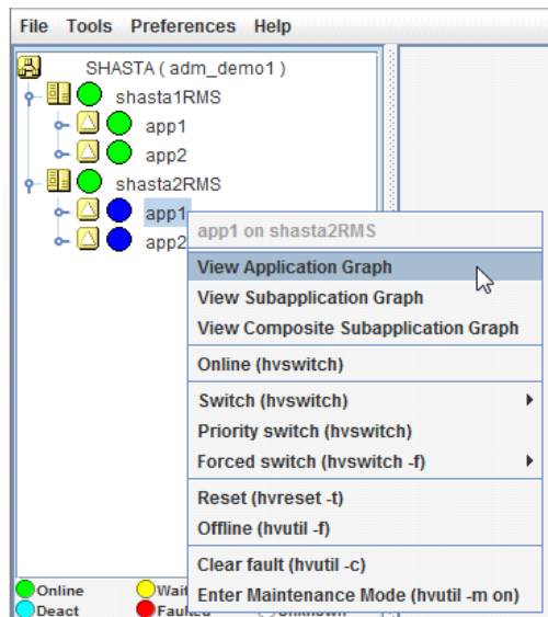
Figure 101: Pop-up context menu for an offline application
