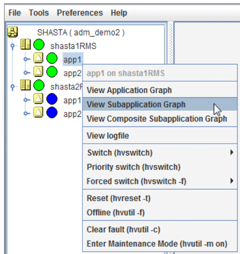
Figure 126: Viewing an RMS subapplication graph
