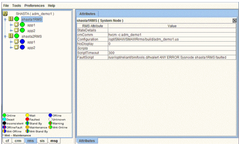
Figure 97: Main Cluster Admin window—RMS view
