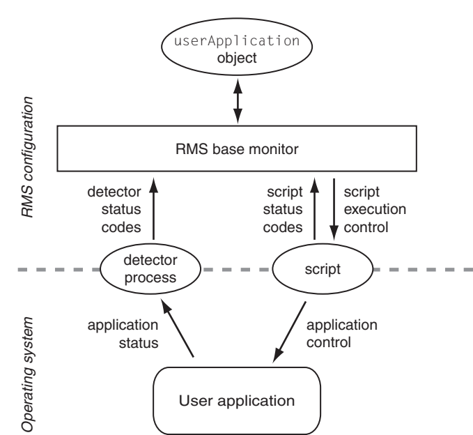
Figure 2: Interface between RMS and the operating system
