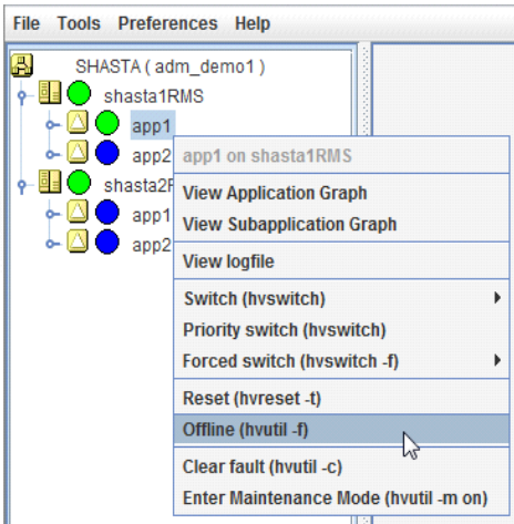
Figure 172: Shutting down an application
