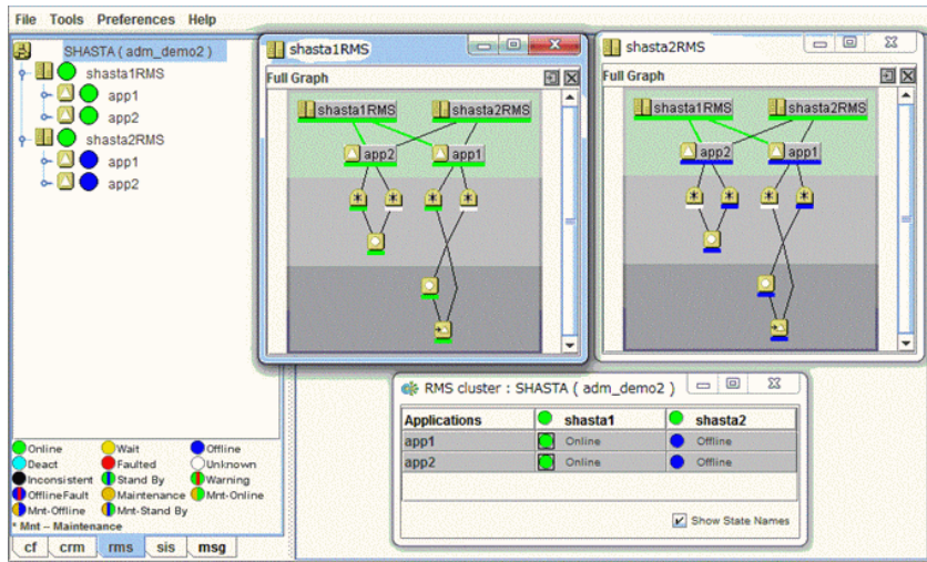
Figure 137: Cluster state before RMS is shut down
