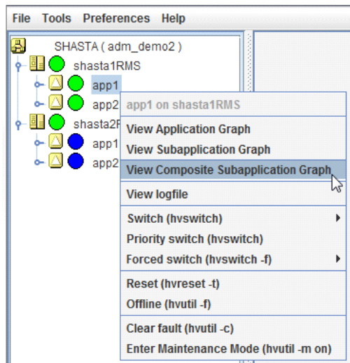
Figure 129: Viewing an RMS composite subapplication graph
