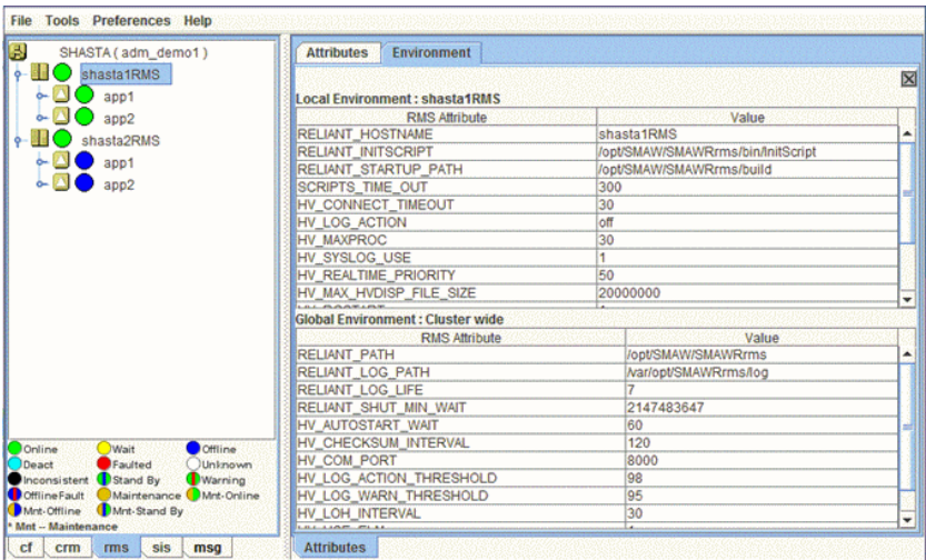
Figure 106: Local environment variables view
