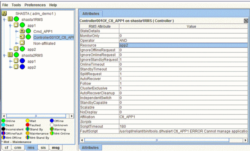
Figure 98: RMS tree with a controller object
