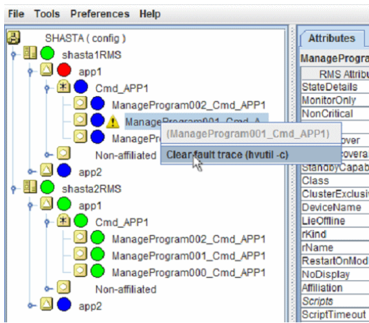
Figure 185: Clearing the Fault trace
