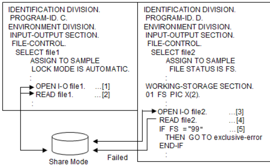
Figure 6.9 Record Locking
