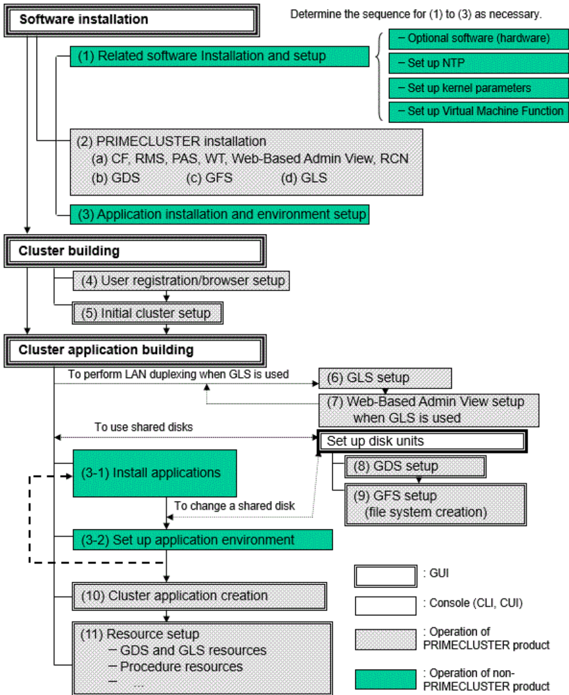
Figure 1.2 Flow of PRIMECLUSTER system installation
