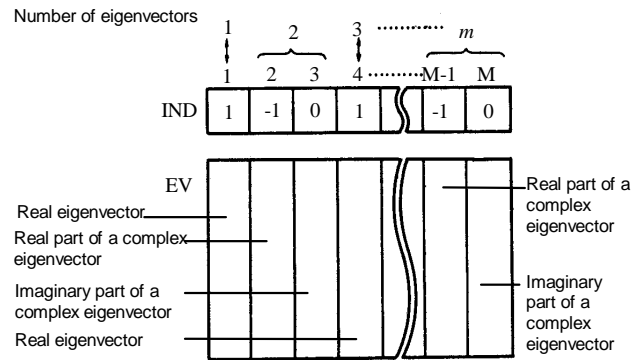
Fig. NRML-1 Relationship between IND and EV
