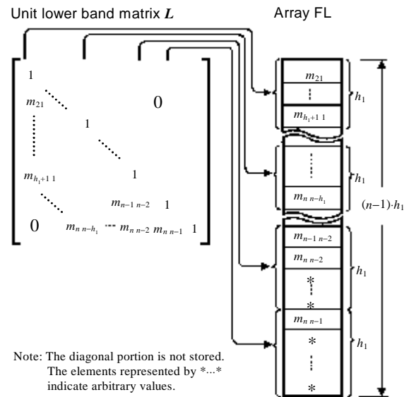
Fig. LBX1R-1 Storing method for each element of L into array FL.
