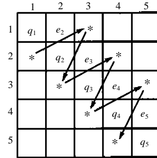
Fig. ASVD1-3 Behavior of non-zero elements(n=5)
