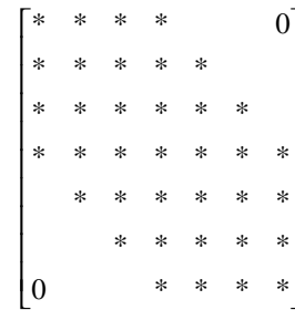
Fig. BSC1-4 Coefficient matrix (for m=3 and n_i=5 )
