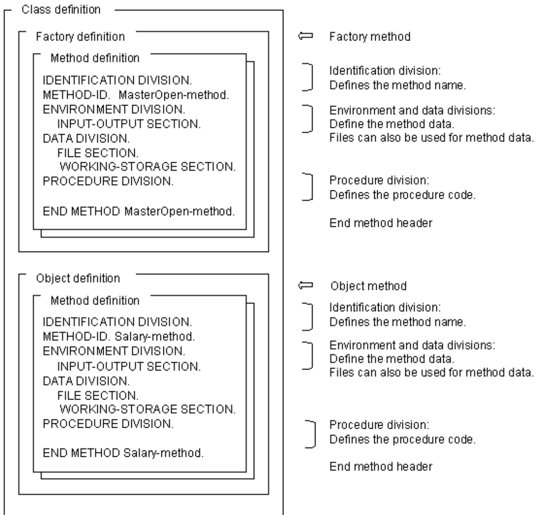
Figure 14.8 Method definitions
