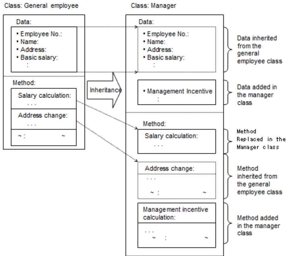
Figure 13.3 Inheritance example
