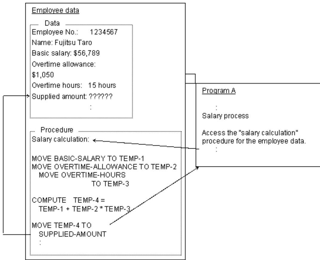
Figure 13.2 Data Hiding
