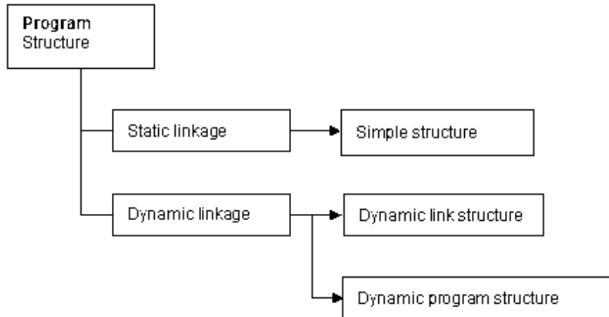
Figure 4.1 Program Structure
