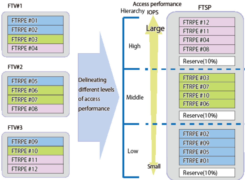
Figure 3.3 FTRPE Moving in Boundary of Each Sub-Pool
