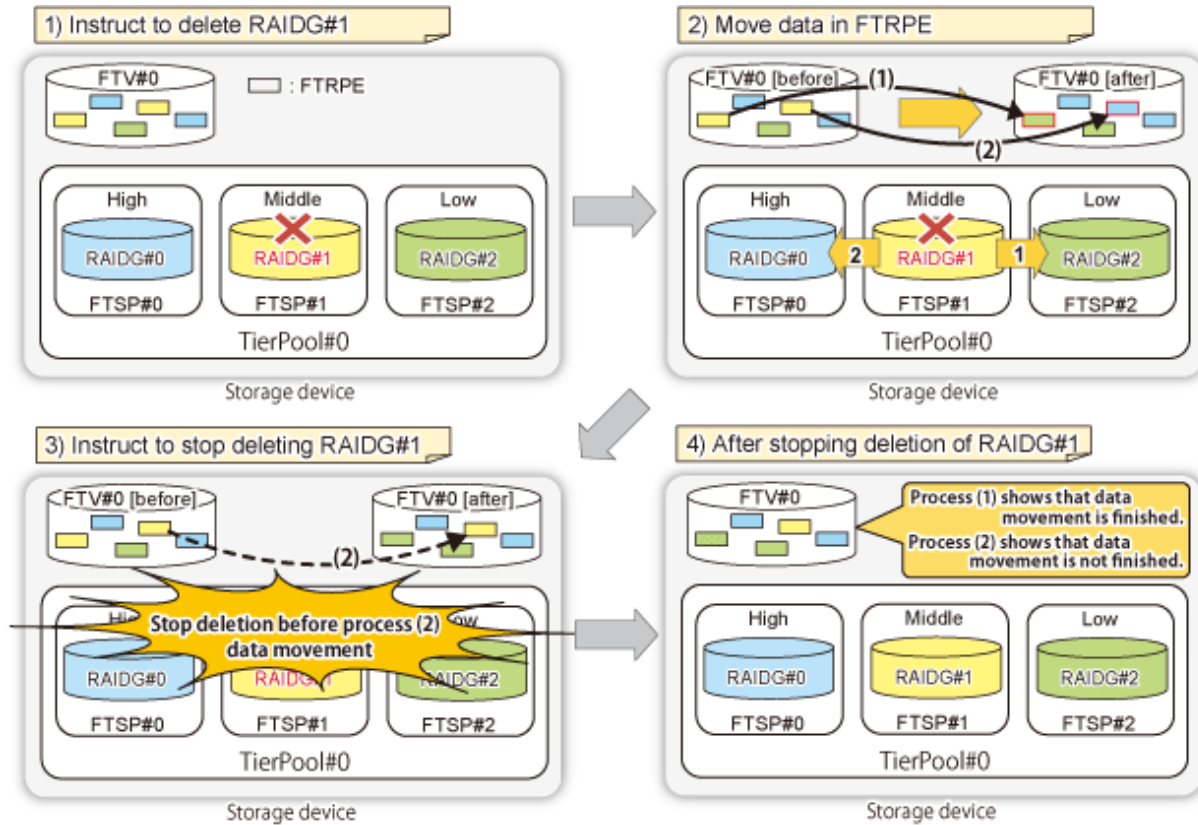
Figure 4.2 Operation Example of When a RAID Group Deletion Process Is Stopped
