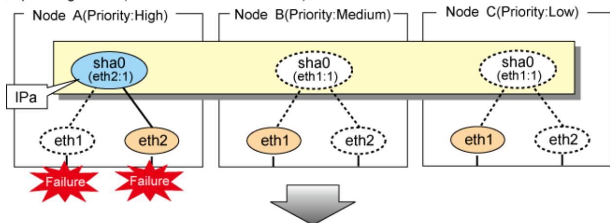
Figure 5.34 Switching operation of NIC switching mode (logical IP takeover) [Operating Status(Failure occurred in node A)]
