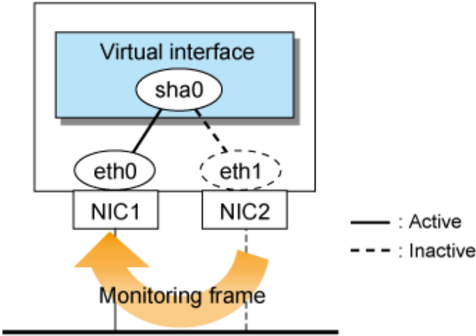
Figure 2.39 Automatic fail-back function Initial status
