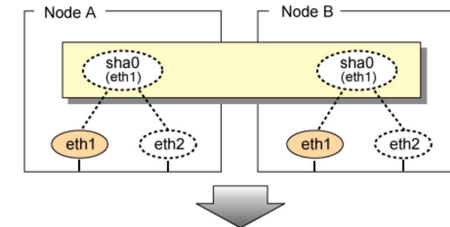
Figure 5.8 Startup behavior of NIC switching mode (takeover physical IP address I) [Before an userApplication starts up]
