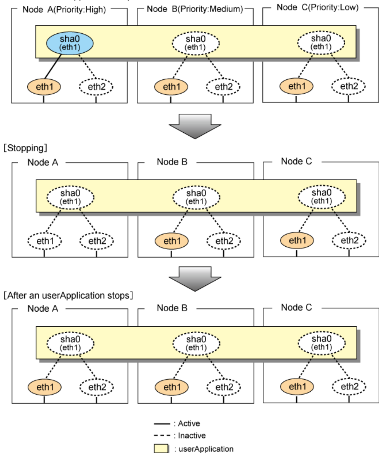
Figure 5.39 Stopping operation of NIC switching mode (physical IP takeover I) [Before an userApplication stops]
