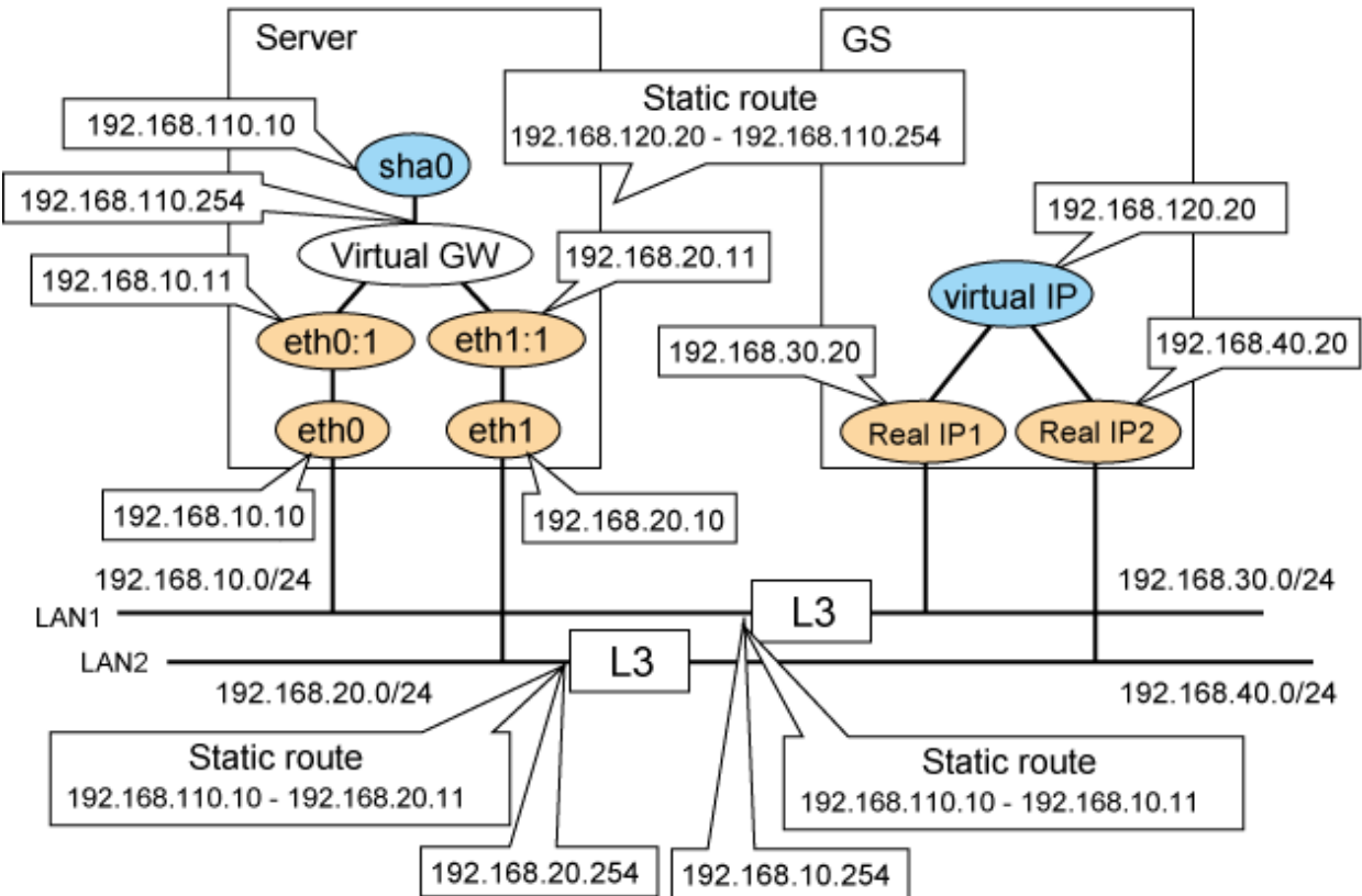
Figure H.2 Remote configuration
