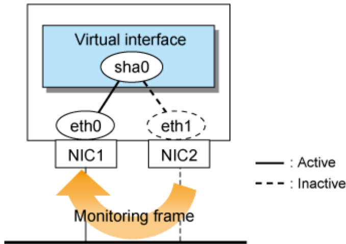
Figure 2.41 Automatic fail-back function
