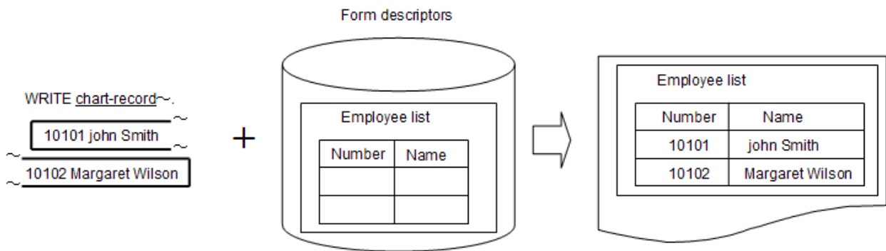
Figure 7.7 Flow of control with form descriptors
