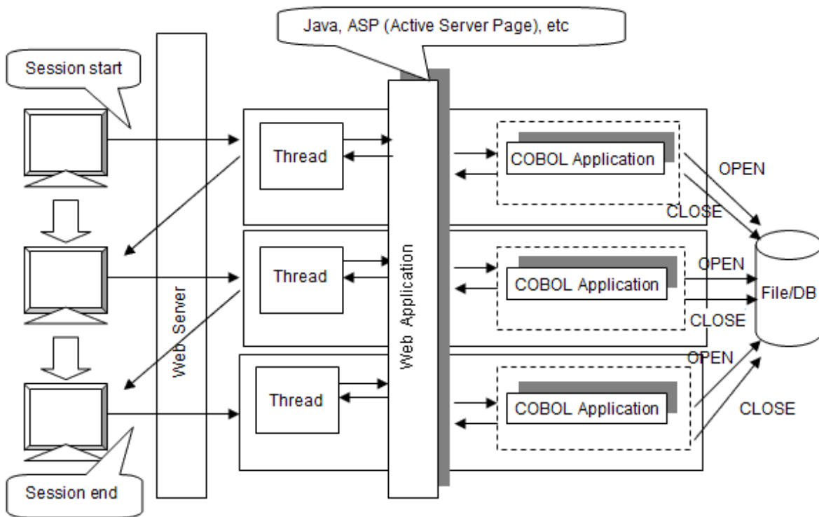
Figure 19.3 When run unit data is not relayed
