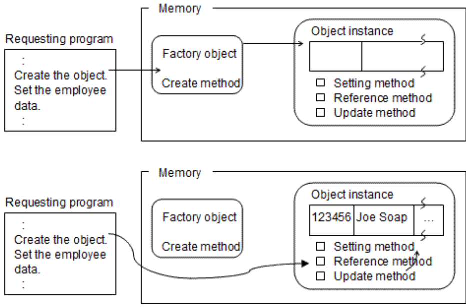
Figure 14.7 Creating an object and populating the data
