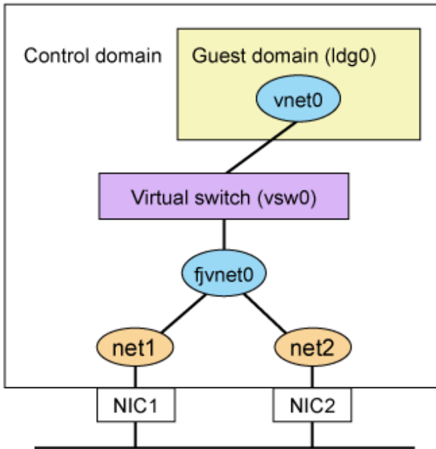
Figure 3.3 Example of configuration in the Oracle VM environment
