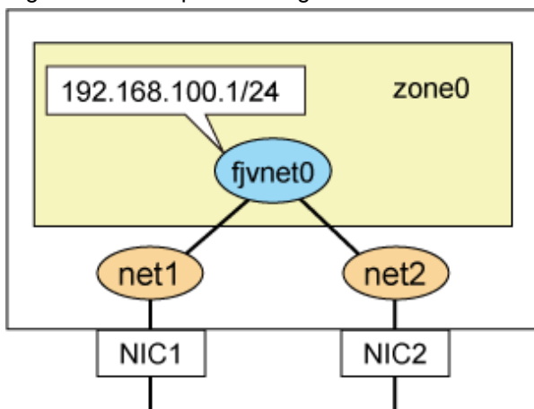
Figure 3.2 Example of configuration in the Solaris Zones environment
