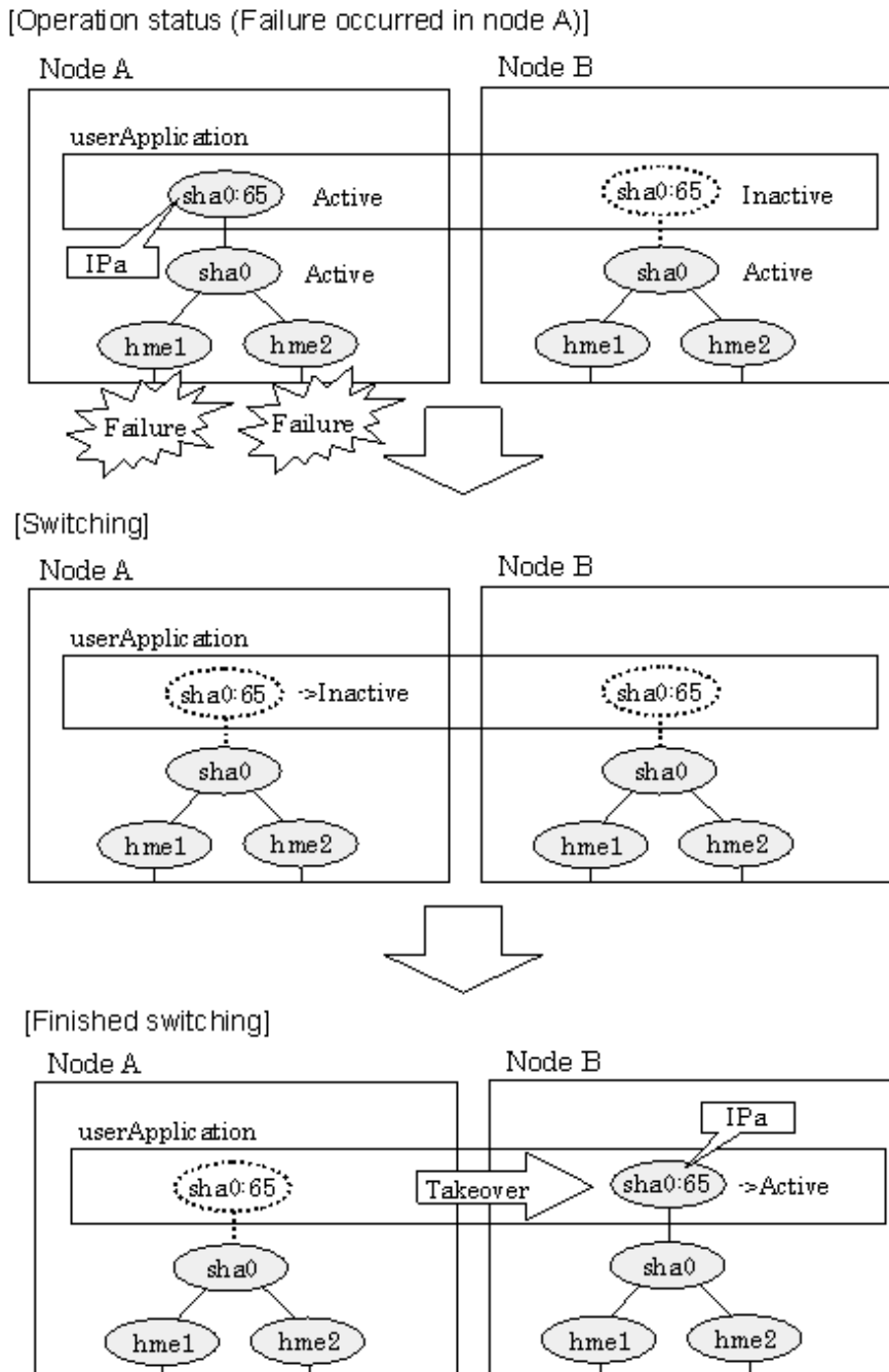
Figure 5.7 Switching behavior of Fast switching mode
