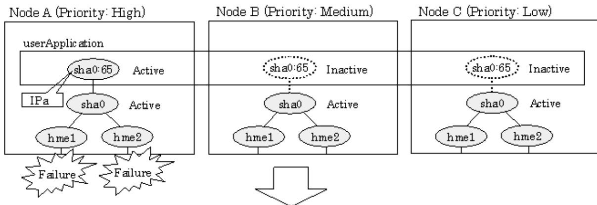
Figure 5.25 Switching operation of Fast switching mode
