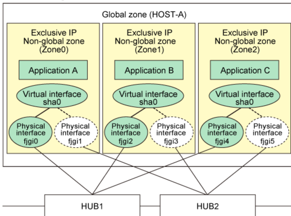
Figure C.2 Network interface configuration example of Solaris Zones in the exclusive-IP zone
