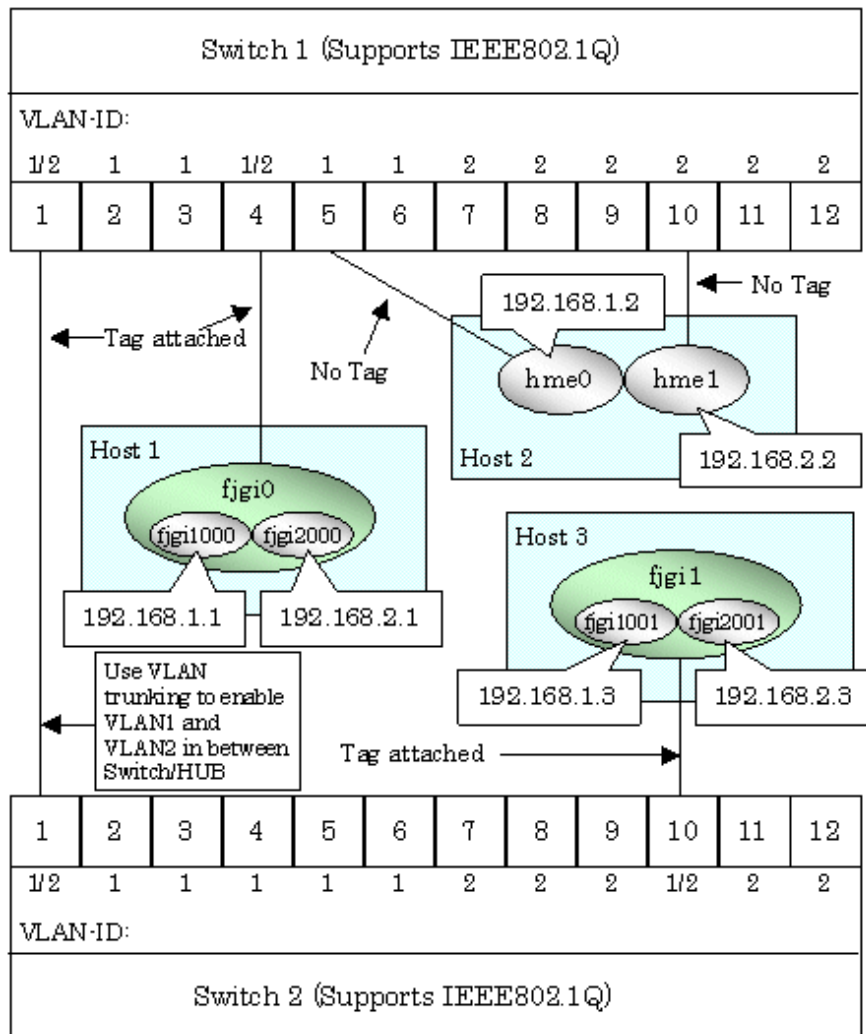
Figure 2.43 Network structure using Tagged VLAN
