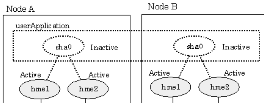
Figure 5.6 Startup behavior of GS/SURE linkage mode
