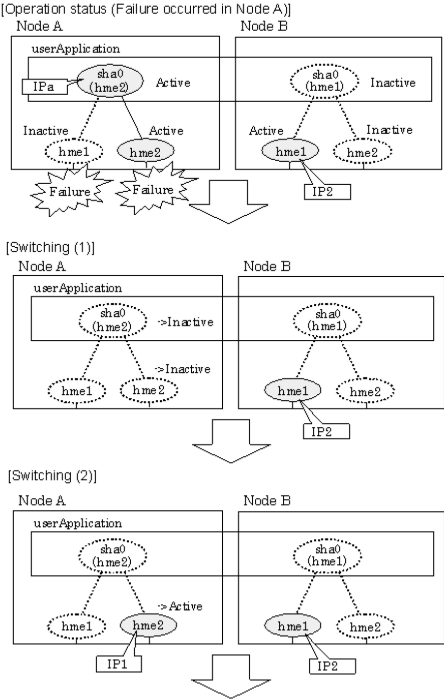
Figure 5.9 Switching behavior of NIC switching mode (takeover physical IP 1) (continues)
