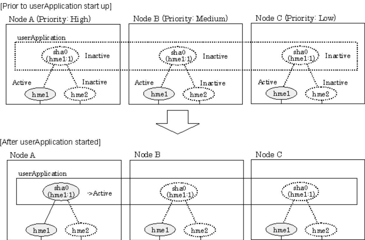
Figure 5.22 Start-up behavior of NIC switching mode (logical IP takeover)
