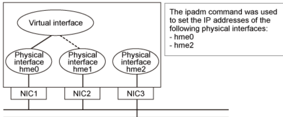
Figure 3.3 Setup example of the OS setting file in the NIC switching mode (For Solaris 11)
