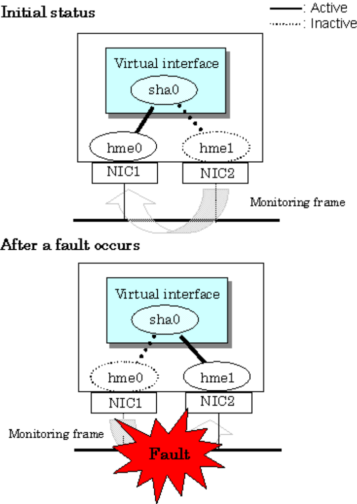
Figure 2.31 Automatic fail-back function (continued)
