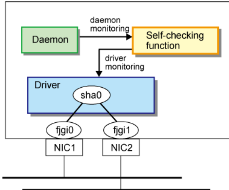
Figure 2.46 Self-checking function
