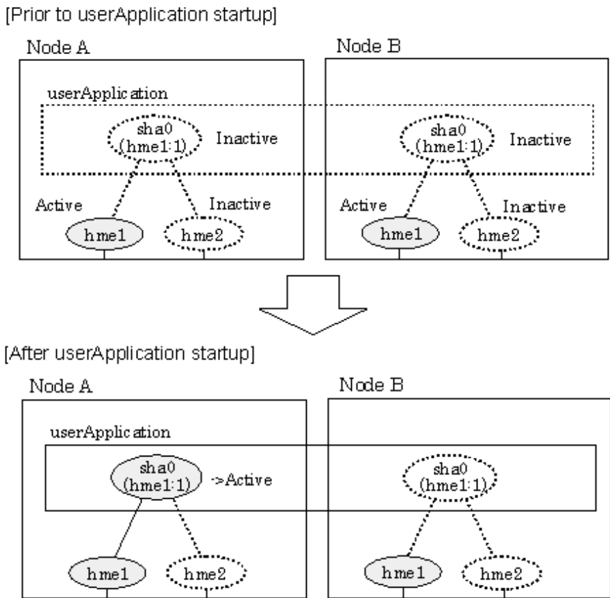
Figure 5.3 Startup behavior of NIC switching mode (take over logical IP)
