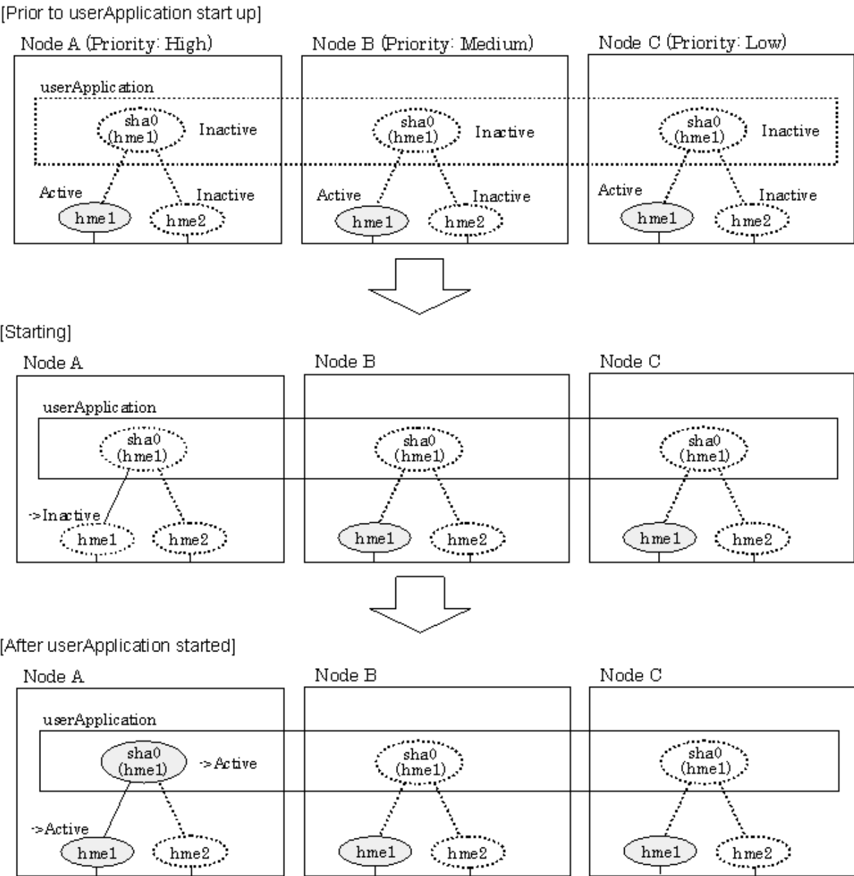
Figure 5.23 Start-up behavior of NIC switching mode (physical IP takeover)
