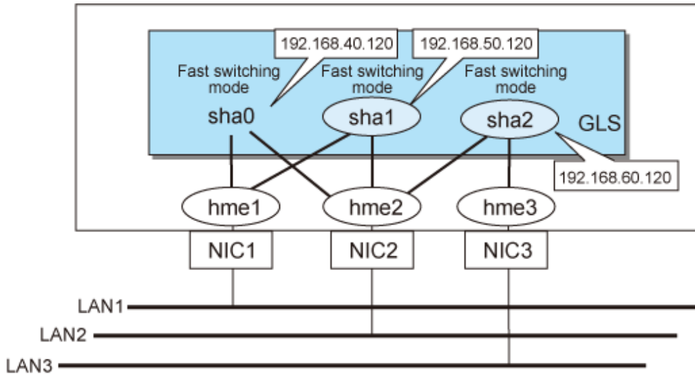
Figure 2.20 Example of sharing physical interface (1)
