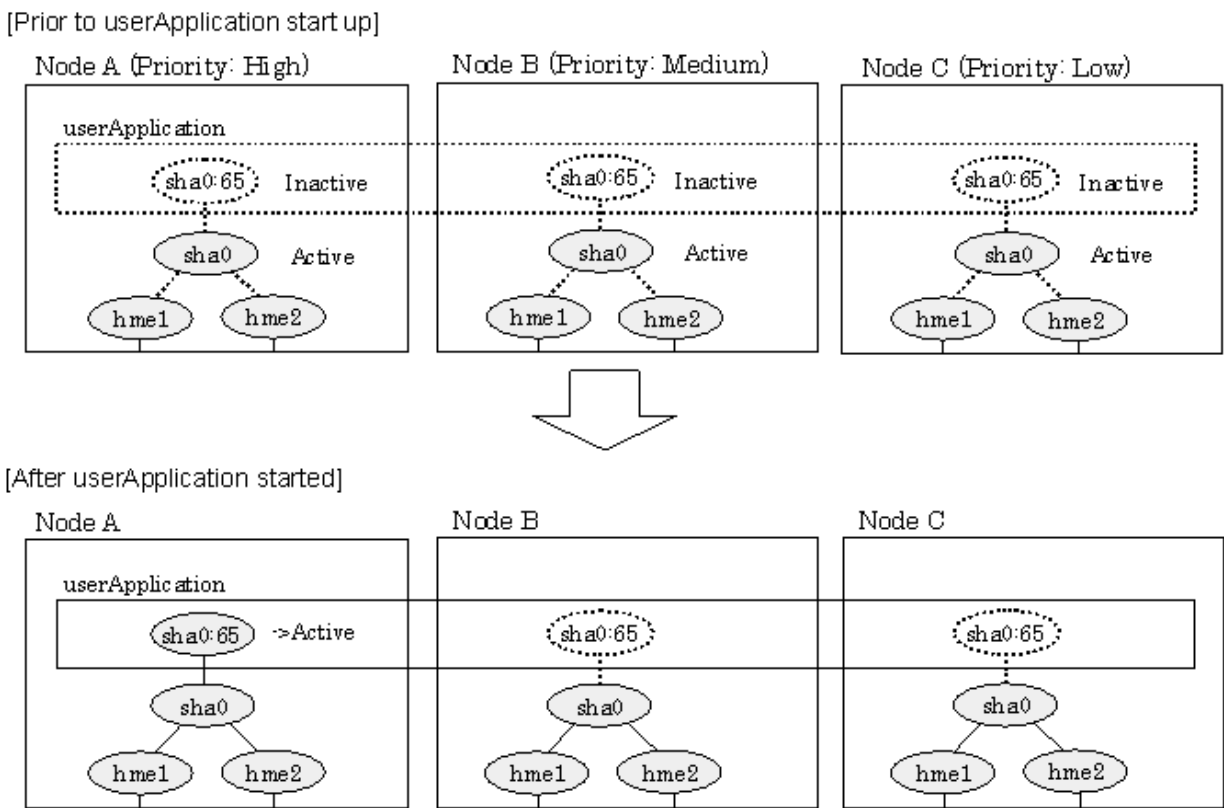
Figure 5.21 Start-up behavior of Fast switching mode
