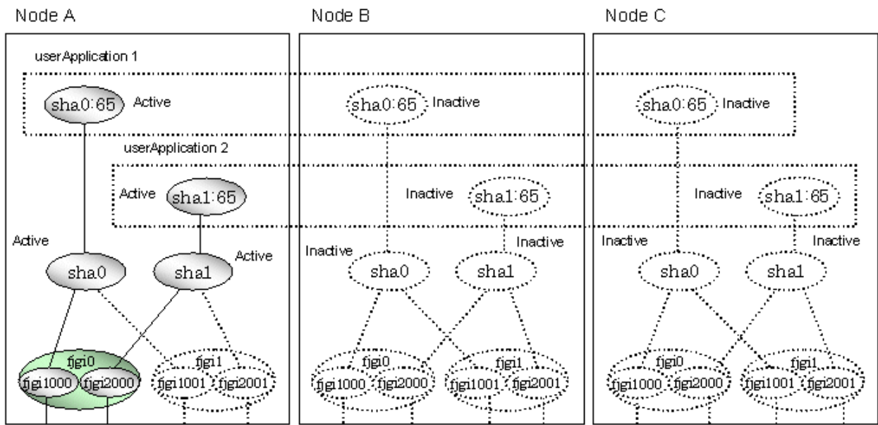
Figure 5.39 Tagged VLAN interface multiplexing on NIC switching mode (Cascade)
