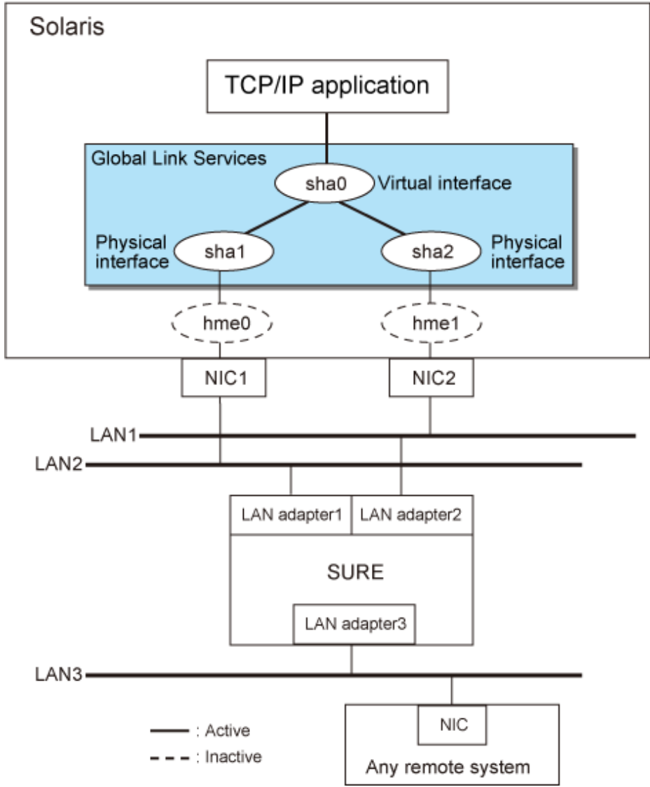
Figure 1.9 GS/SURE linkage mode (TCP relay function)
