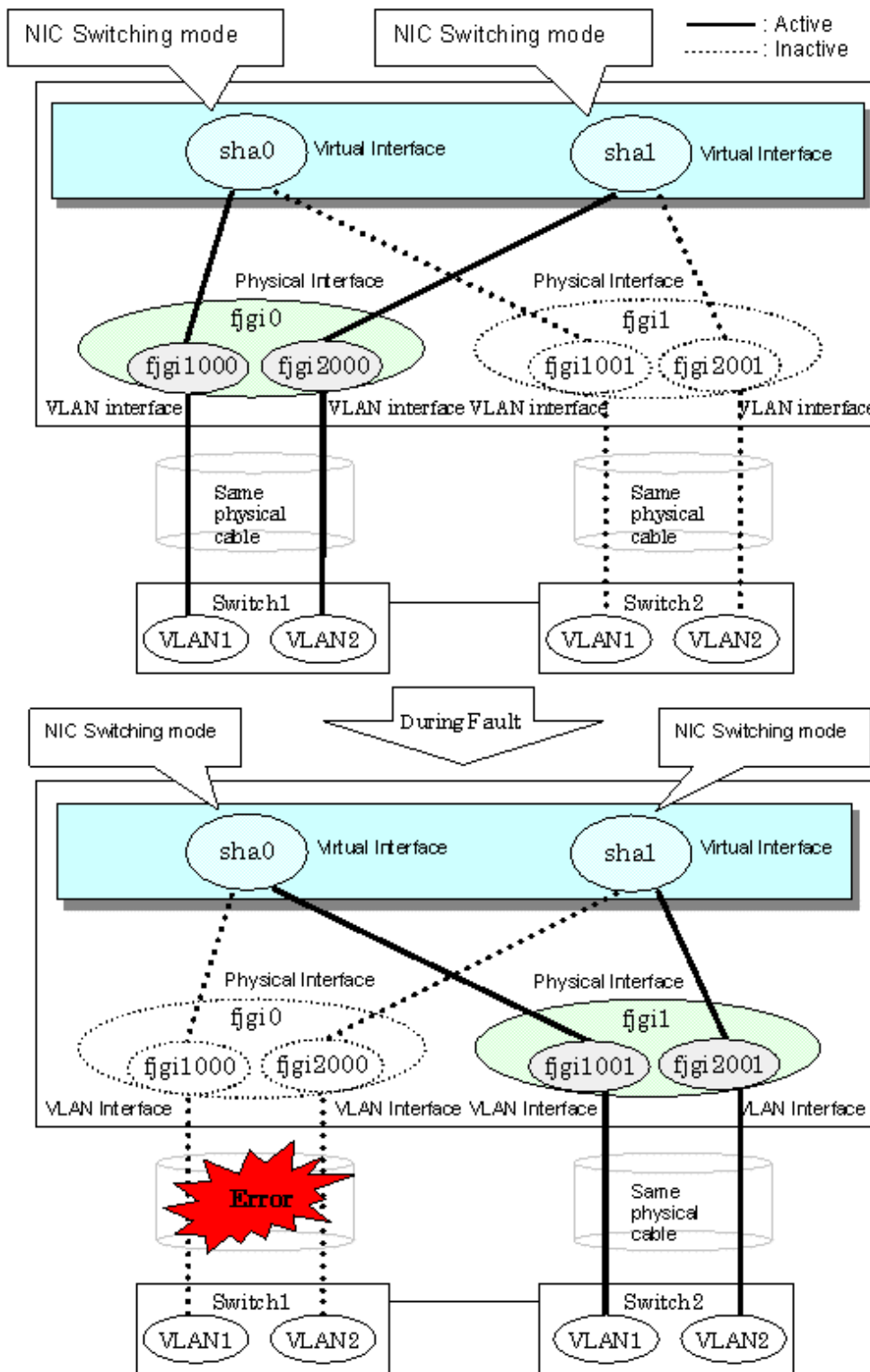
Figure 2.43 Using Tagged VLAN Interface architecture
