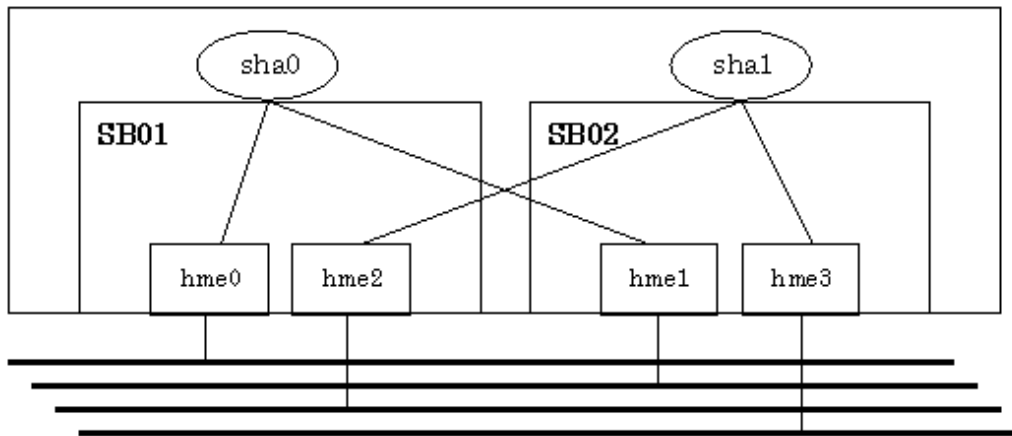
Figure 3.15 Recommended LAN configuration
