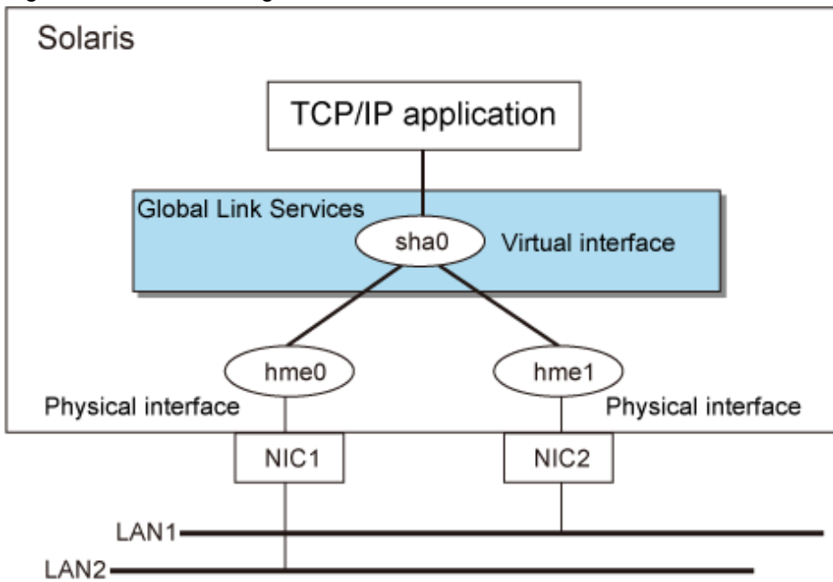
Figure 1.6 Fast switching
