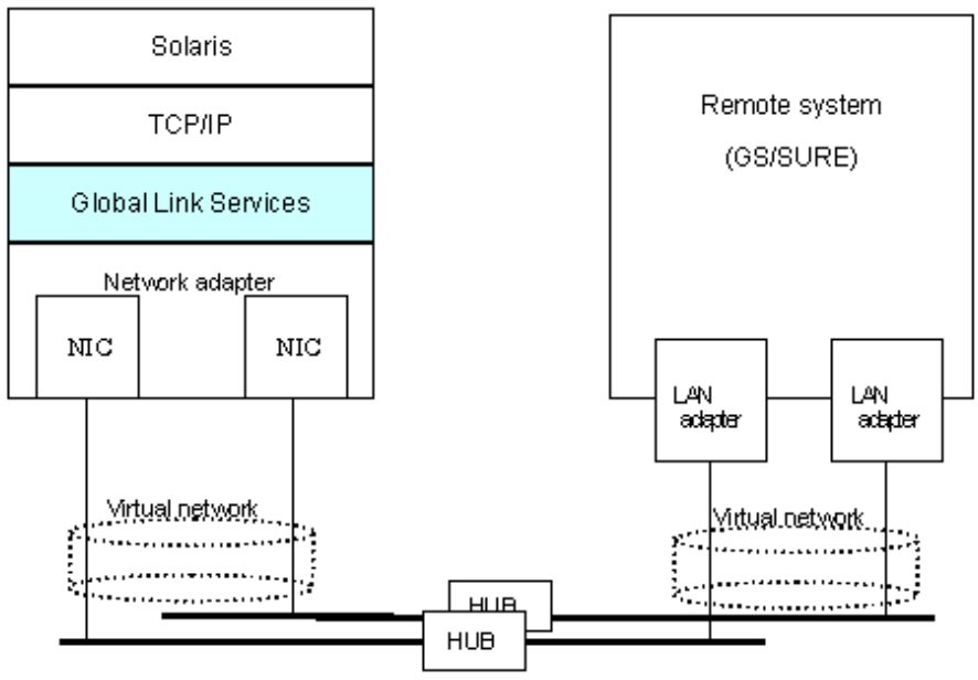
Figure 1.3 GS/SURE linkage mode (GS/SURE connection function)
