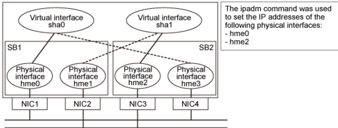
Figure F.4 Configuration of NIC switching mode after change (For Solaris 11)
