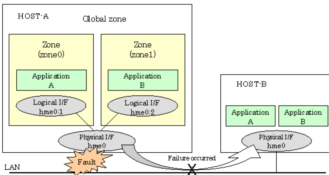
Figure C.3 Interface structure without redundant line control
