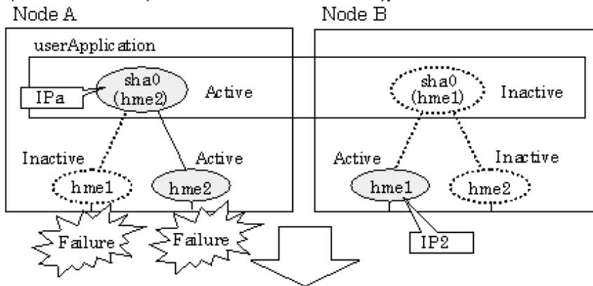
Figure 5.9 Switching behavior of NIC switching mode (takeover physical IP I) (continues)
