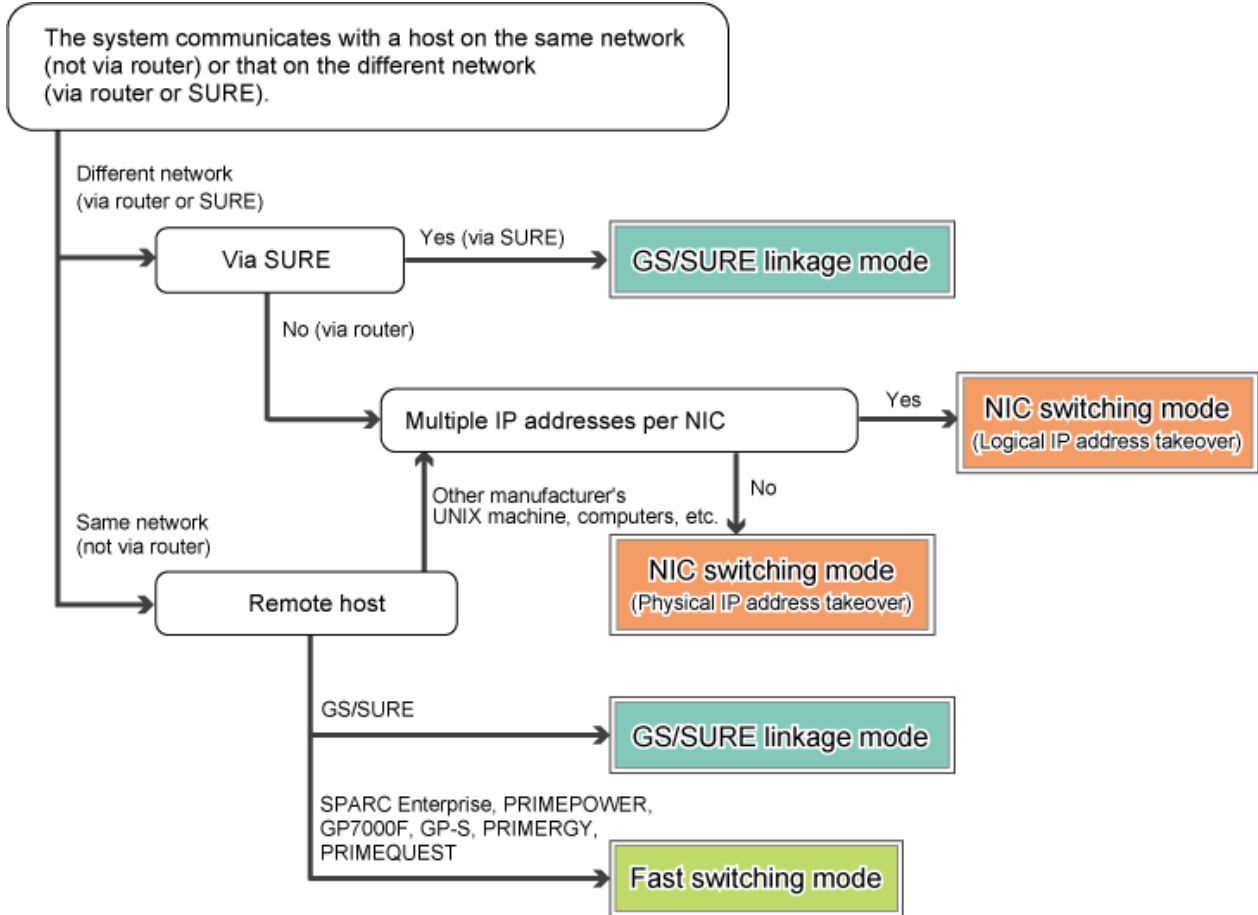
Figure 1.5 Redundant line control method decision flow chart
