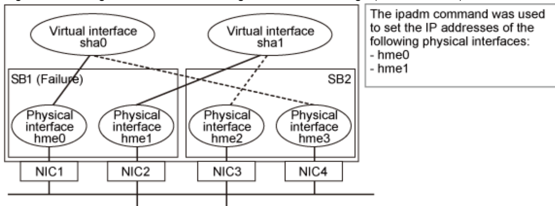
Figure F.2 Configuration of NIC switching mode before change (For Solaris 11)
