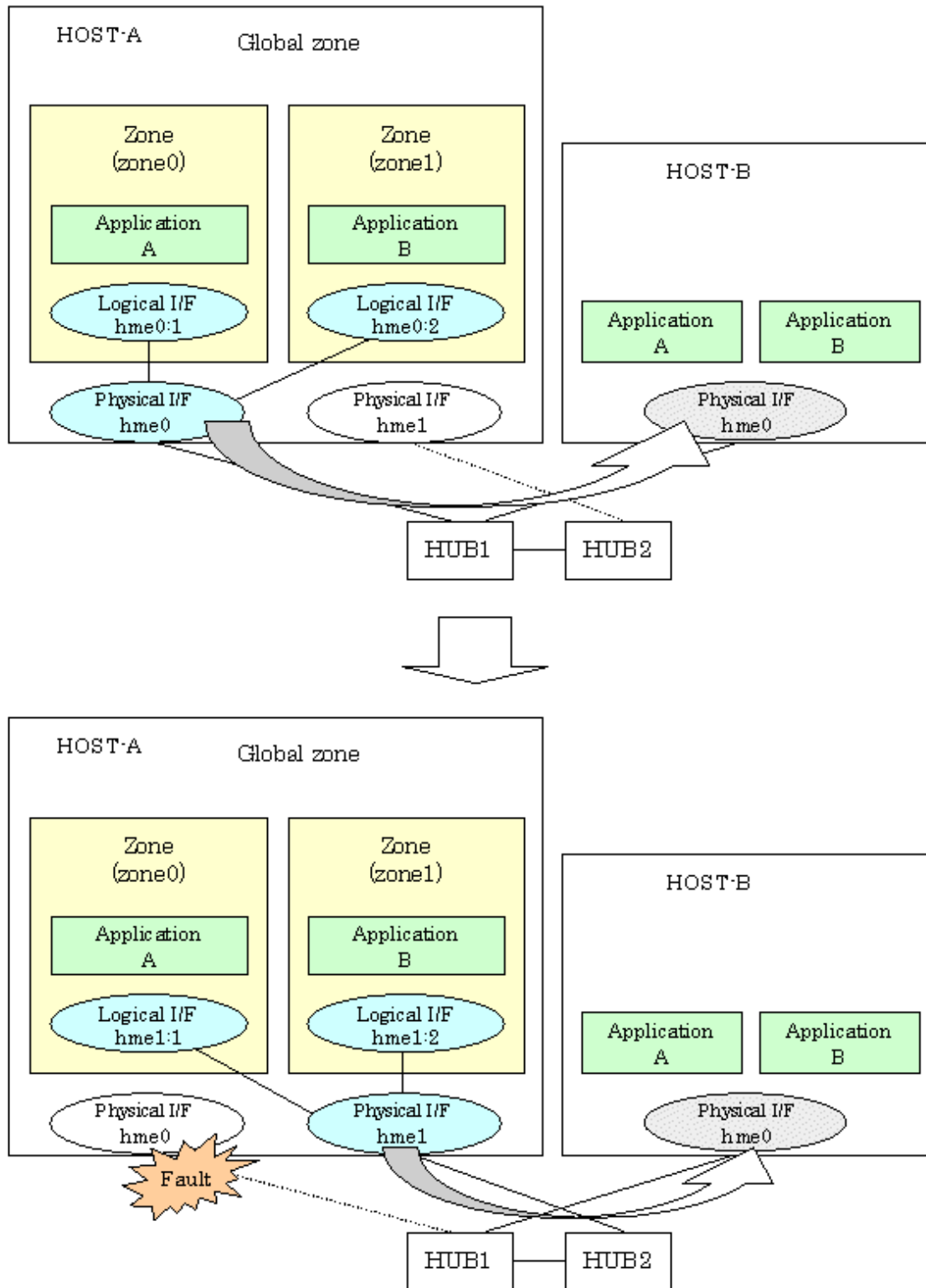
Figure C.5 Network reliability in NIC switching mode
