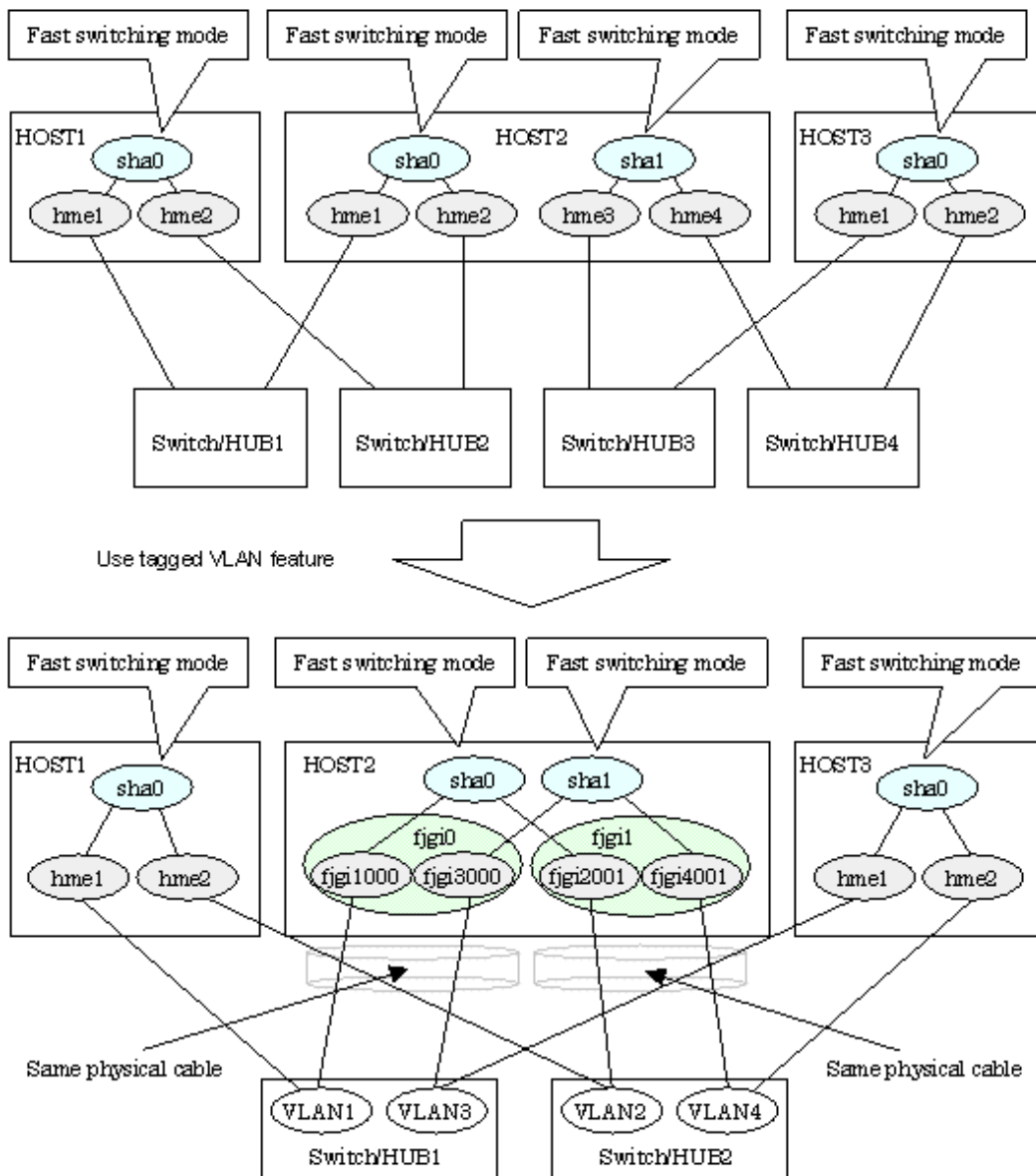
Figure 2.44 When Switch/HUB and NIC come short.
