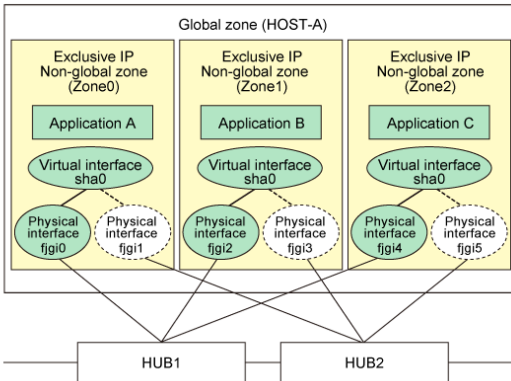
Figure C.2 Network interface configuration example of Solaris containers in the exclusive-IP zone
