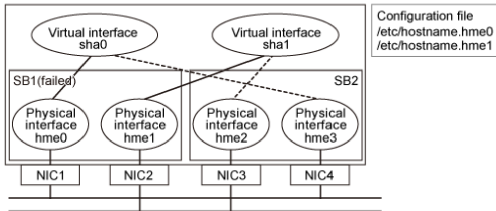
Figure F.1 Configuration of NIC switching mode before change (For Solaris 10)
