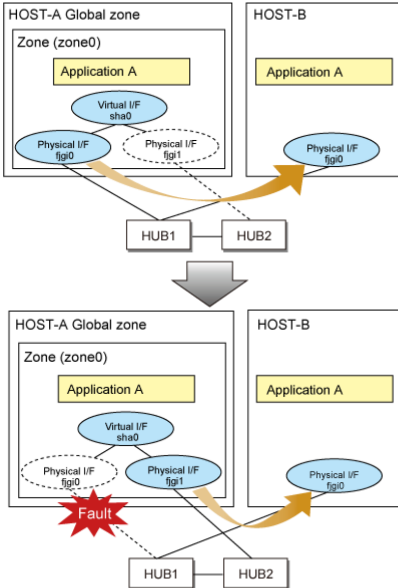
Figure C.6 For using NIC switching mode
