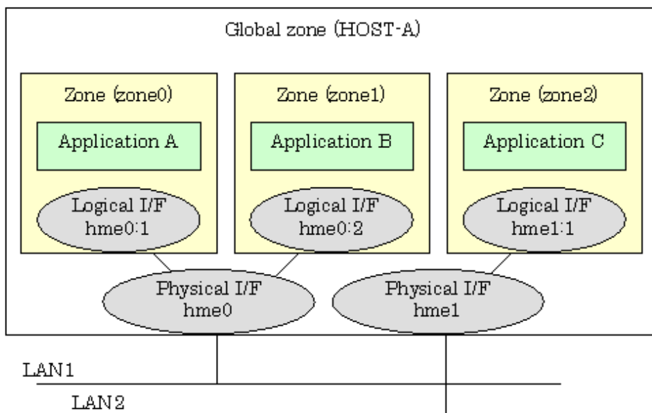
Figure C.1 Network interface configuration example of Solaris containers in the shared IP configuration
