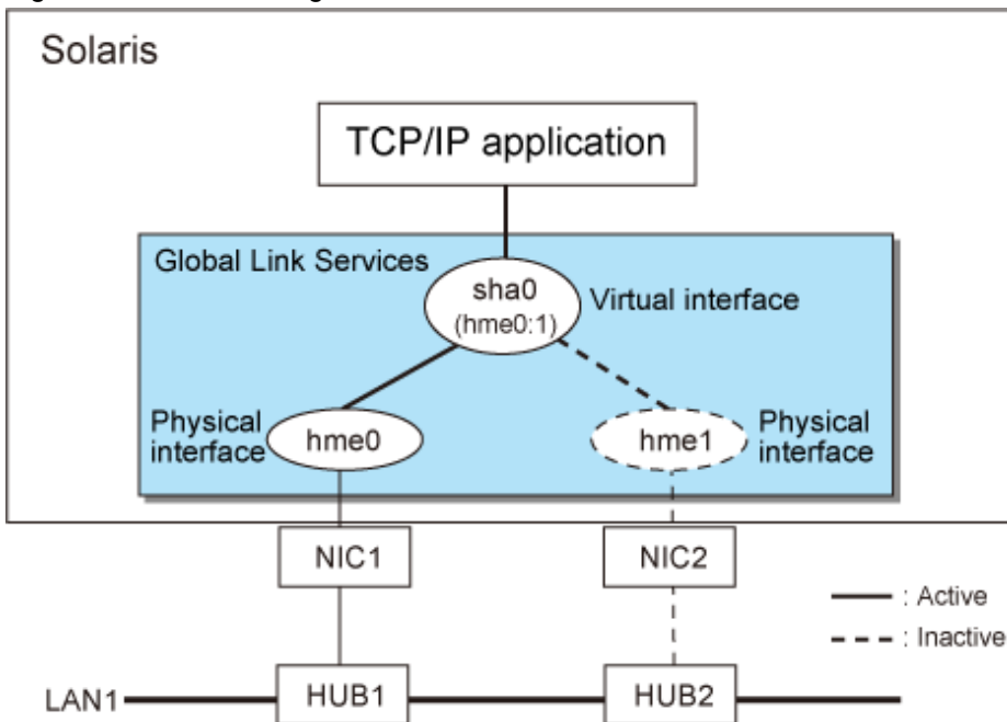
Figure 1.7 NIC switching mode
