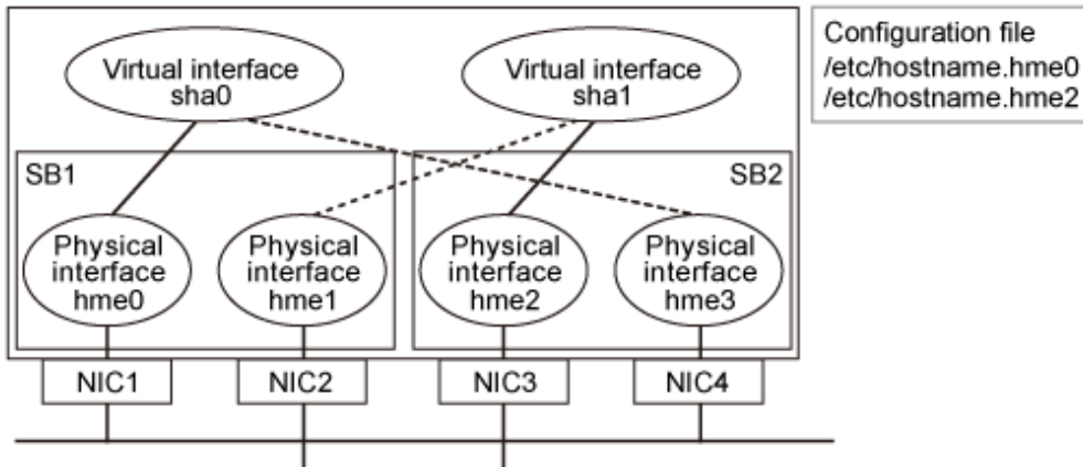
Figure F.3 Configuration of NIC switching mode after change (For Solaris 10)
