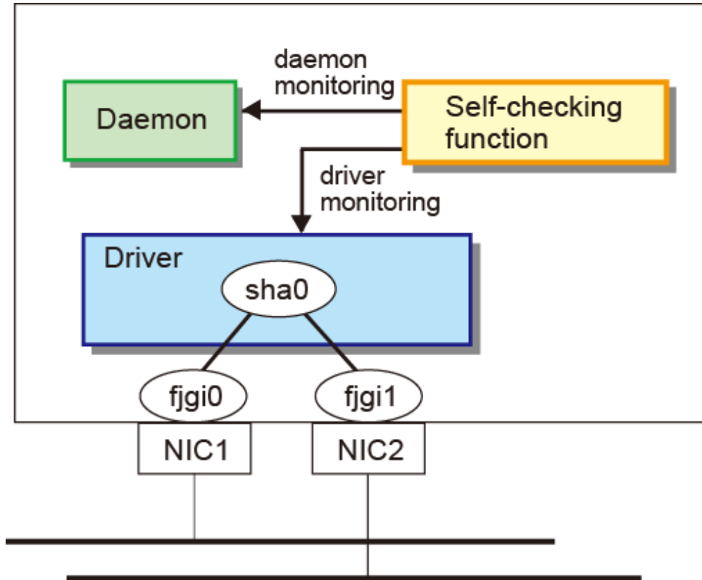
Figure 2.45 Self-checking function
