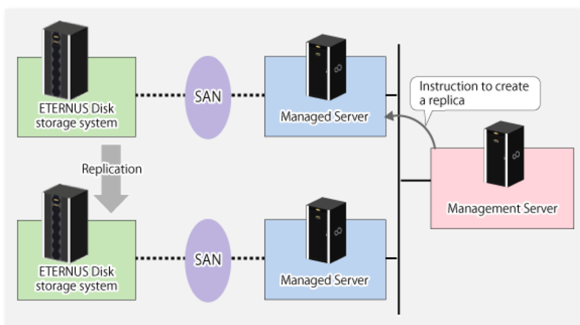
Figure 7.9 Configuration of Servers That Perform Replication
