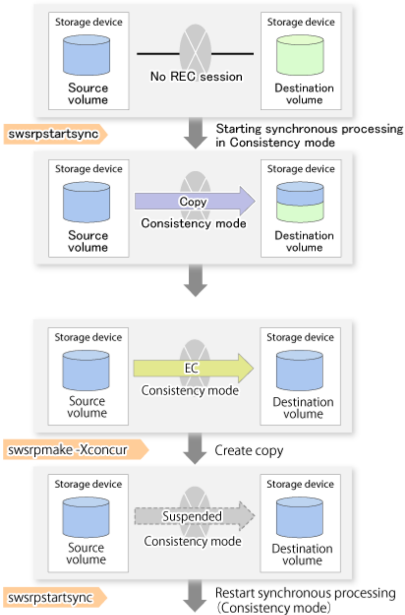
Figure 7.43 When Consistency Mode Used
