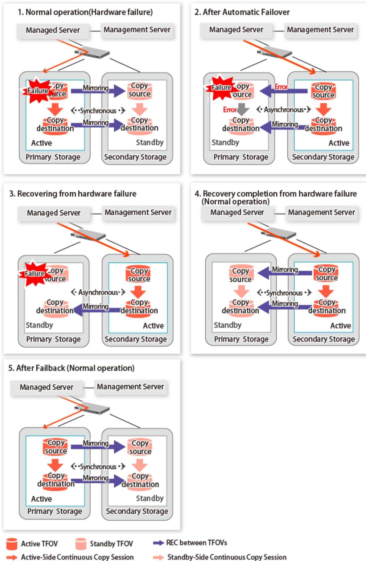
Figure 8.8 When Automatic Failover Is Performed Due to Hardware Failure Occuring on Primary Storage Where TFO Status Is "Active"
