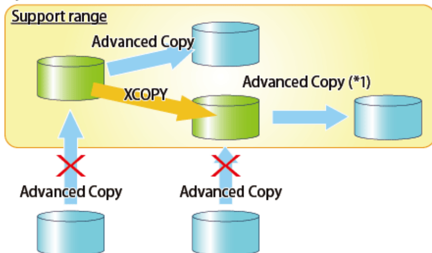
Figure 11.6 Use in Combination with XCOPY
