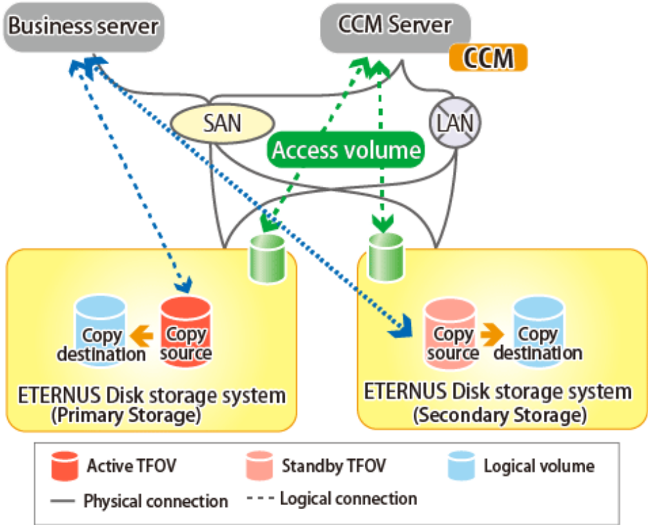
Figure 3.16 System Configuration for Performing Intra-box Copy (OPC/QuickOPC/SnapOPC+/EC)
