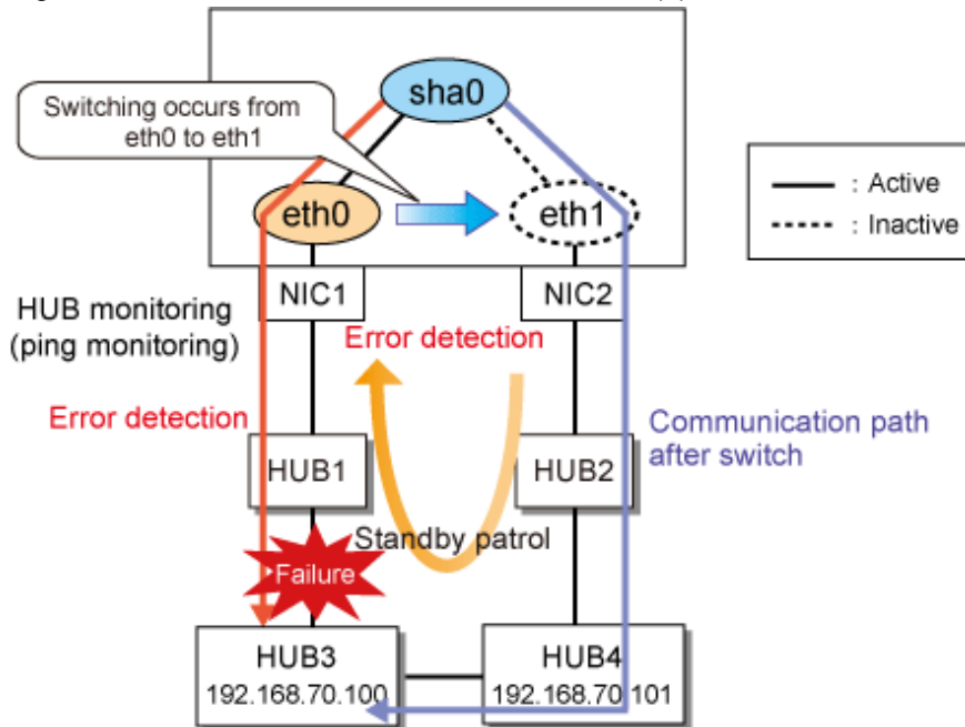
Figure G.3 When the communication is switched (2)
