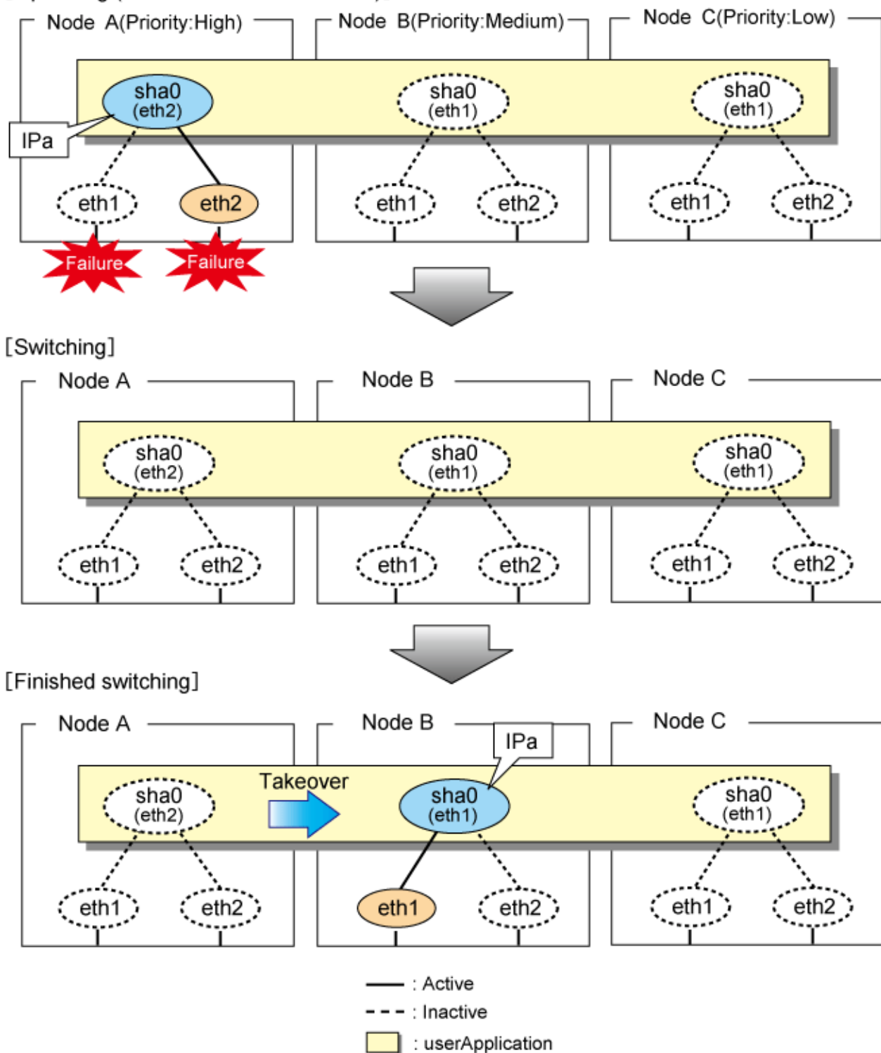
Figure 5.37 Switching operation of NIC switching mode (physical IP takeover II) [Operating (Failure occurred in node A)]
