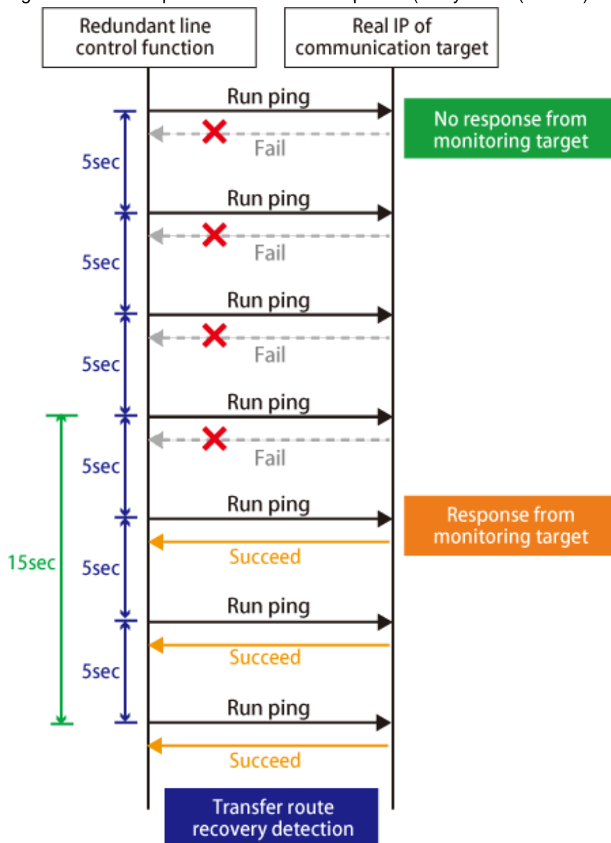
Figure I.1 Transfer path error detection sequence (Retry count (2 times))
