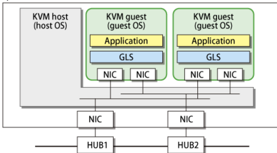
Figure C.2 Configuration 2: Configuration diagram for creating a highly reliable network on KVM guests in a single system
