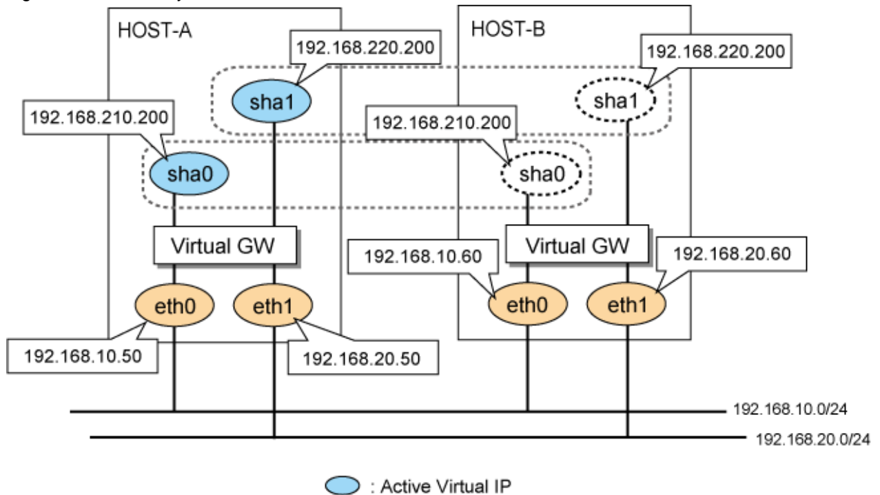
Figure 3.22 Cluster system
