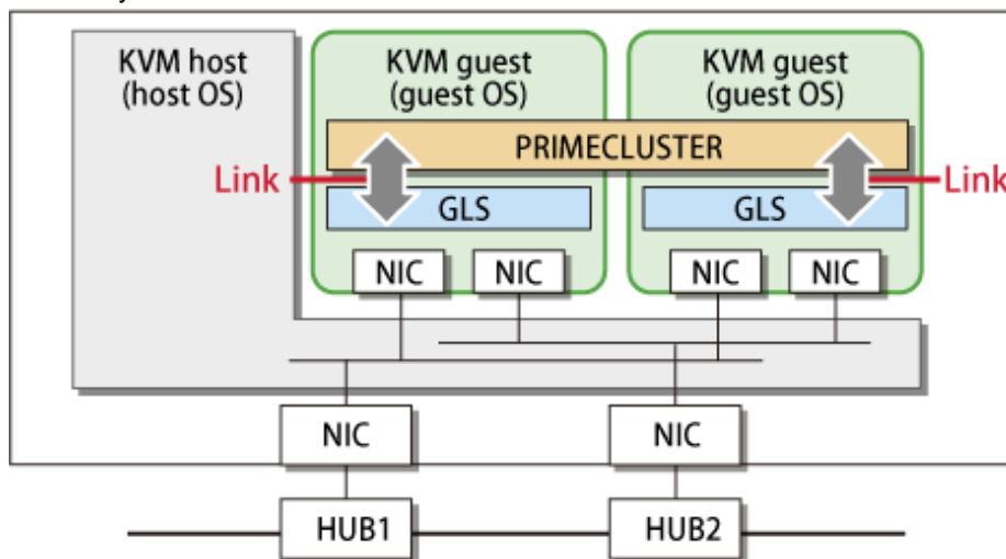
Figure C.3 Configuration 3: Configuration diagram for creating a highly reliable network on each KVM guest in a cluster system
