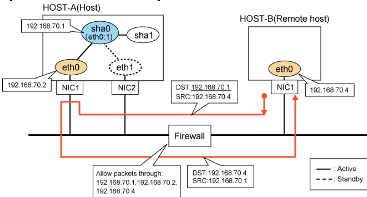
Figure G.4 The remote host is the transmitting side.
