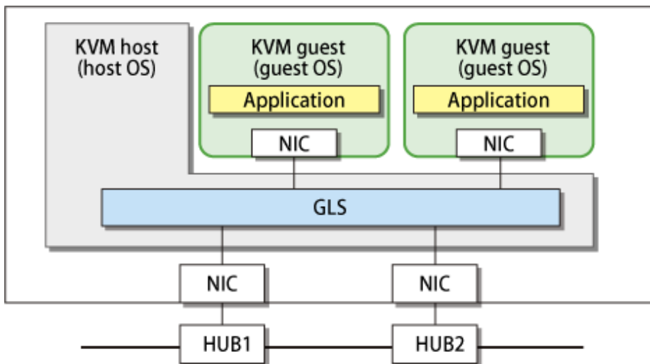
Figure C.1 Configuration 1: Configuration diagram for creating a highly reliable network of KVM guests on the KVM host
