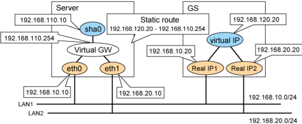
Figure H.1 Adjacent configuration
