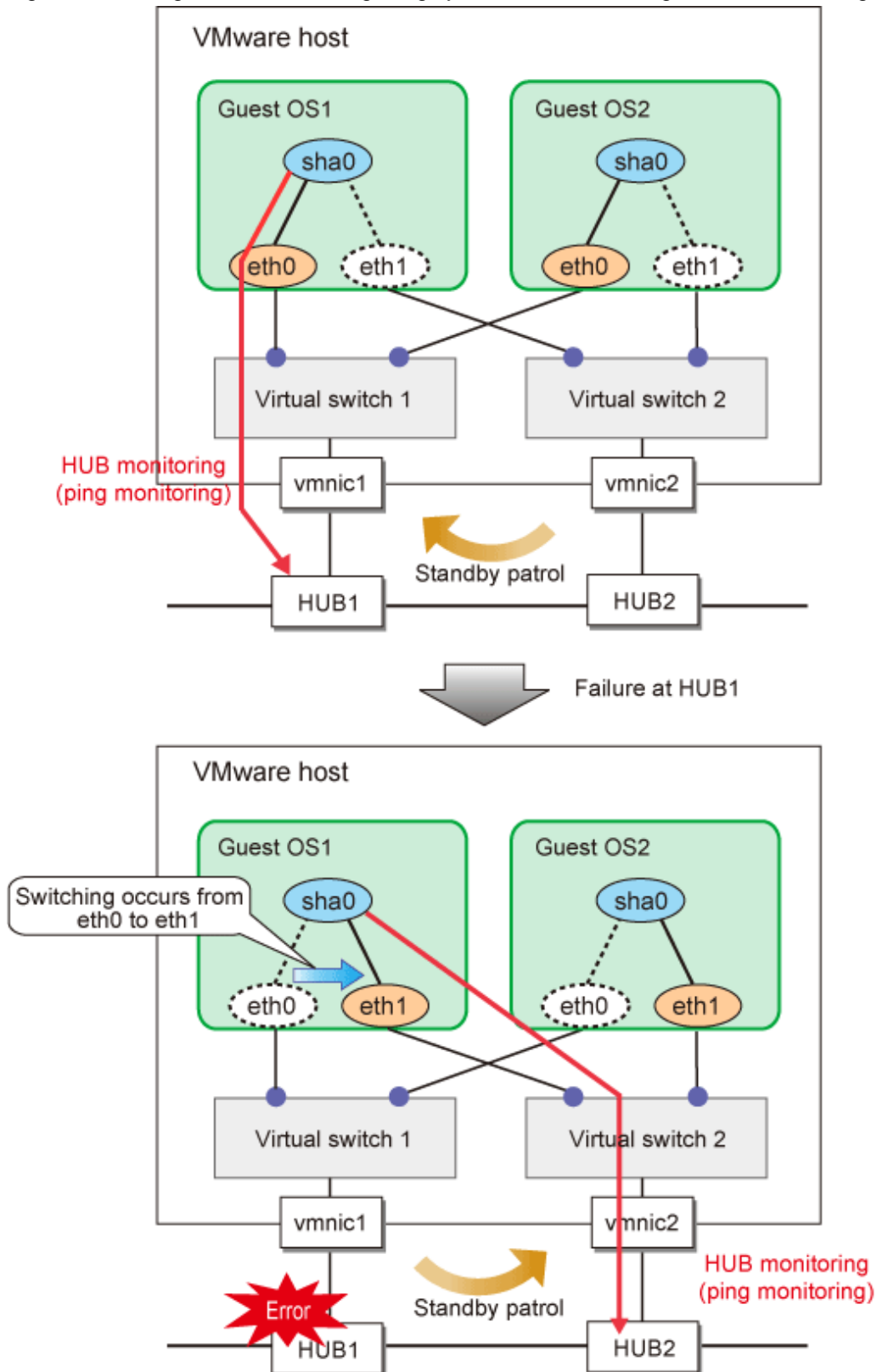
Figure D.1 Configuration for creating a highly reliable network on guest OSes in a single system
