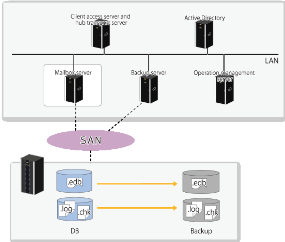
Figure 8.66 Non-DAG configuration (minimum configuration)
