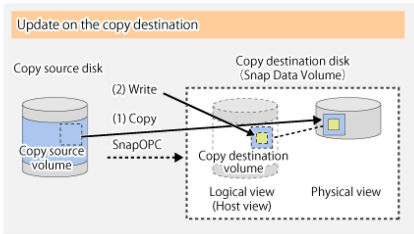
Figure 7.20 When the copy destination volume is updated
