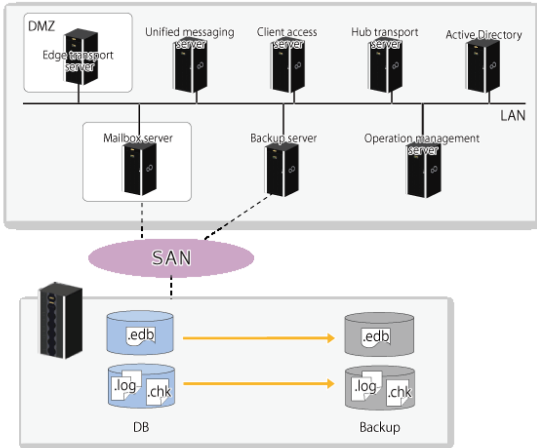
Figure 8.65 Non-DAG configuration
