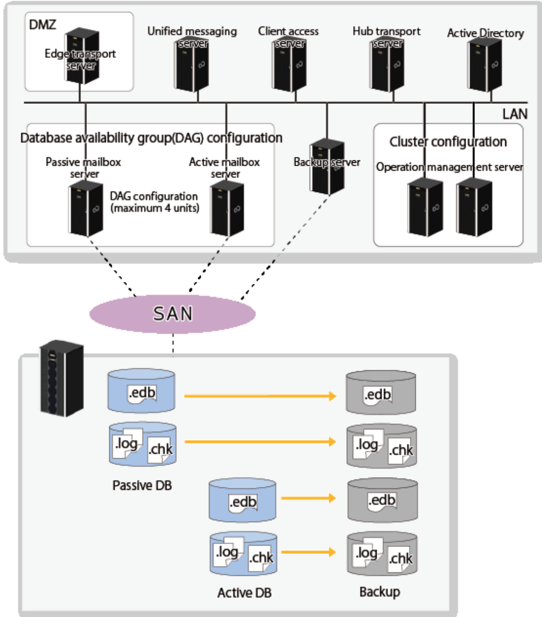
Figure 8.62 DAG configuration (Management Server: Cluster configuration)
