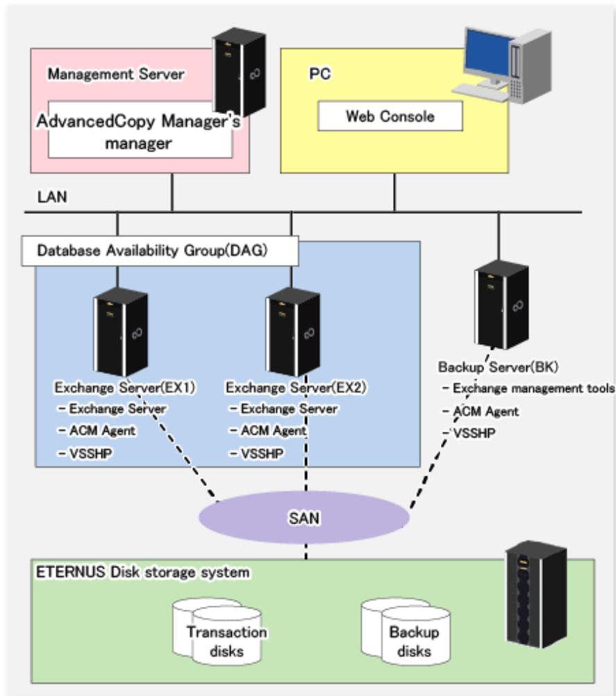
Figure 8.54 Server configuration
