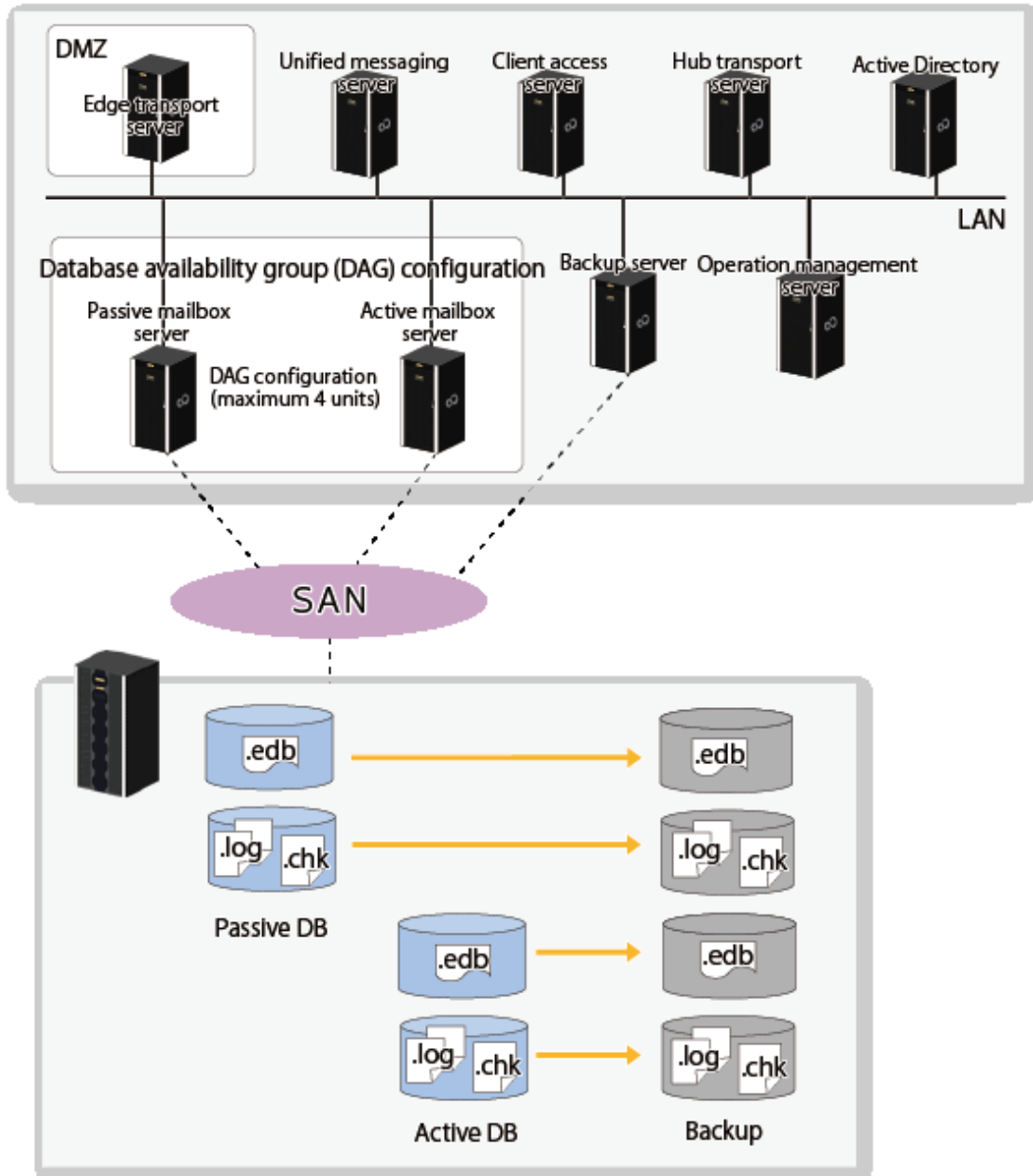
Figure 8.63 DAG configuration (Management Server: Non-cluster configuration)
