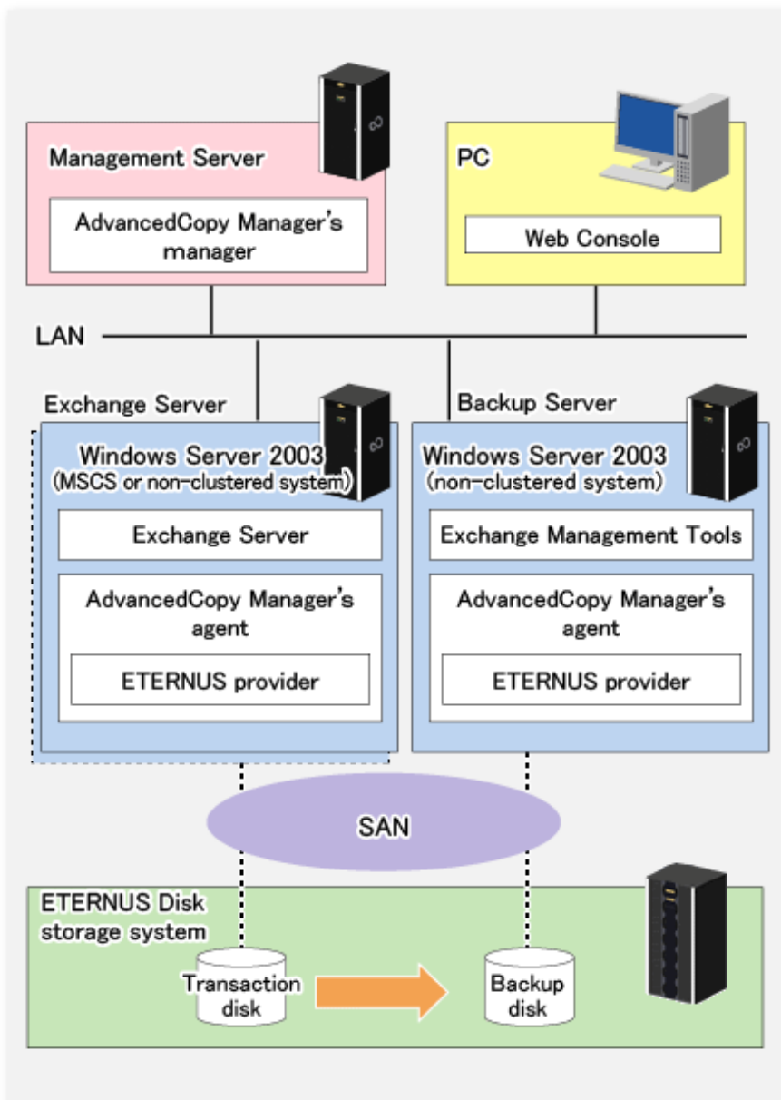
Figure 8.5 System configuration
