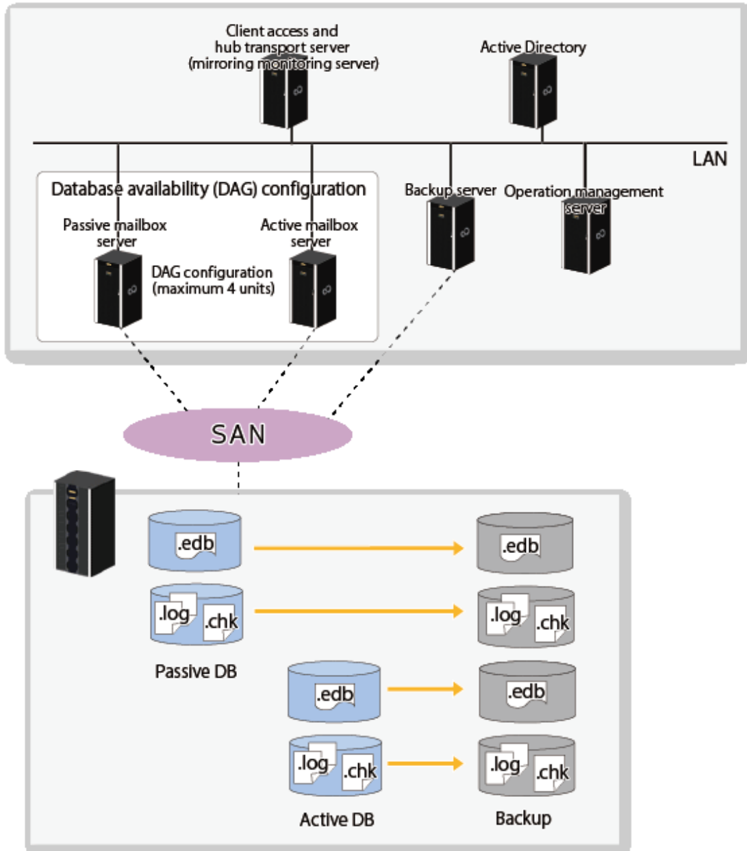
Figure 8.64 DAG configuration (minimum configuration)
