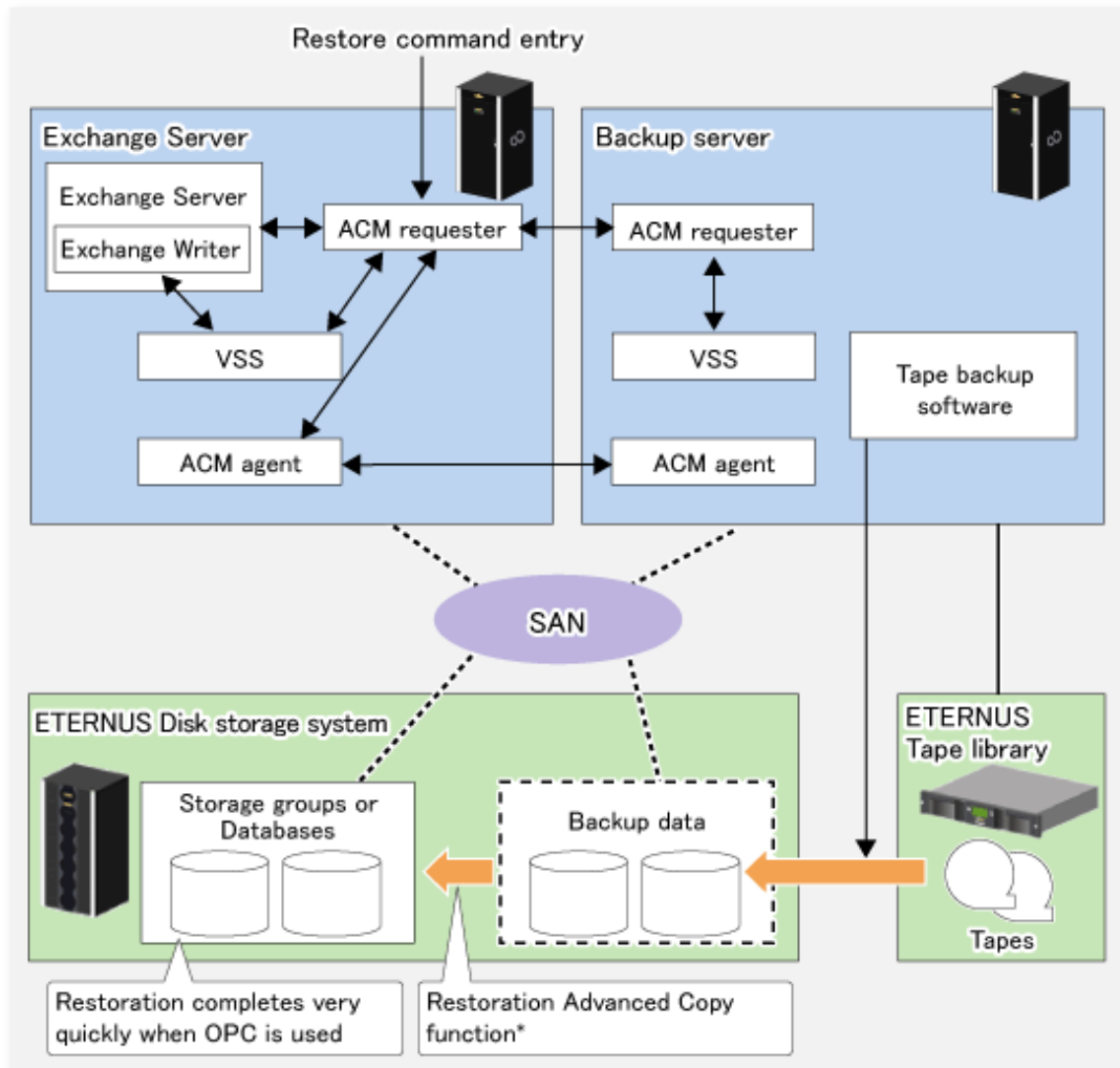
Figure 8.31 Exchange Server database restoration processing image
