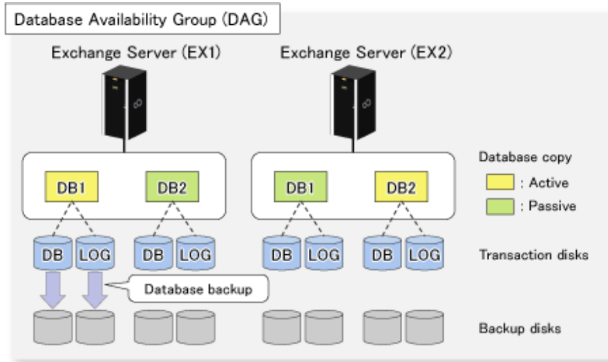
Figure 8.56 Backup of Exchange Server database
