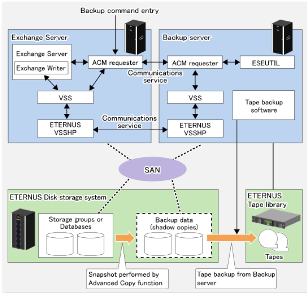
Figure 8.30 Exchange Server database backup processing image
