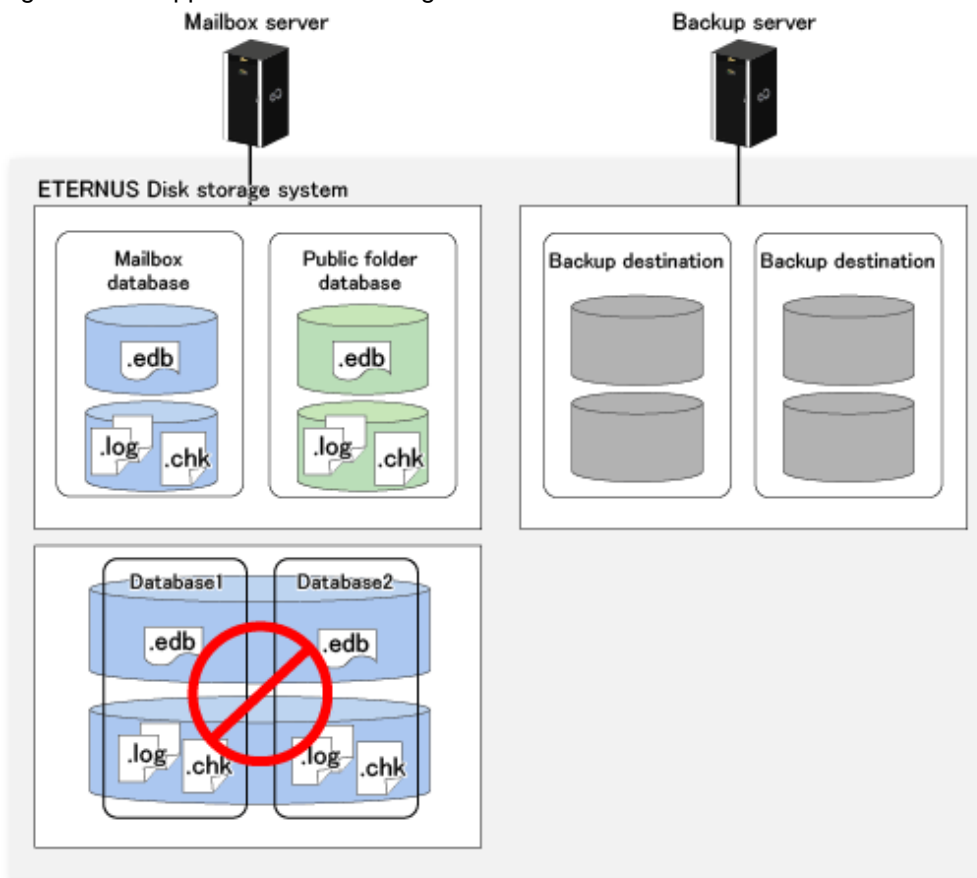
Figure 8.68 Supported volume configurations
