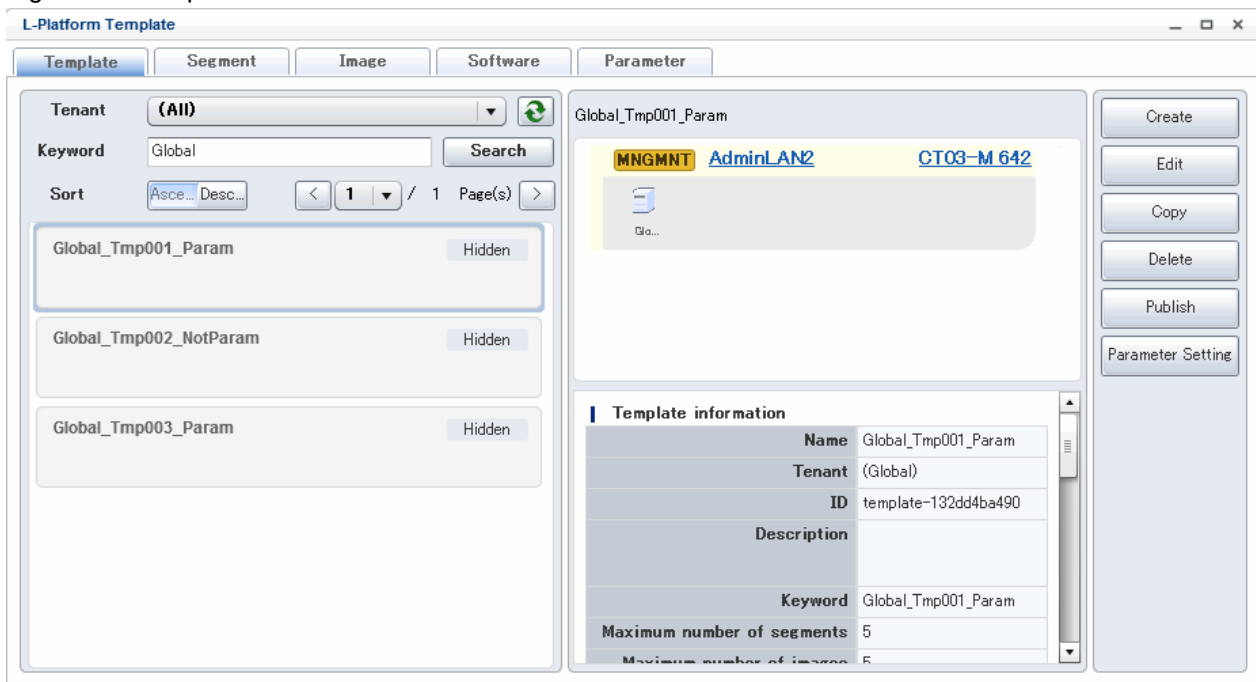
Figure 7.9 Template tab
