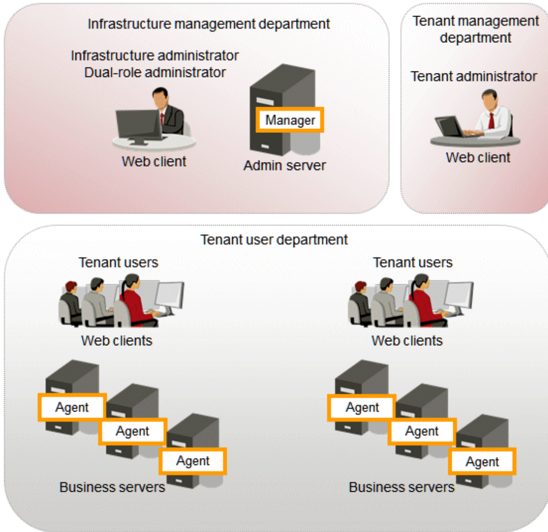
Figure 1.3 System configuration for managing software parameters
