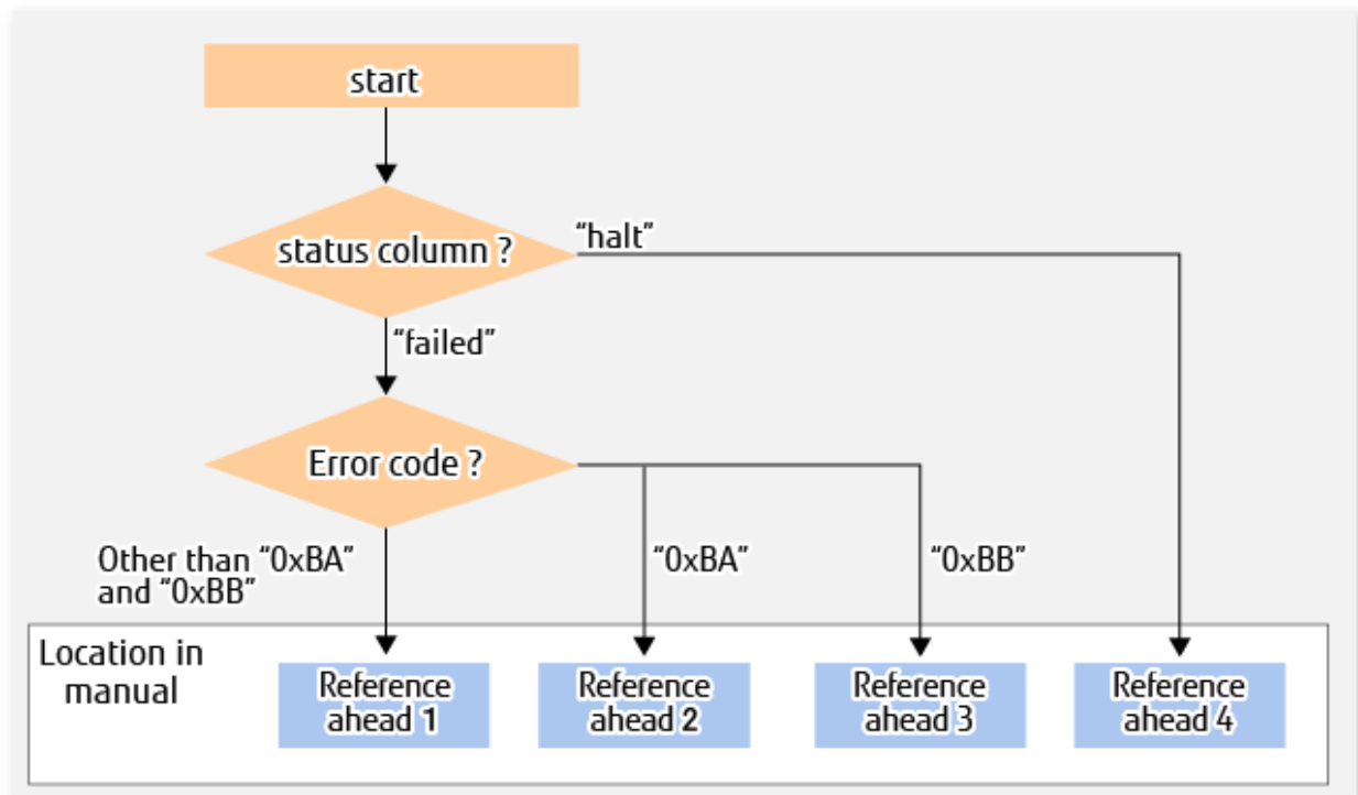
Figure 8.3 Troubleshooting Flow (When Fault Occurs During Replication)
