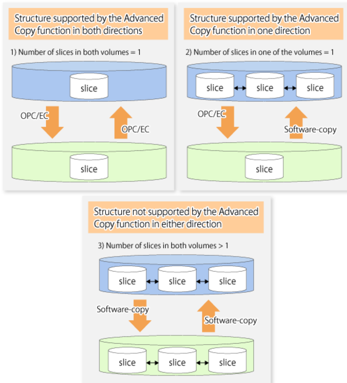
Figure 7.48 Copy Destination Volume Structures Supported by Advanced Copy Function
