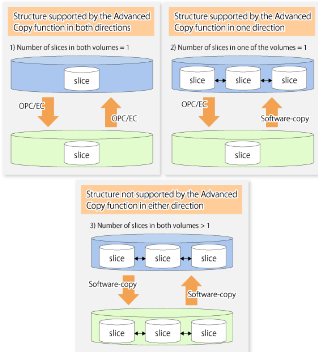
Figure 7.48 Copy destination volume structures supported by the Advanced Copy function
