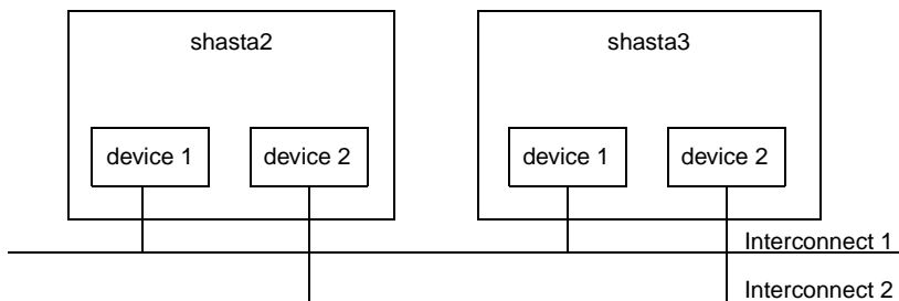
Figure 84: Conceptual view of CF interconnects
