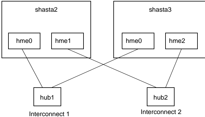
Figure 85: CF with Ethernet interconnects
