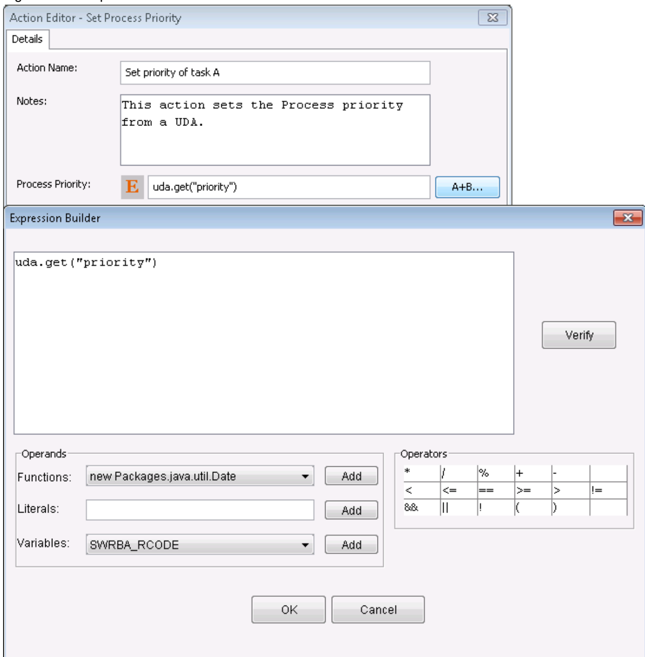
Figure 11.48 Expression Builder
