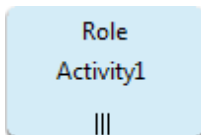
Figure 6.22 Activity Node
