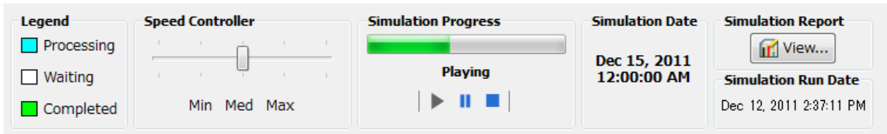
Figure 12.11 Simulation Controller
