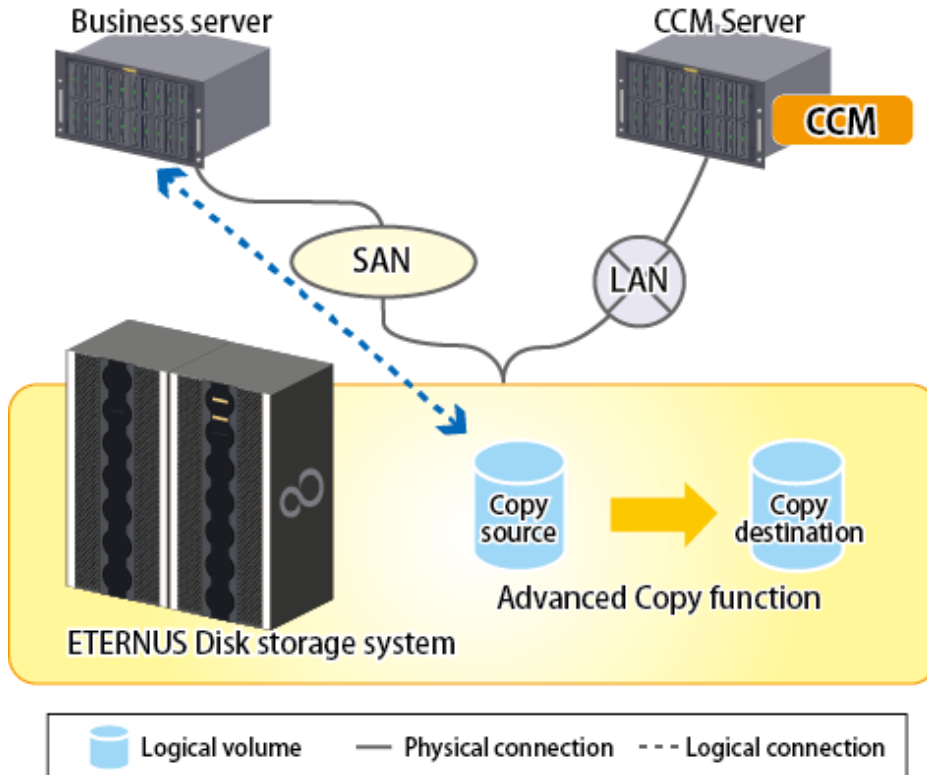
Figure 1.4 Sample configuration where intra-box copy is executed (using Copy command via LAN)
