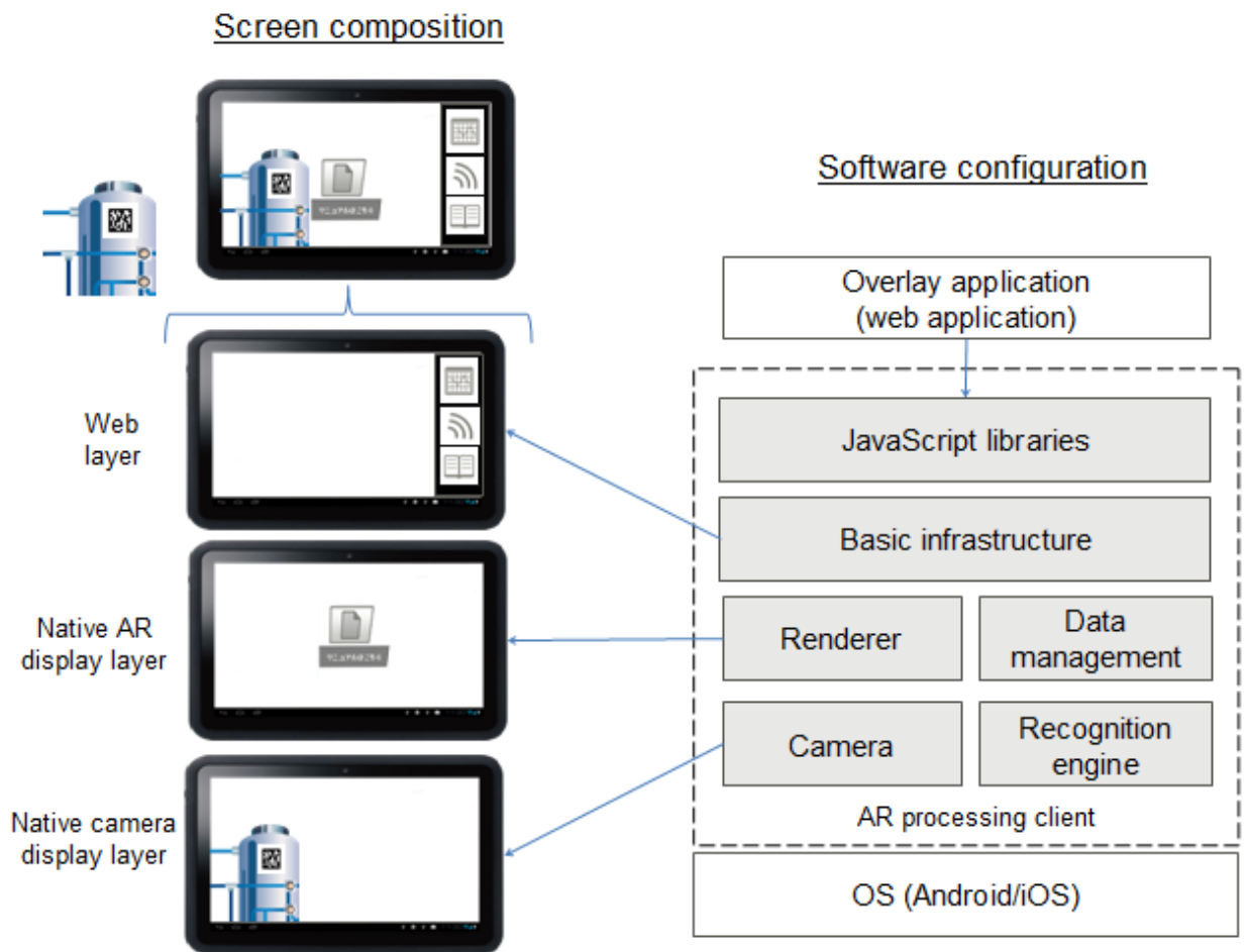
Figure 3.1 Example screen composition
