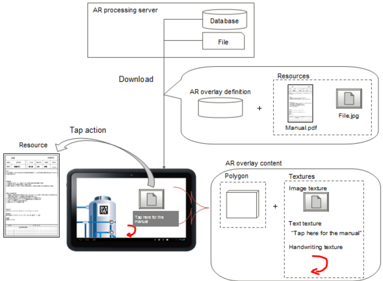
Figure 1.2 Example of operations up to rendering of AR overlay content
