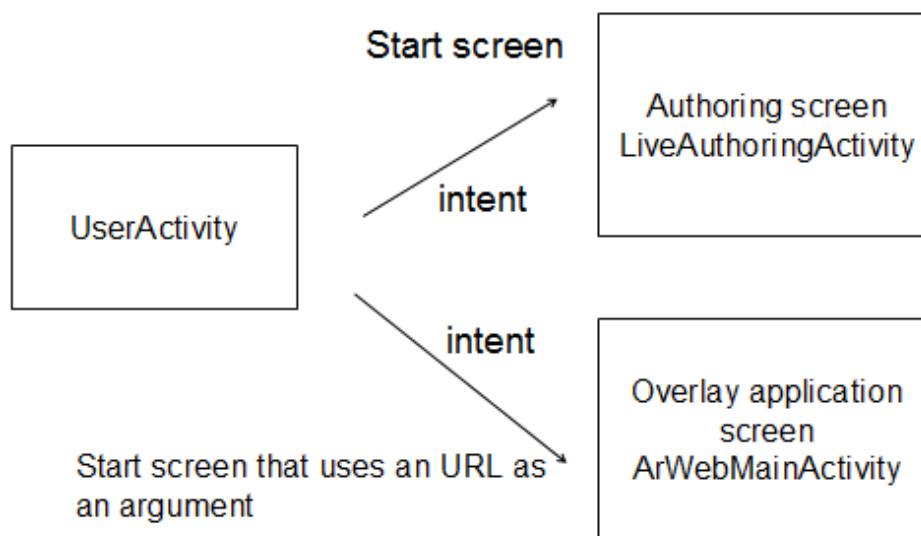
Figure 4.1 Image of native application operation
