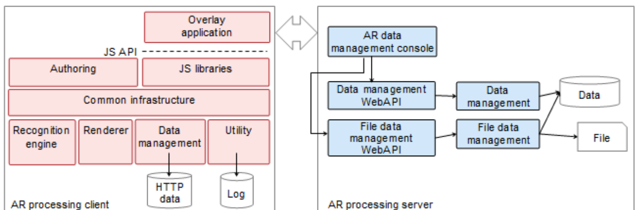
Figure 1.1 Architecture
