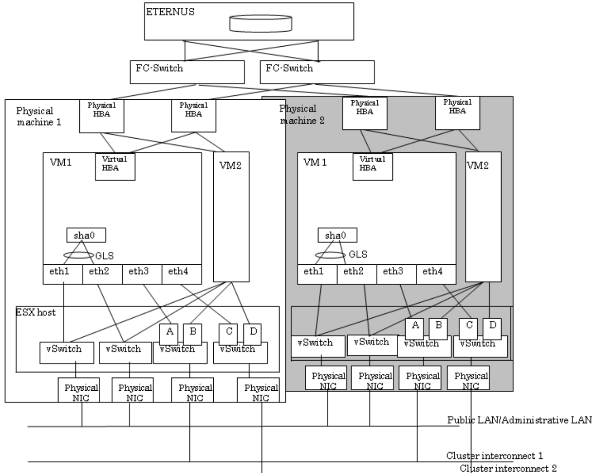
Figure H.2 Sample configuration of a cluster between guest OEs on two ESX hosts
