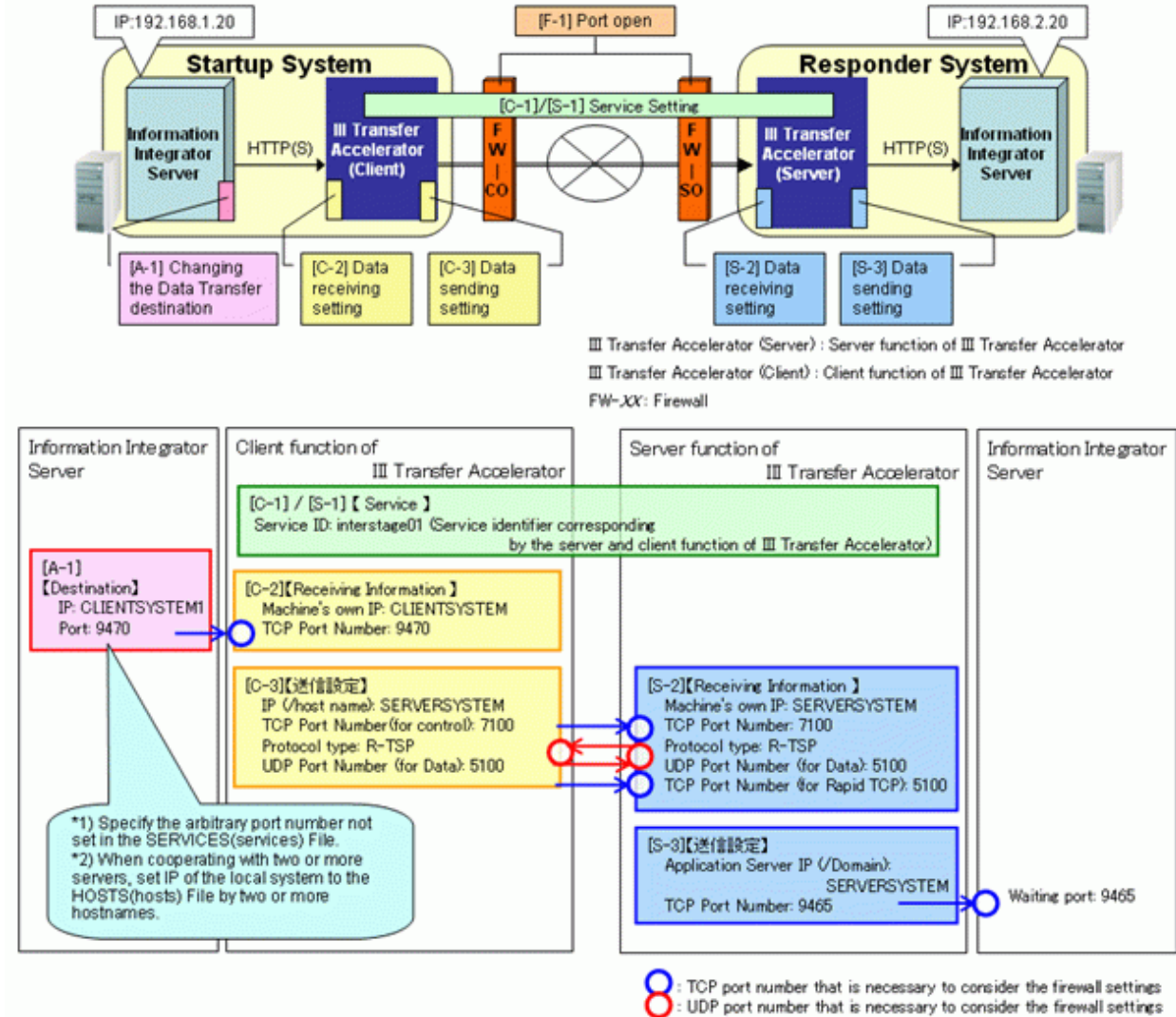
Figure C.2 Example of the system configuration and the set up information
