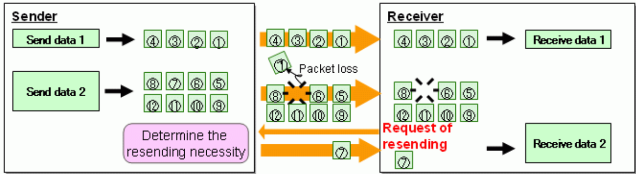
Figure 1.4 Mechanism of UNAP
