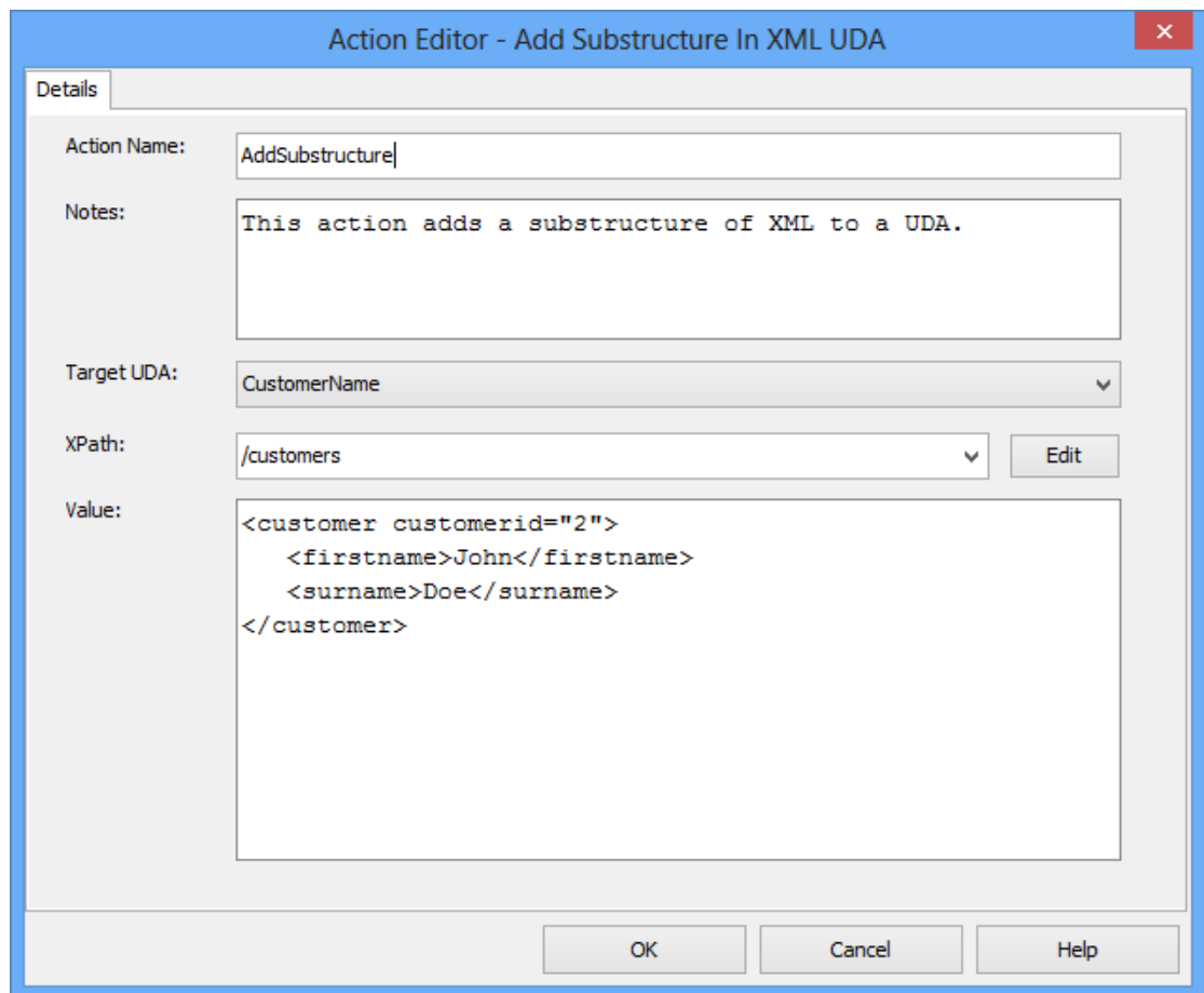
Figure 189: Adding a Substructure in XML UDA
