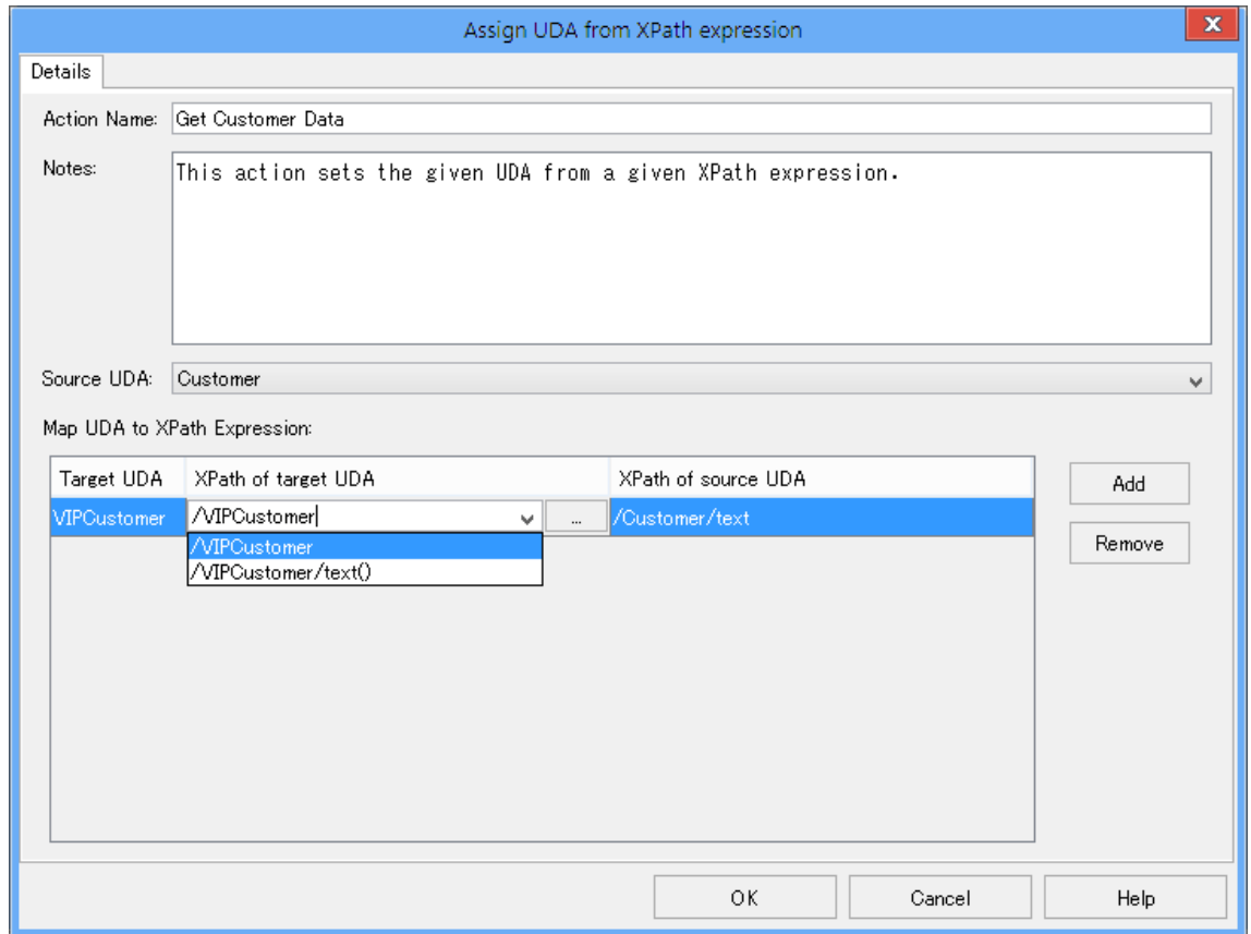
Figure 190: Extracting Data from an XML String - XPath of target UDA
