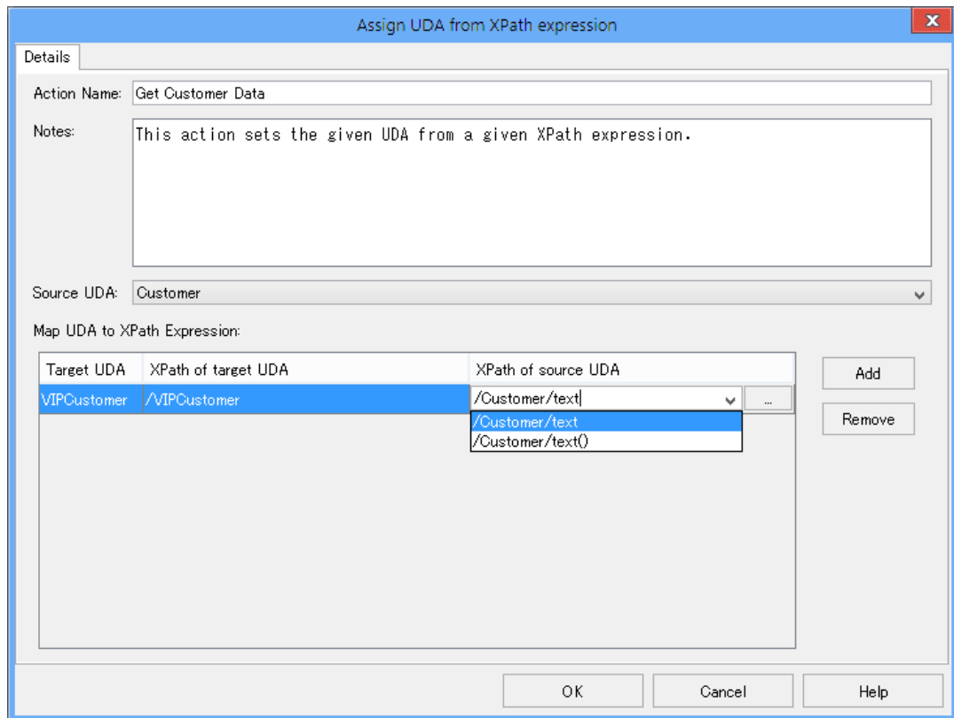
Figure 191: Extracting Data from an XML String - XPath of source UDA
