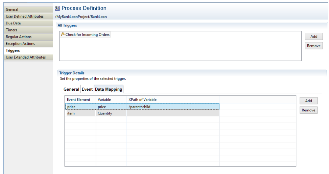
Figure 227: Defining Data Mappings
