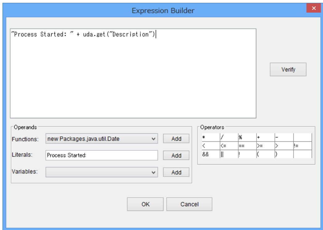
Figure 235: Building a Sample JavaScript Expression
