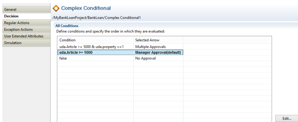
Figure 123: Defining Complex Conditions
