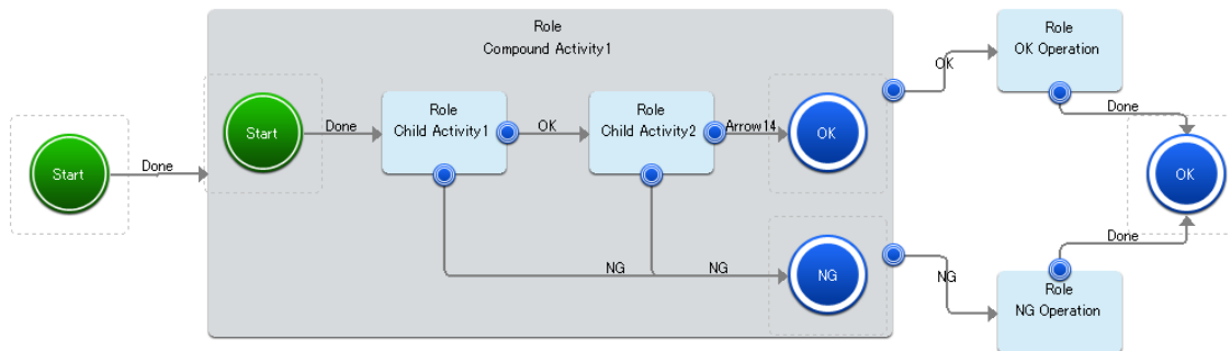
Figure 108: Compound Activity Node
