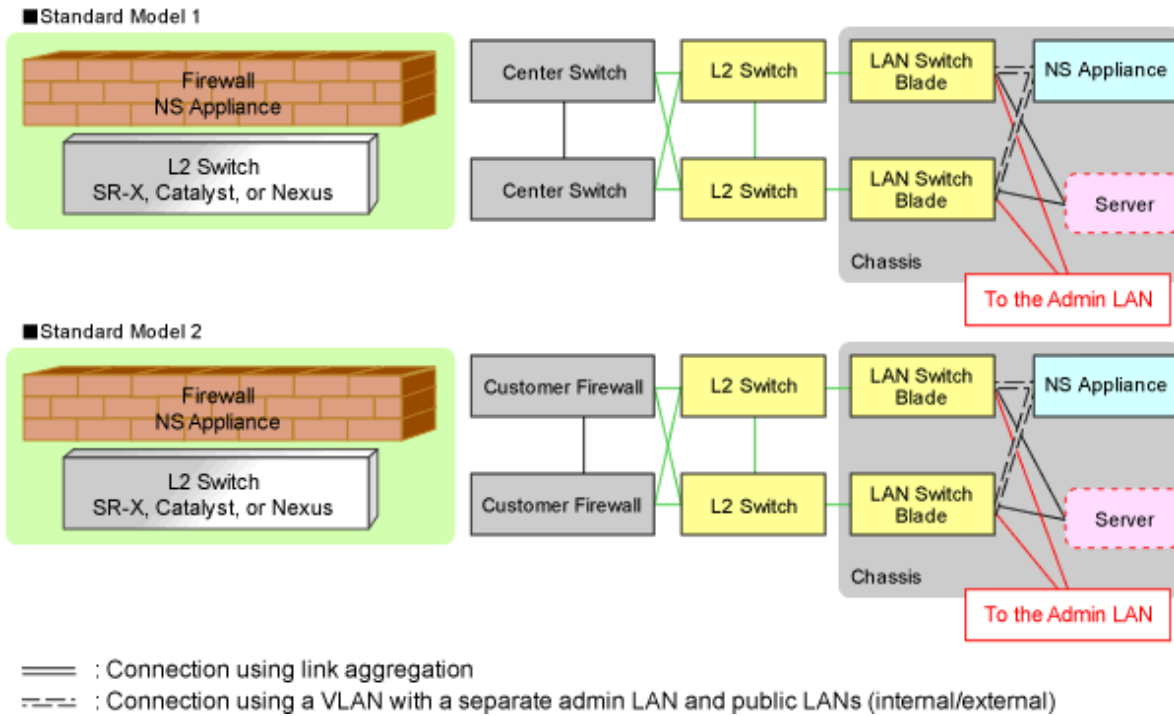
Figure G.3 Standard Model Configurations of Sample Scripts (NSAppliance)
