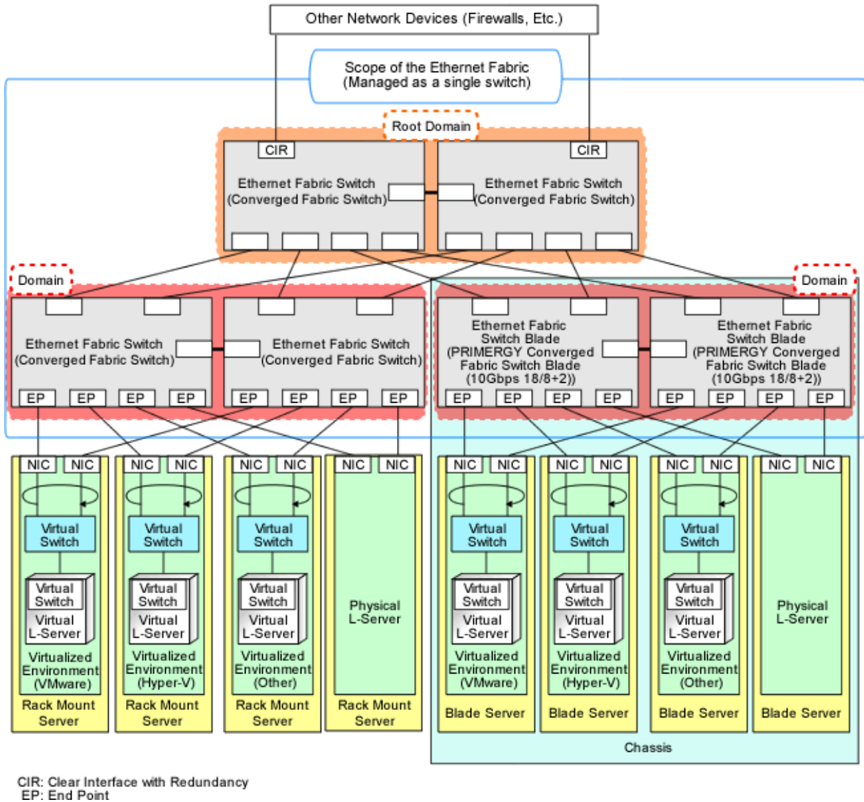
Figure H.1 Network Device Management Unit
