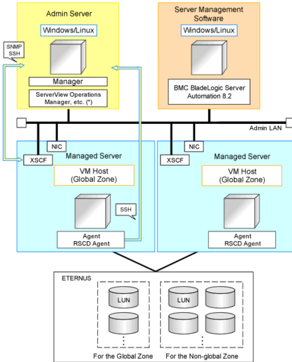
Figure E.18 System Configuration Example Using Solaris Zones
