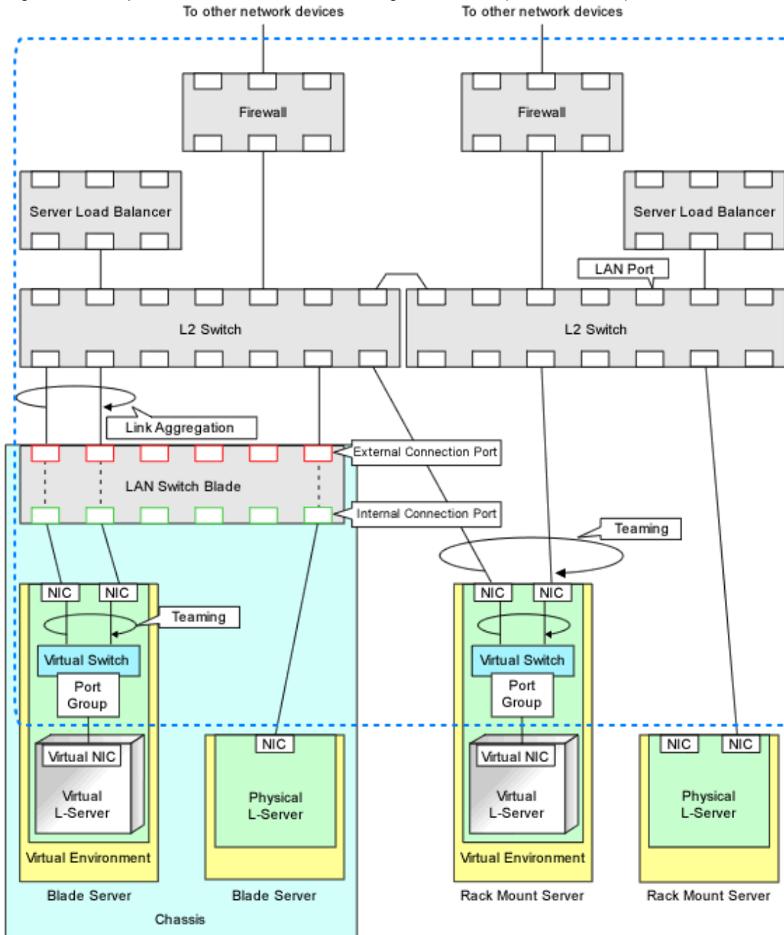
Figure 2.4 Scope of Automatic Network Settings Execution (For L2 Switch)
