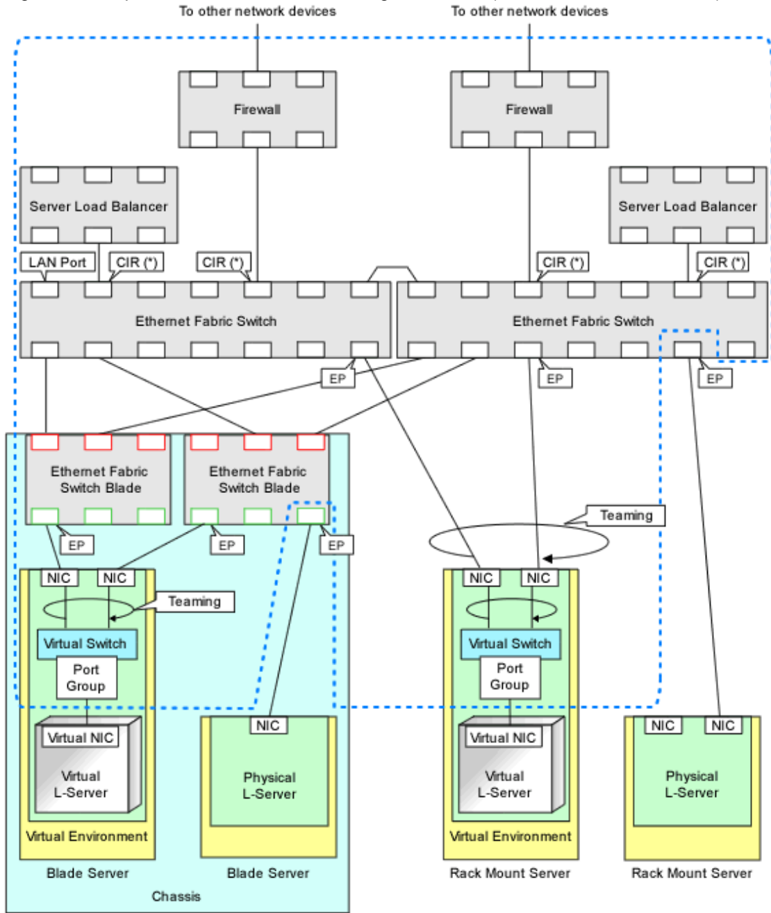
Figure 2.5 Scope of Automatic Network Settings Execution (For Ethernet Fabric Switch)
