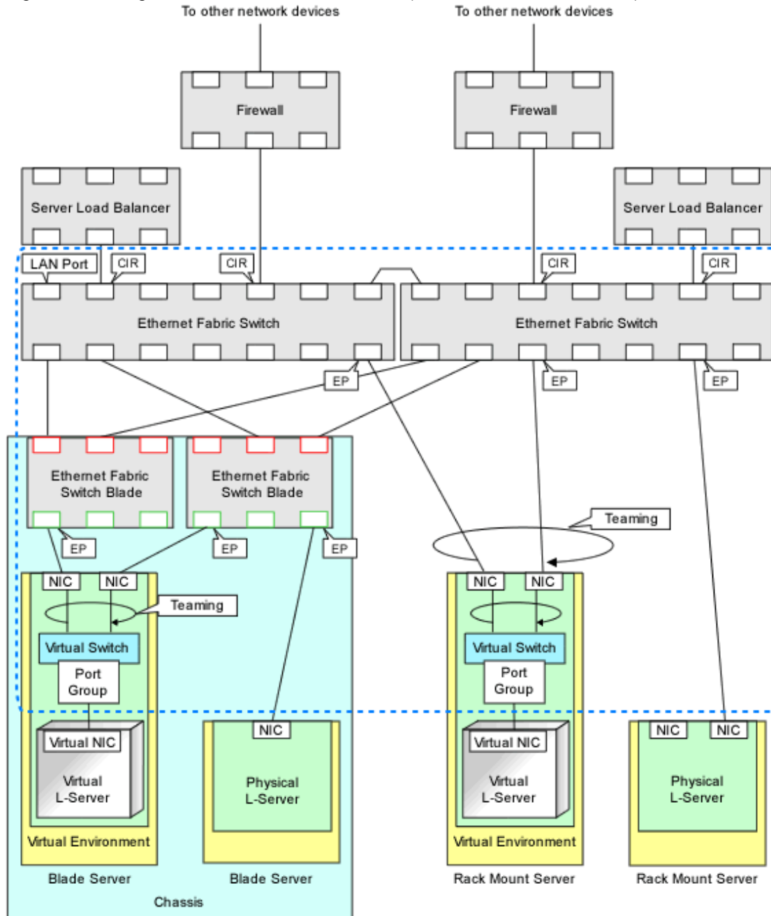
Figure 2.7 Hiding of Network Device Information (For Ethernet Fabric Switch)
