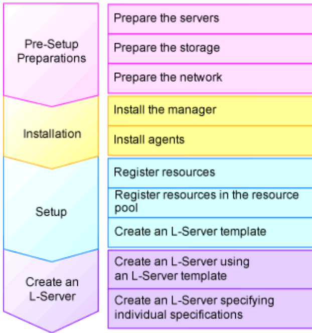
Figure E.24 Flow of L-Server Creation
