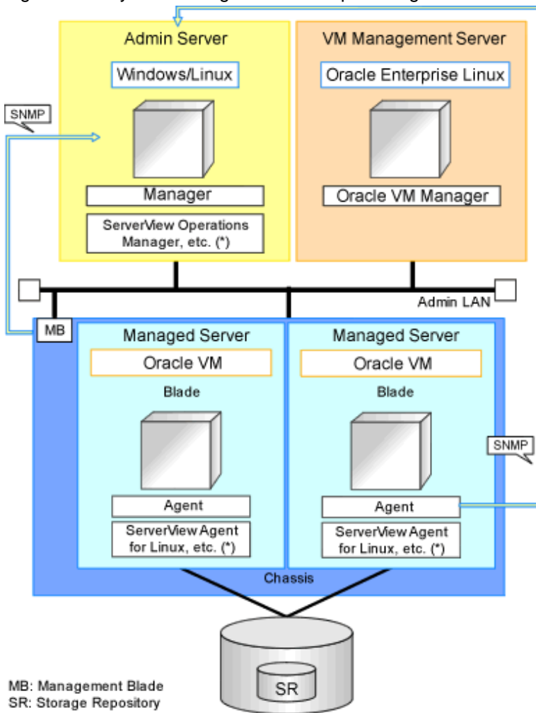
Figure E.14 System Configuration Example Using OVM for x86 2.2
