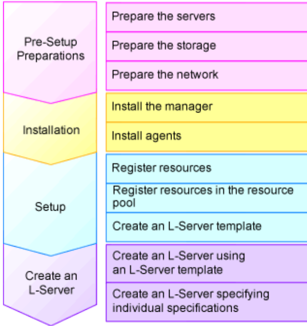
Figure E.27 Flow of L-Server Creation
