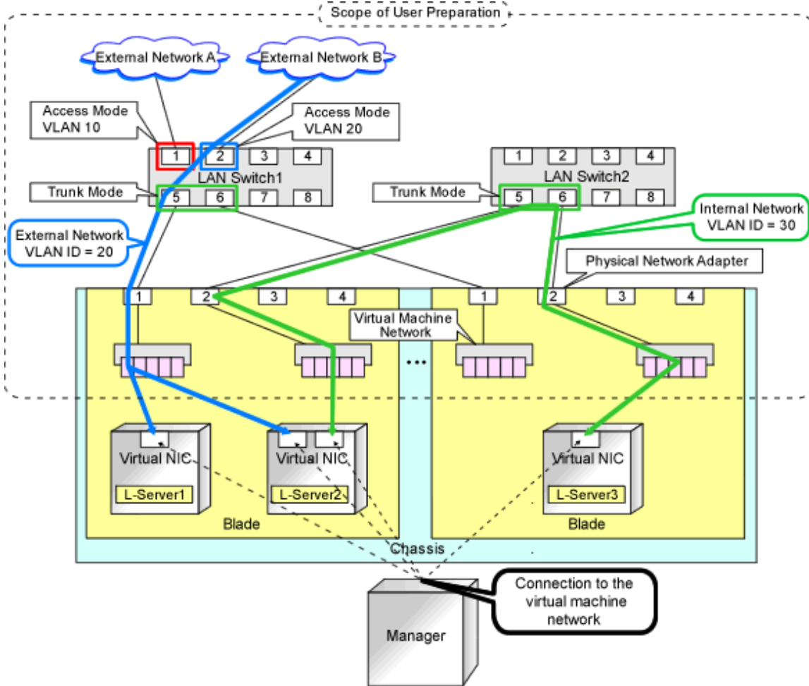
Figure E.26 Network Configuration Example
