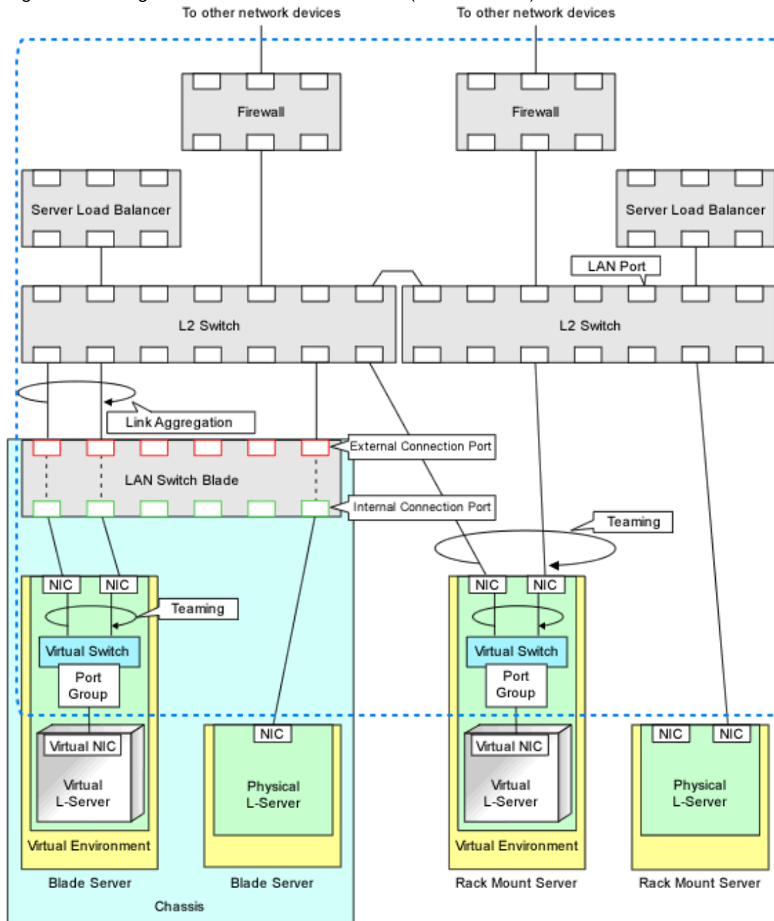
Figure 2.6 Hiding of Network Device Information (For L2 Switch)
