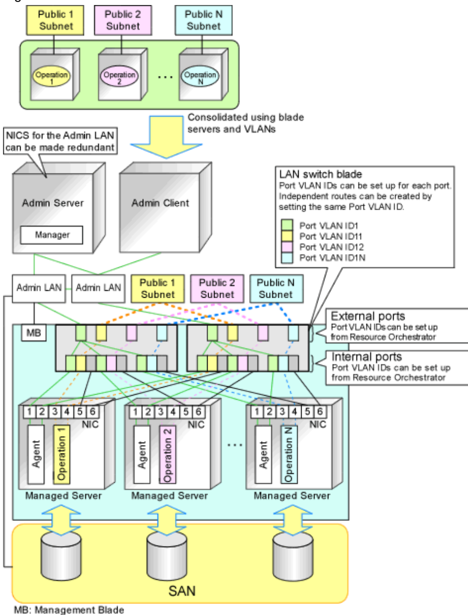
Figure 9.14 With Port VLANs
