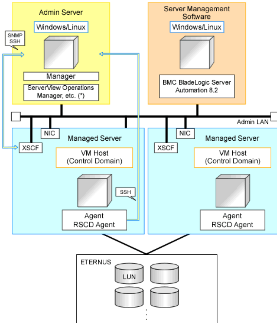
Figure E.21 System Configuration Example Using OVM for SPARC
