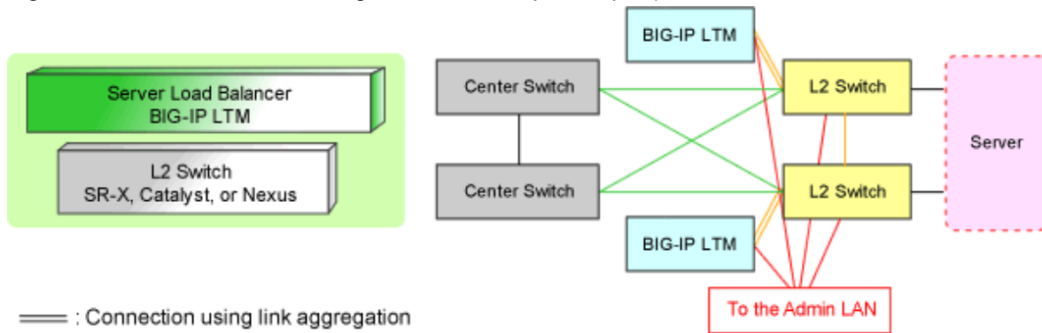
Figure G.7 Standard Model Configurations of Sample Scripts (Server Load Balancers:BIG-IP LTM Series)
