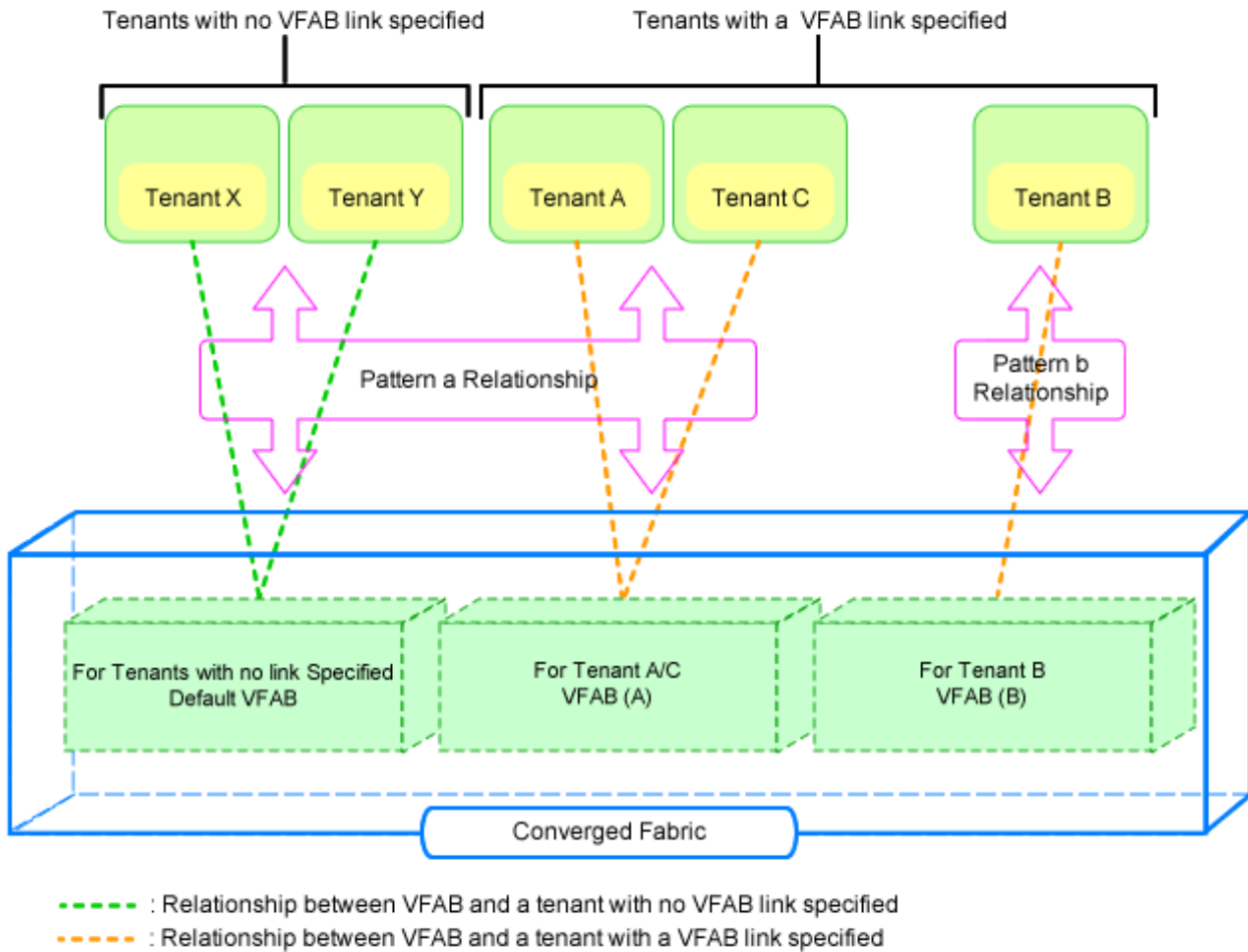
Figure H.4 Relations between Tenants and Virtual Fabrics
