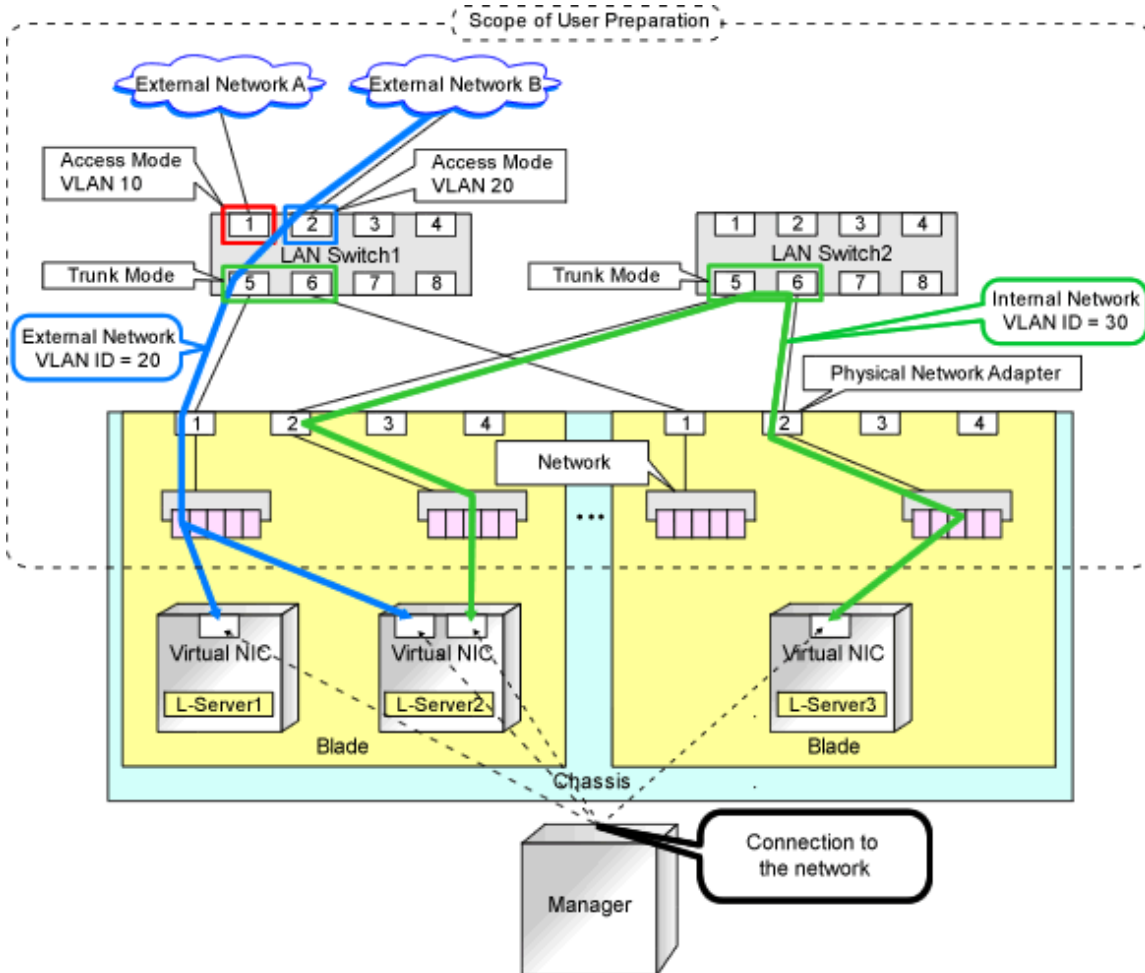
Figure E.23 Network Configuration Example
