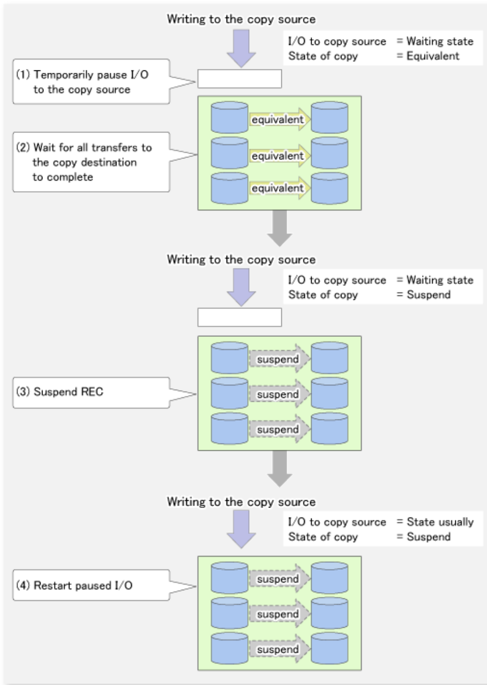
Figure 6.44 Internal operation of ETERNUS Disk storage system
