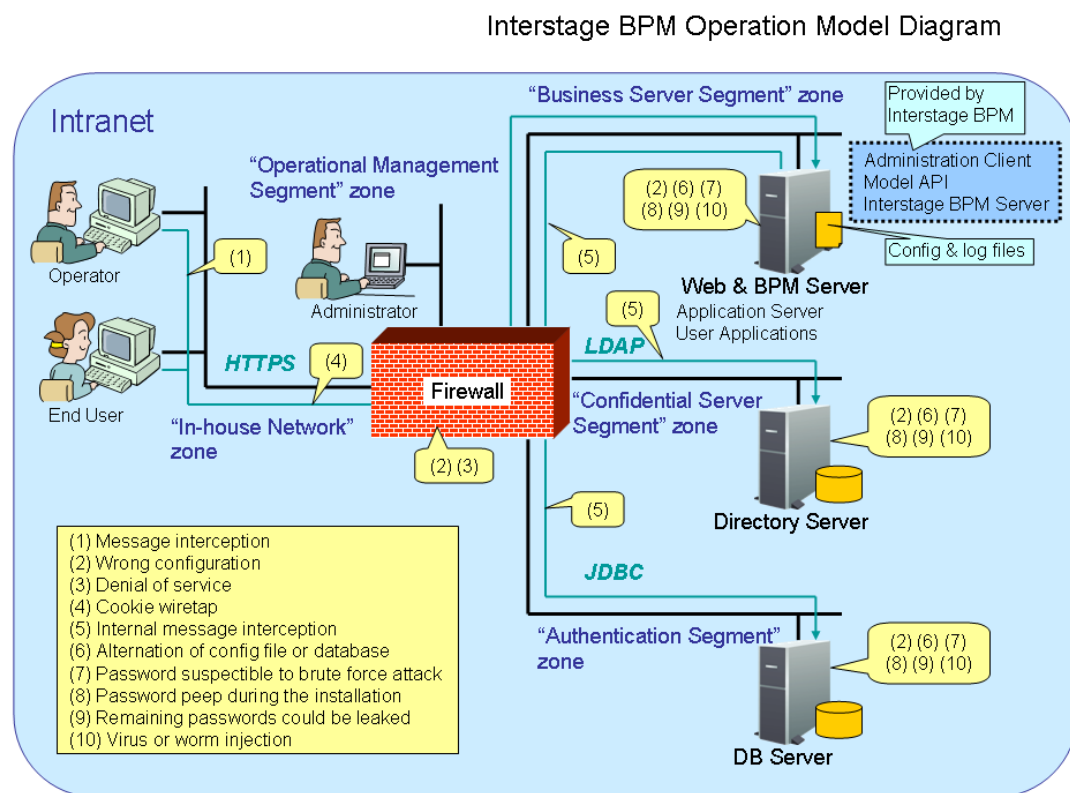
Figure 18: Interstage BPM Operation Model
