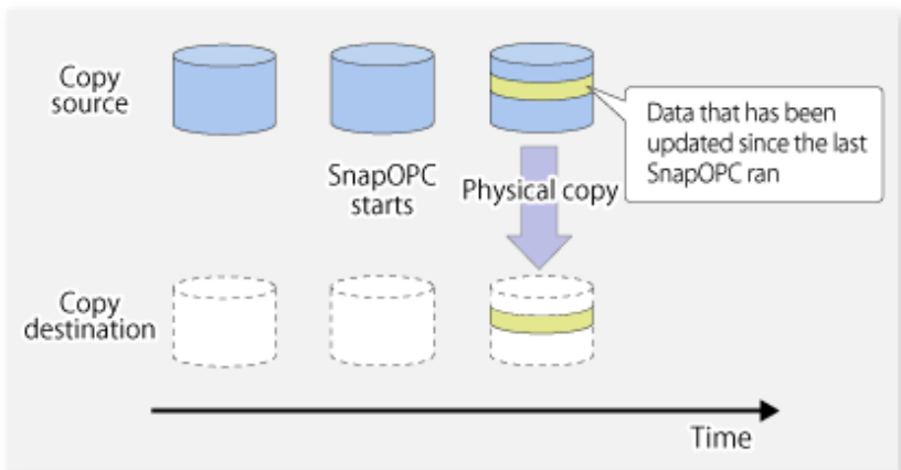
Figure 7.4 SnapOPC replication
