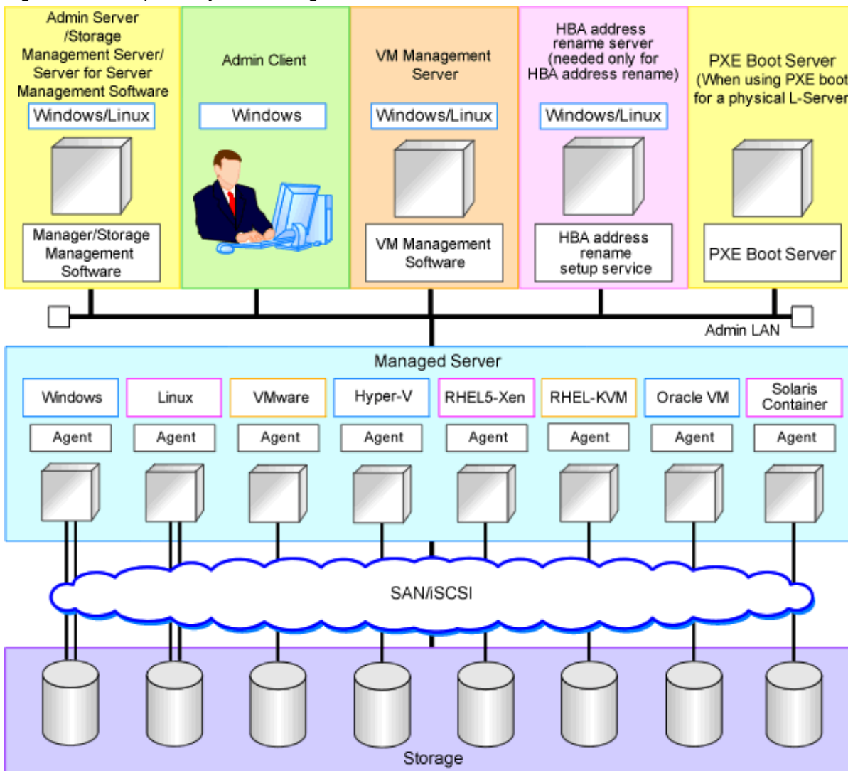
Figure 2.8 Example of System Configuration
