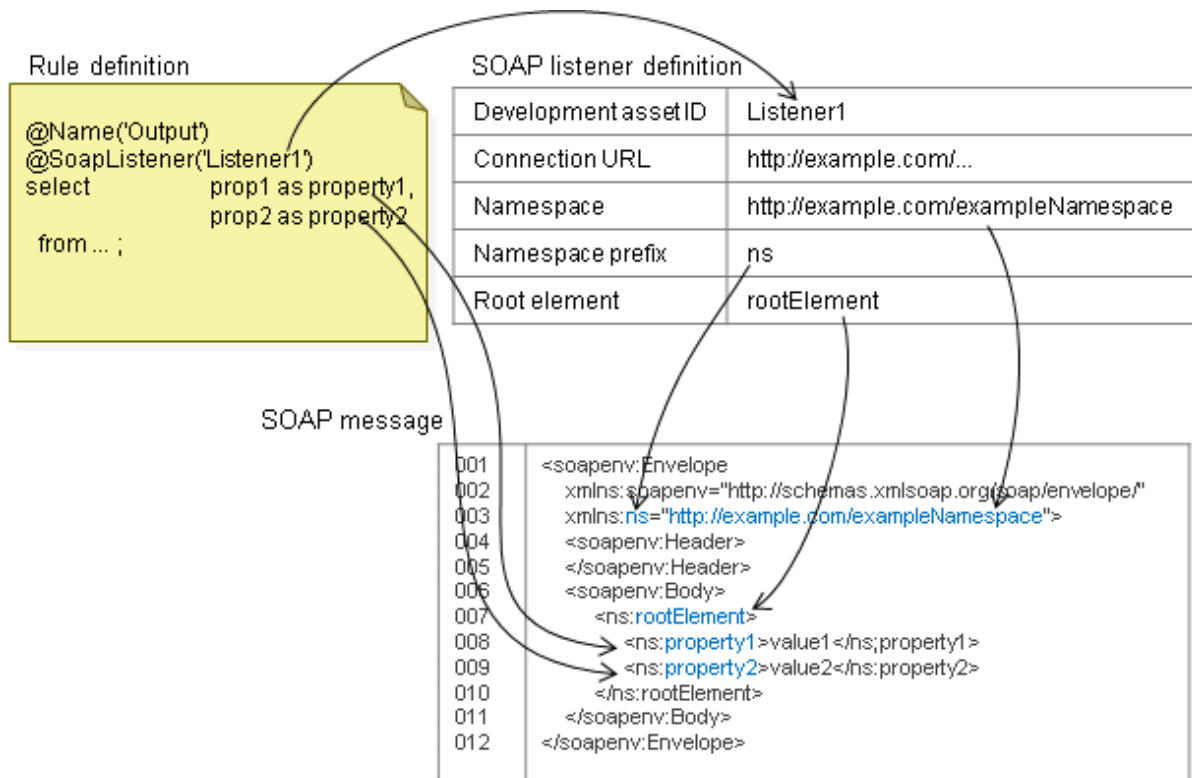
Figure 5.4 Example of the association between a rule definition and a listener definition, and the SOAP messages to be sent
