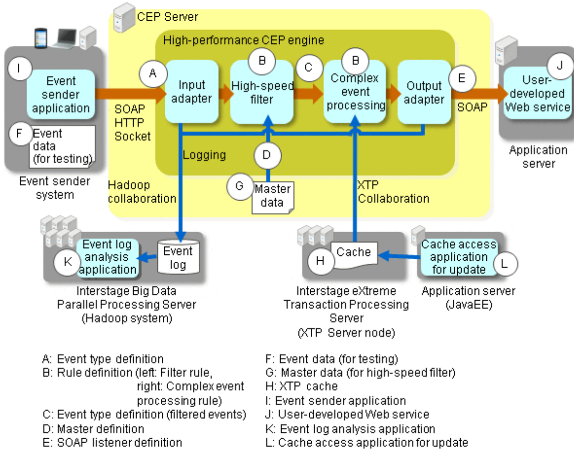
Figure 5.1 Deployment destinations of development assets
