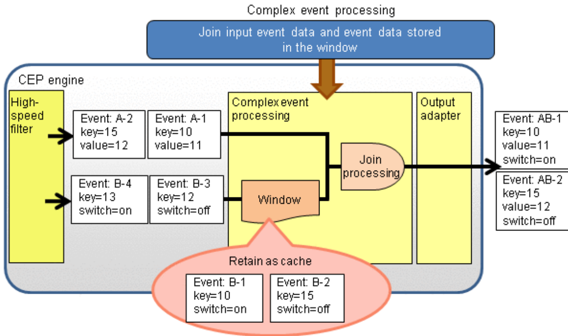
Figure 2.3 Example of join processing of cache data and input events using a window
