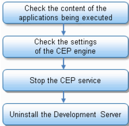
Figure 4.4 Flowchart for canceling Hadoop collaboration
