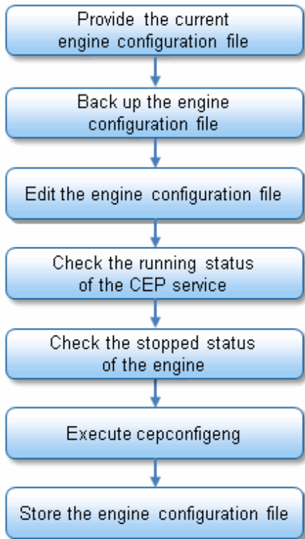
Figure 4.2 Flowchart for deleting a CEP engine
