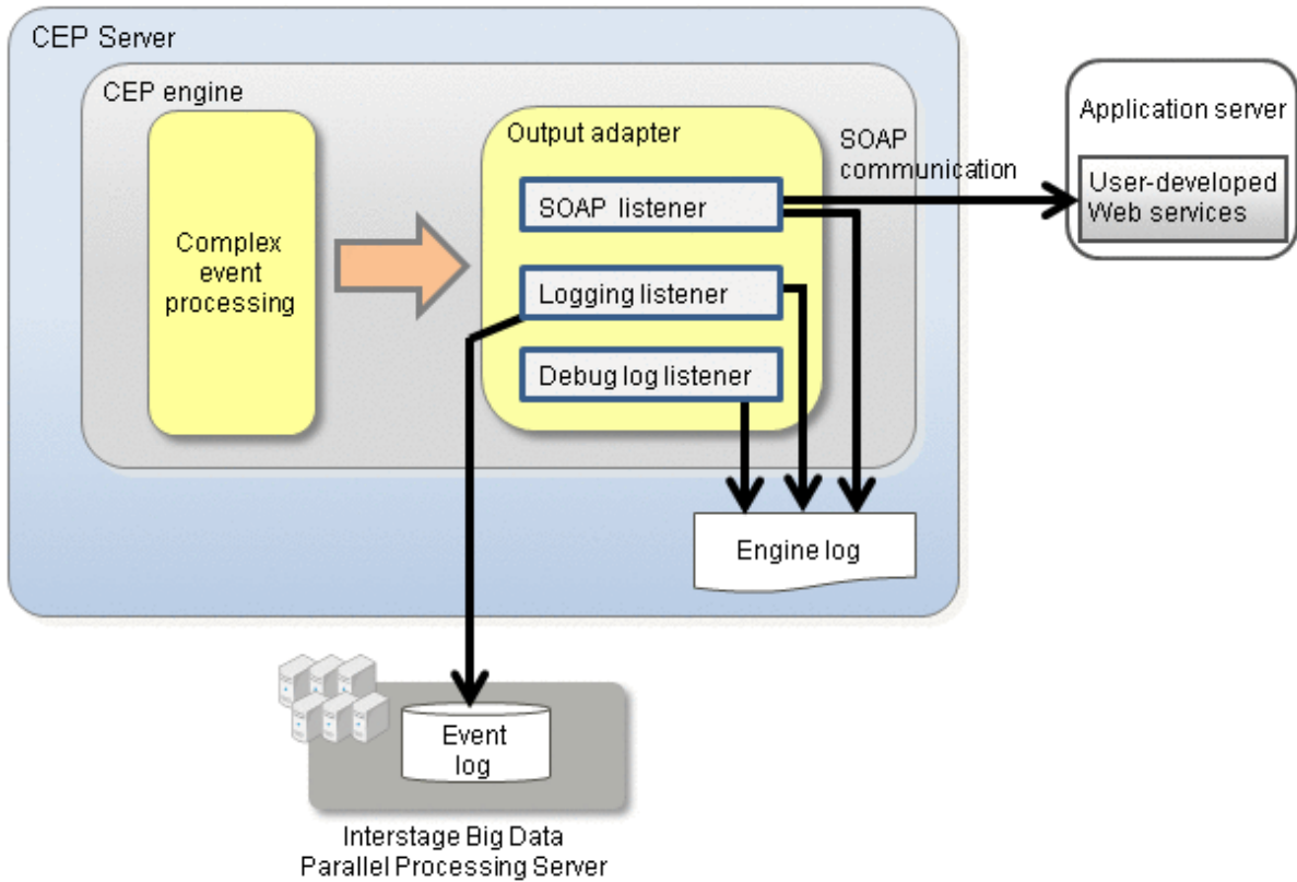
Figure 2.5 Output adapter
