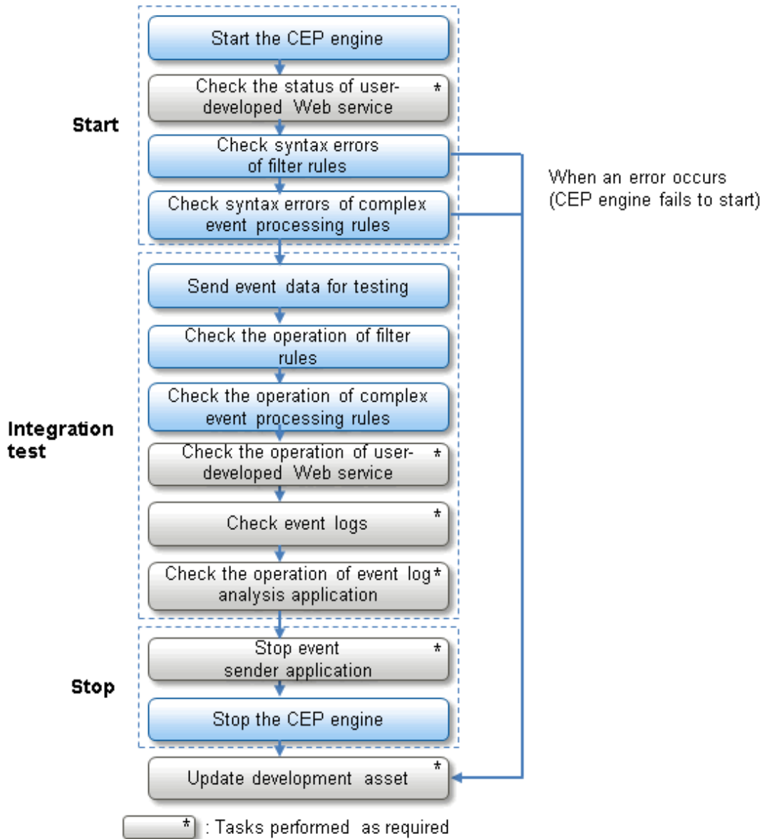
Figure 5.6 Integration test flow
