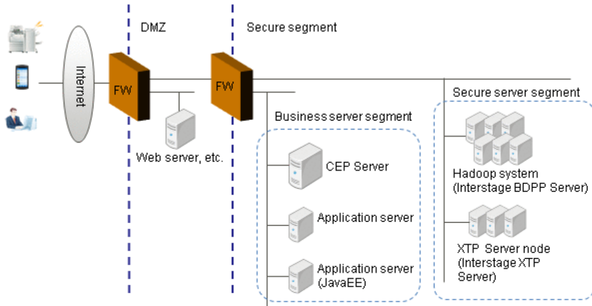
Figure 6.1 Typical operation model of this product
