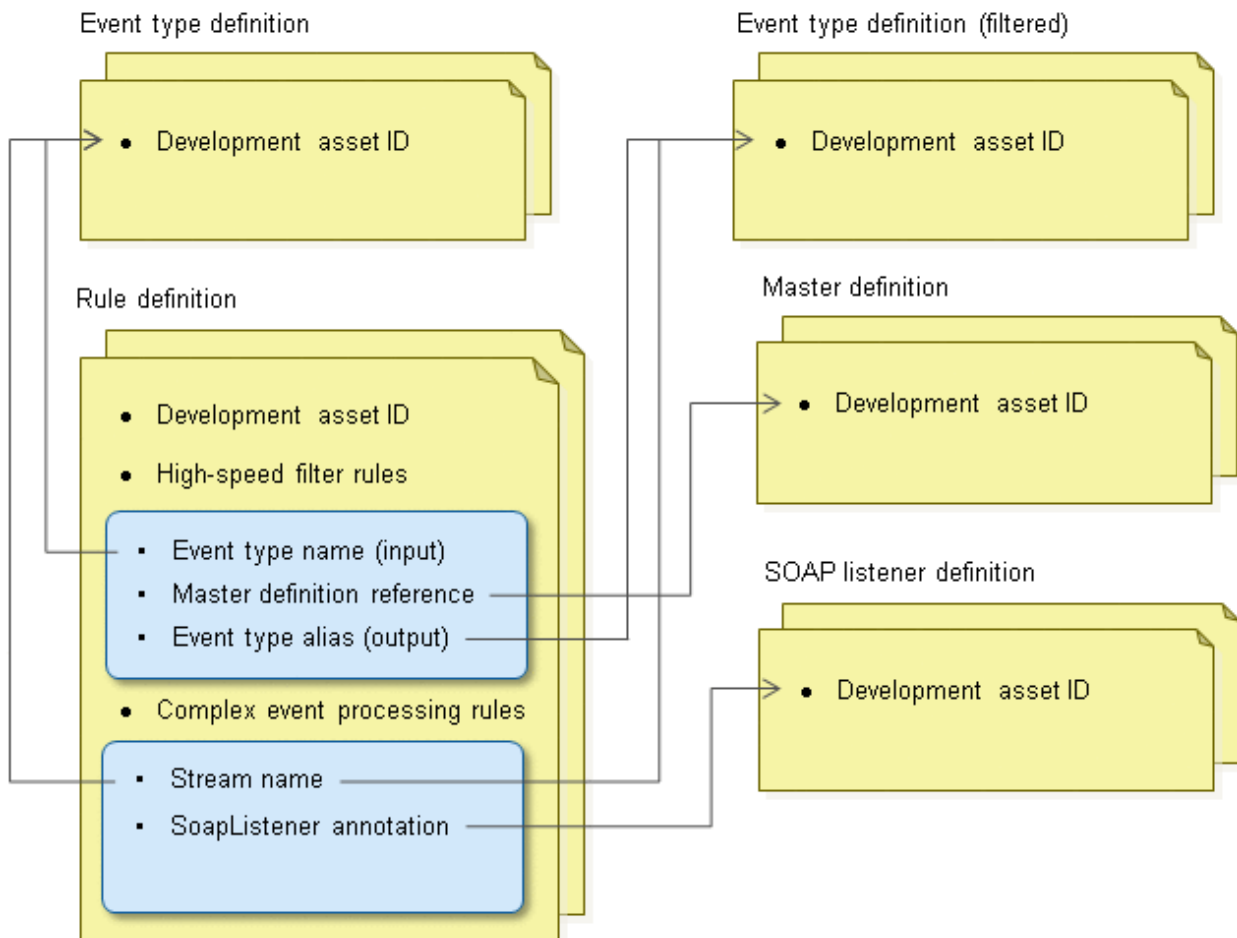
Figure 5.3 Association between development asset IDs and definition information
