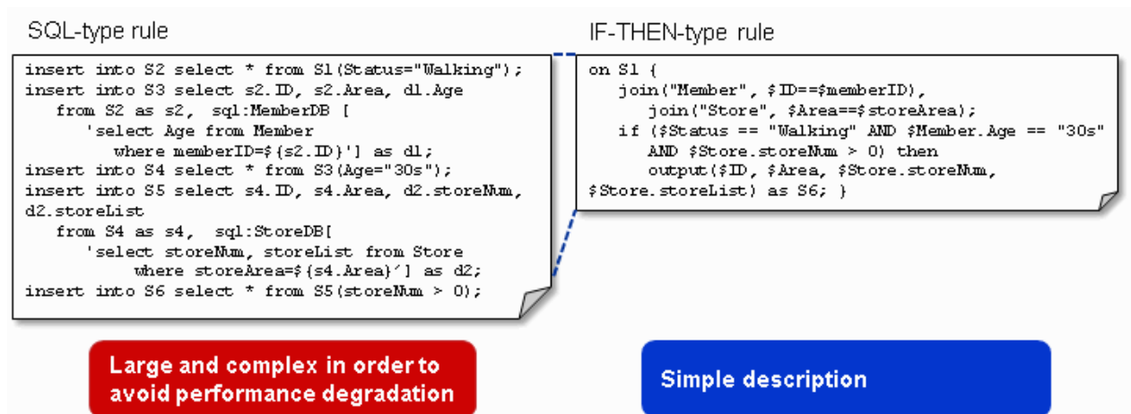
Figure 1.2 Comparison between an SQL-type rule and an IF-THEN-type rule describing a join with master data
