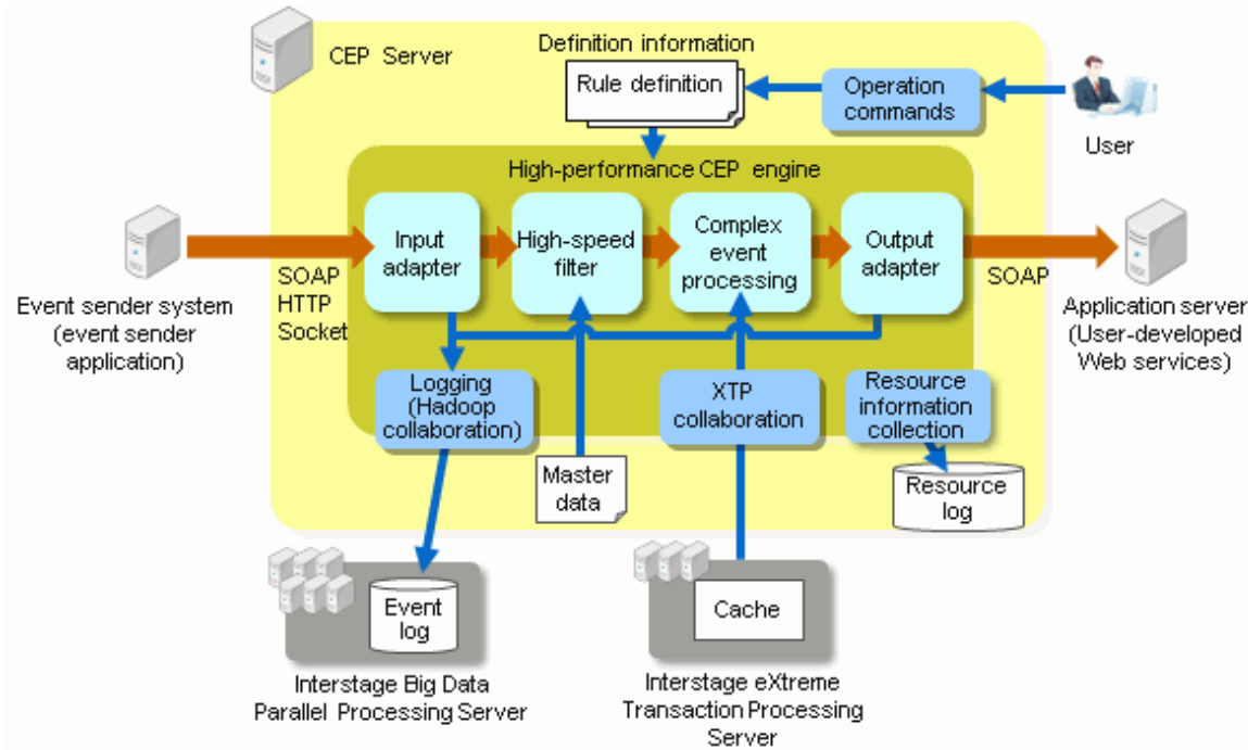
Figure 1.5 List of features provided
