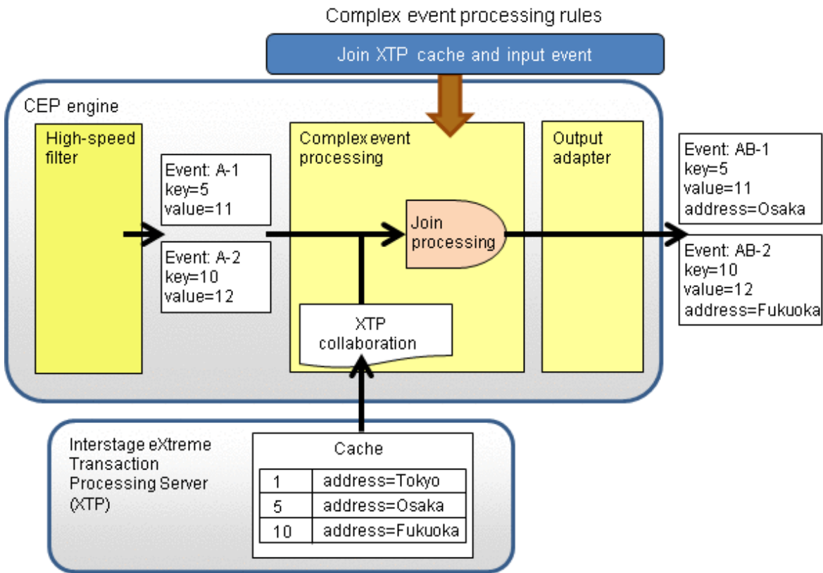
Figure 2.4 Example of XTP collaboration
