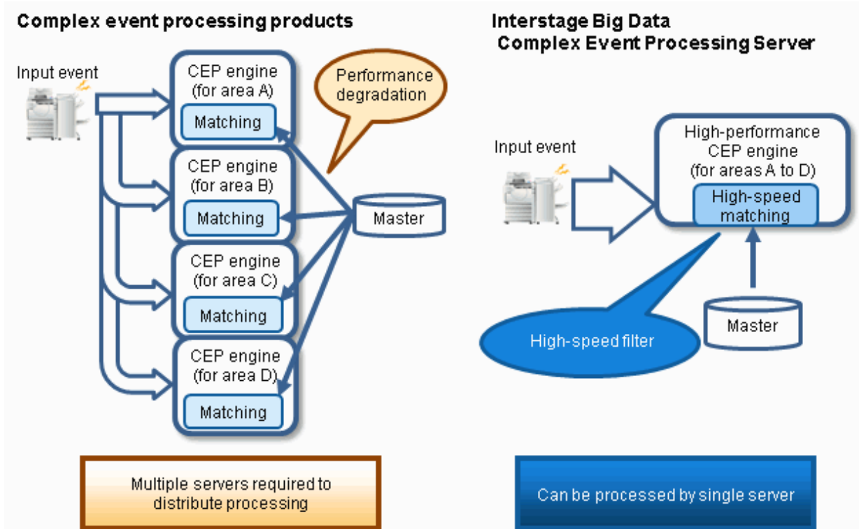
Figure 1.1 Comparison when massive volumes of events are processed
