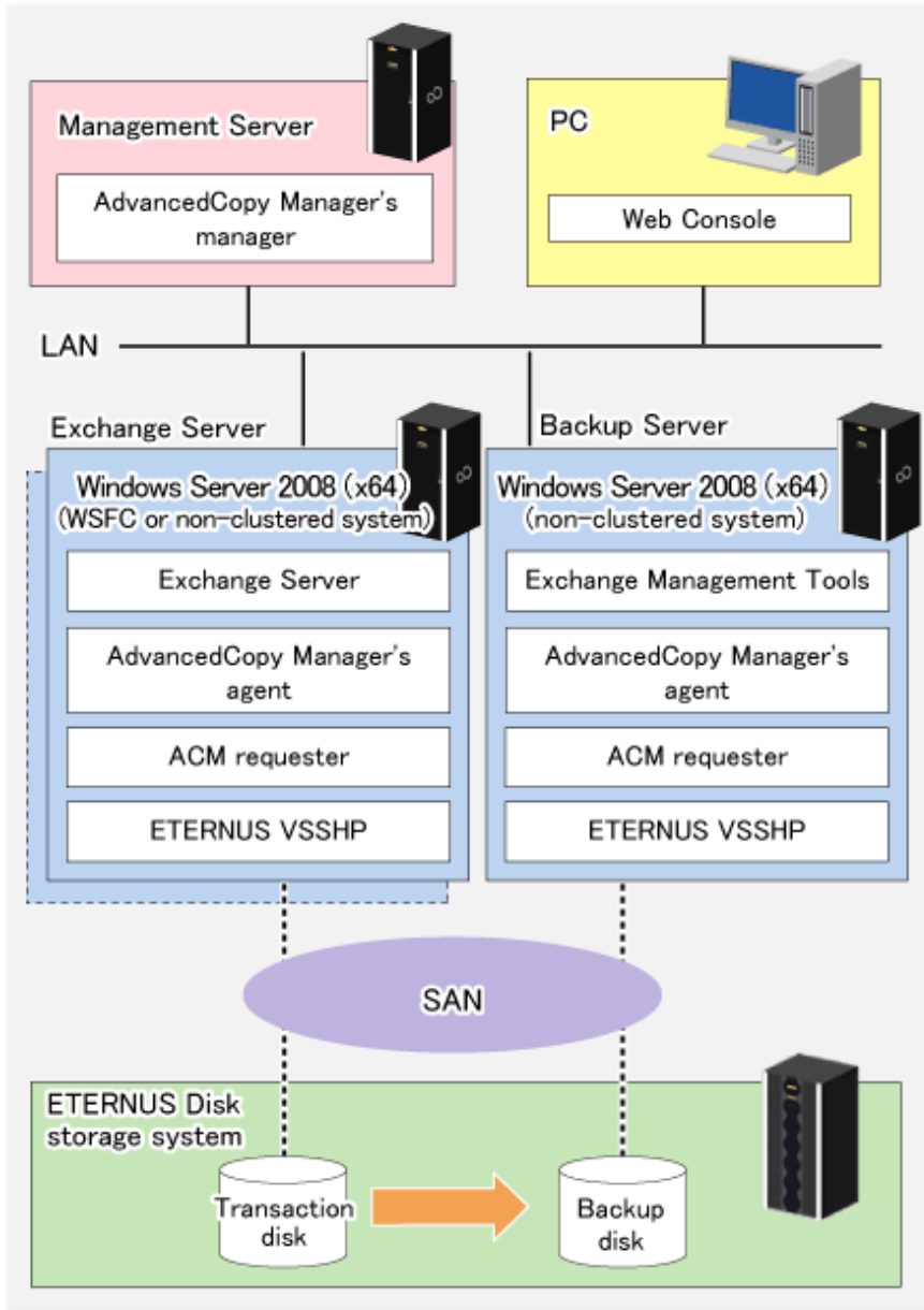
Figure 8.33 System configuration example (For Exchange Server 2007)
