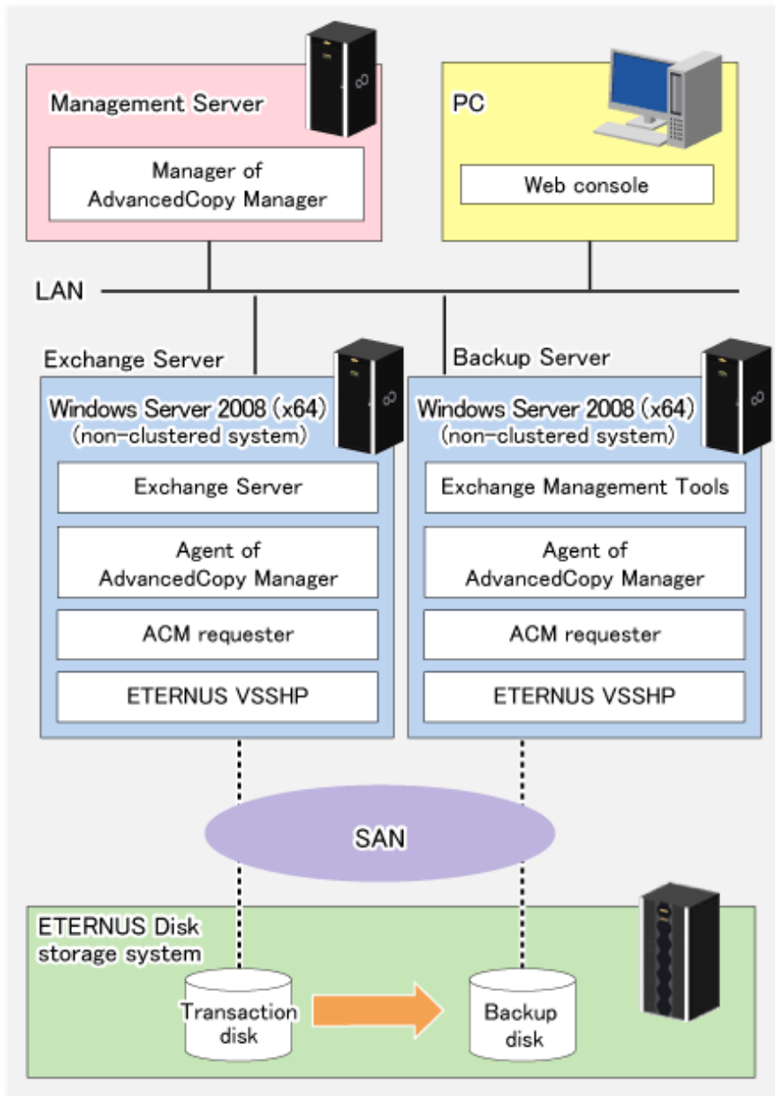
Figure 8.34 System configuration example (For Exchange Server 2010)
