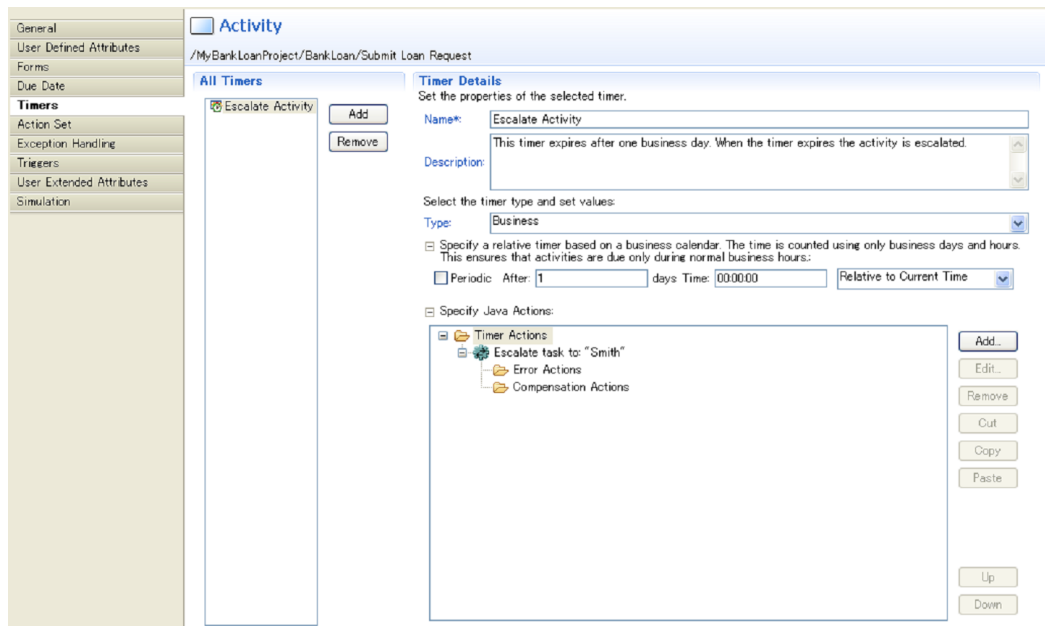
Figure 112: Defining a Timer
