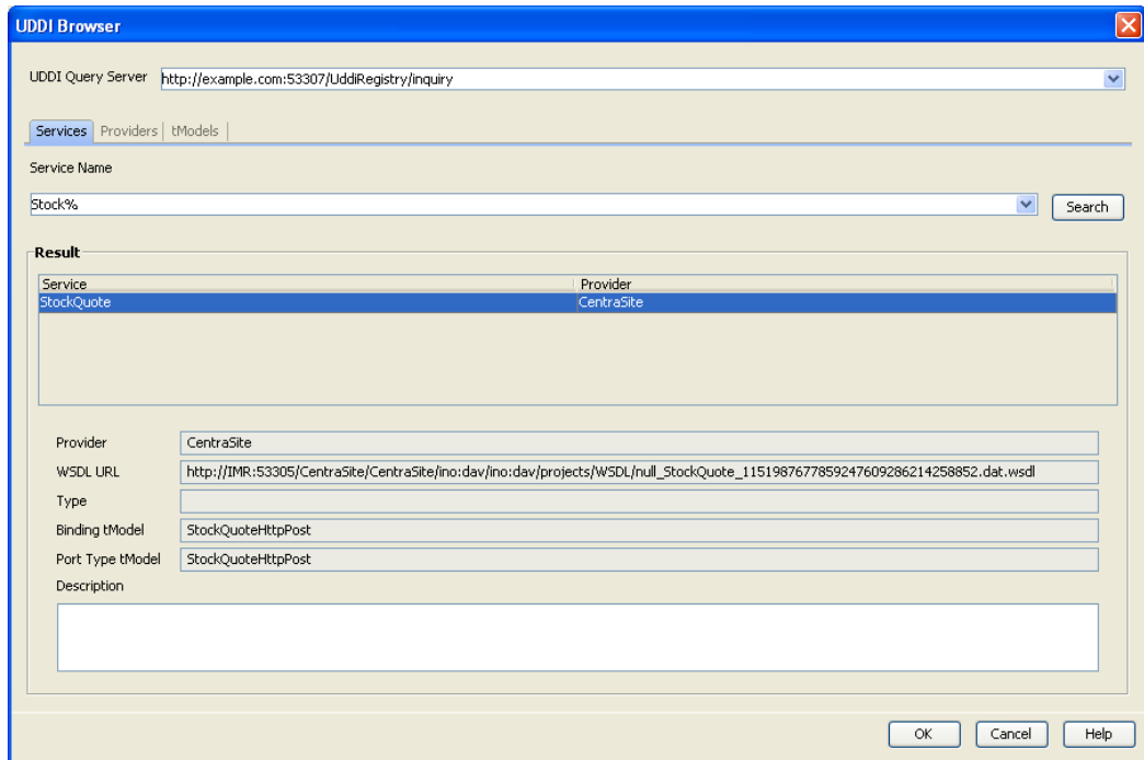
Figure 204: Searching for a WSDL Document
