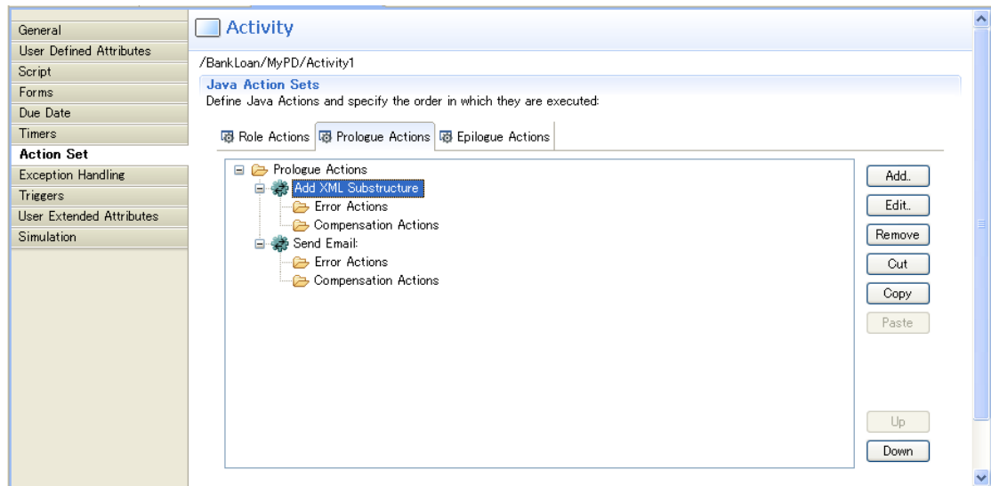
Figure 163: Properties view with Prologue Actions
