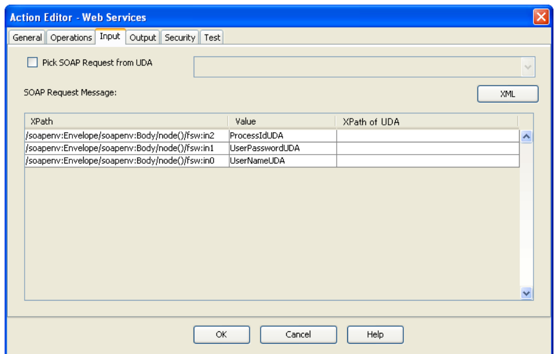
Figure 208: Specifying the Operation's Input Parameters
