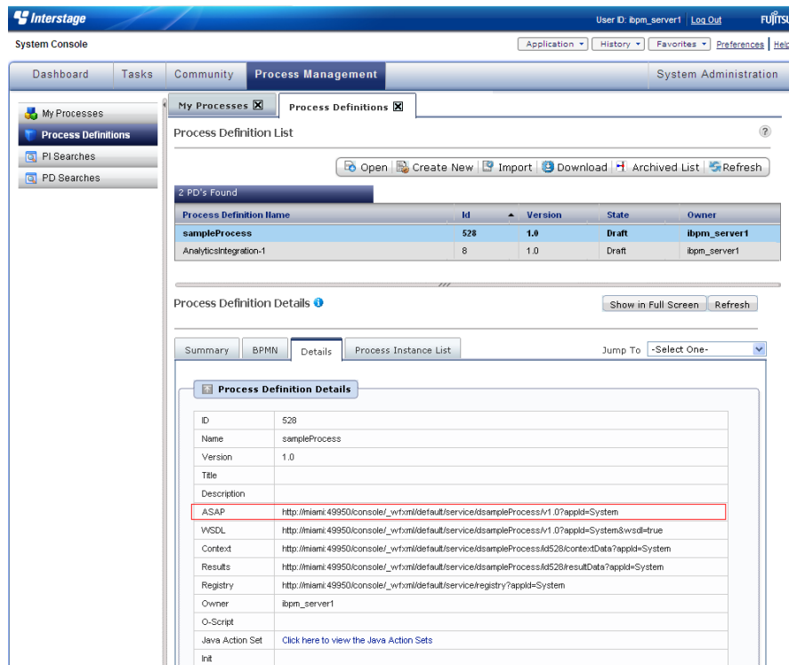
Figure 144: Finding out the URL - part I
