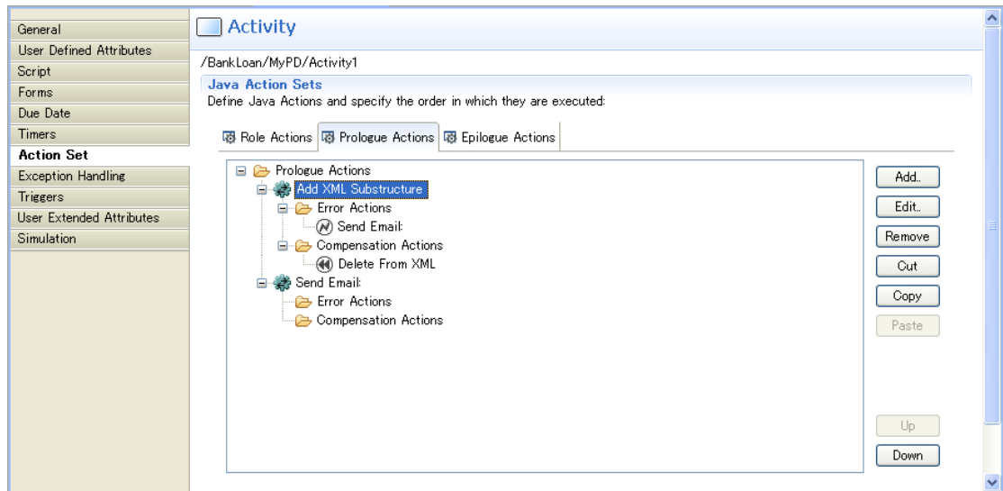
Figure 165: Adding Error and Compensation Actions
