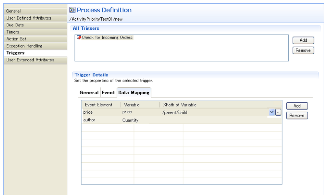
Figure 222: Defining Data Mappings
