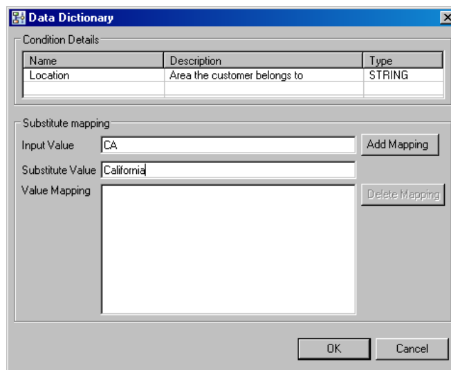
Figure 152: Substitute Mapping CA to California
