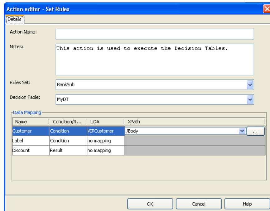
Figure 158: Integrating Decision Tables
