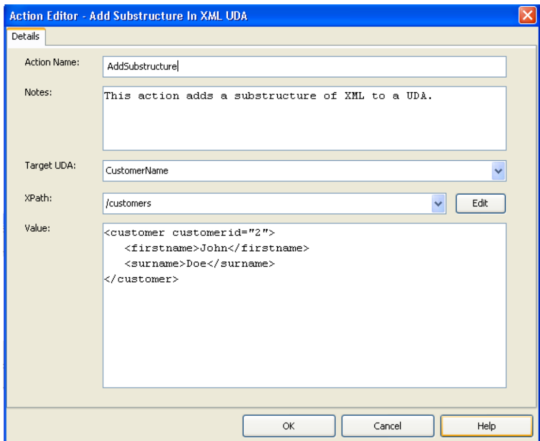
Figure 183: Adding a Substructure in XML UDA
