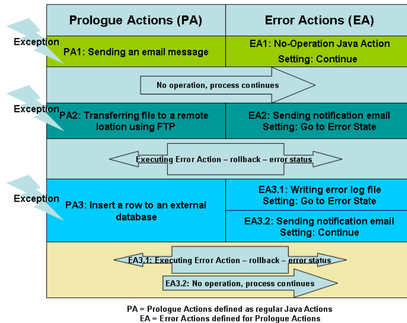
Figure 166: Executing Java Actions and Error Actions
