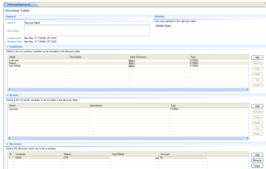
Figure 150: Creating a Decision Table
