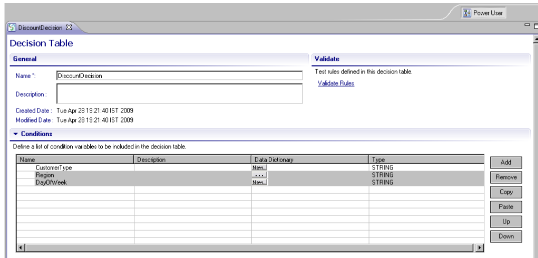
Figure 151: Adding a Condition
