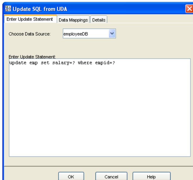
Figure 201: Specifying the Data Source and an SQL Statement
