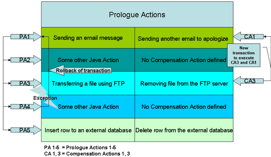
Figure 167: Executing regular Java Actions and Compensation Actions
