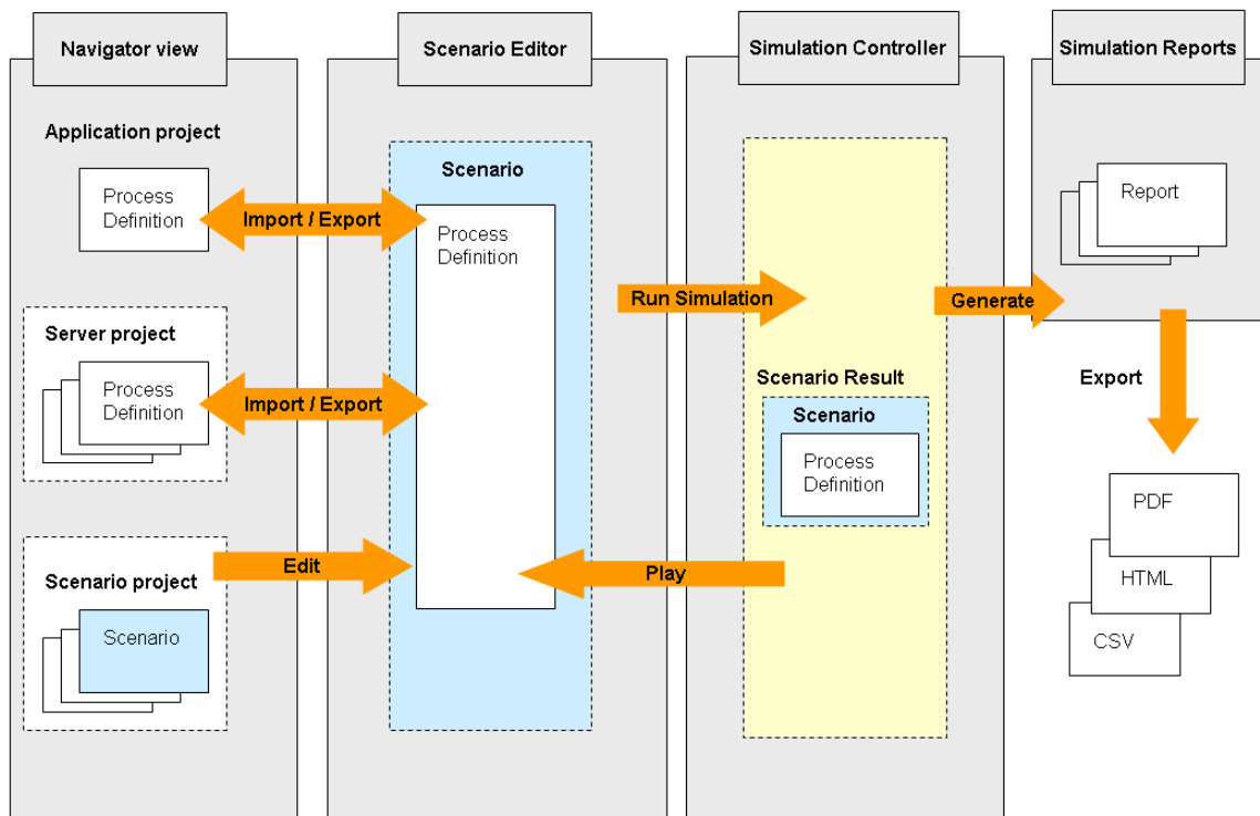
Figure 231: Simulation Process Overview
