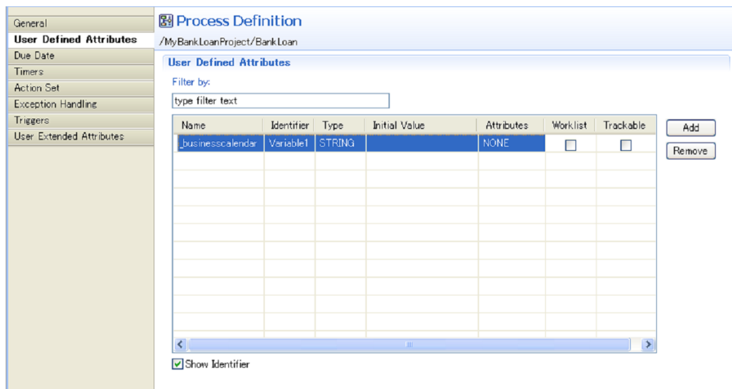
Figure 115: Assigning a Business Calendar
