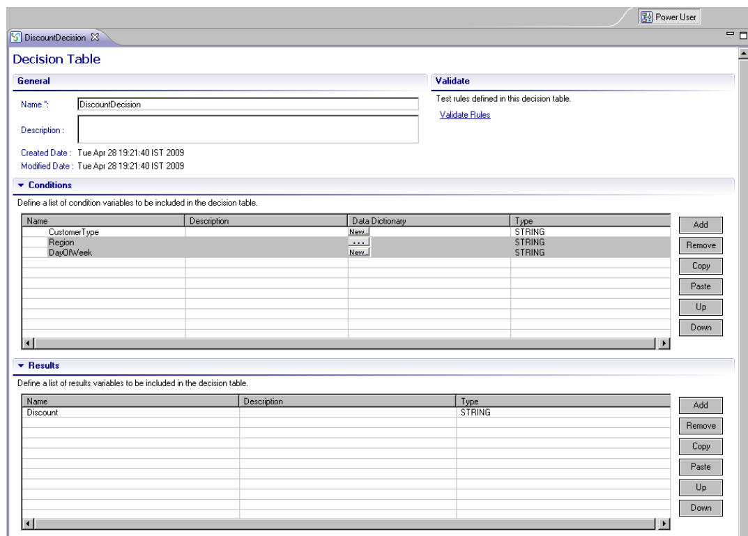
Figure 153: Adding a Result
