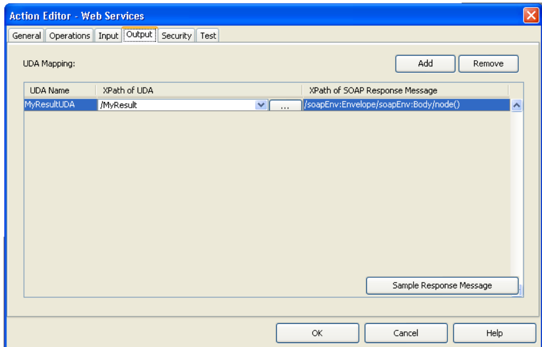
Figure 210: Mapping Return Values to UDAs
