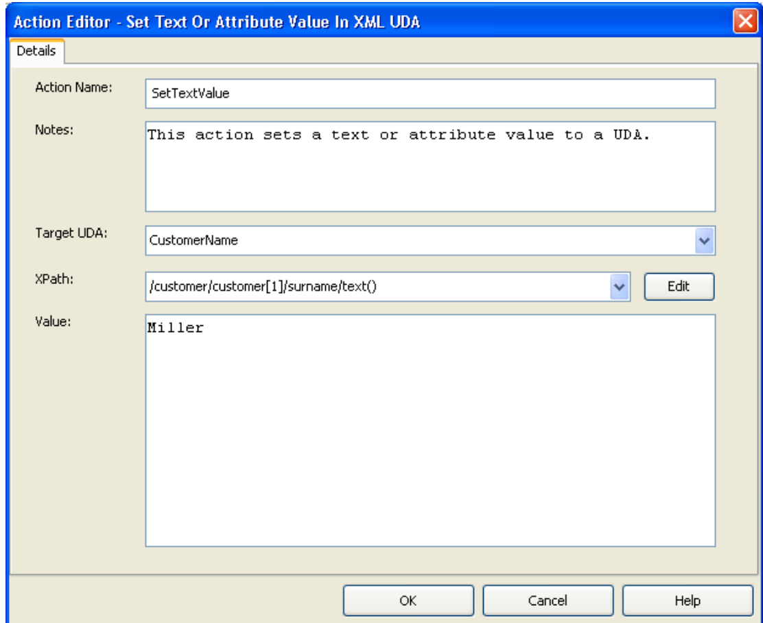
Figure 192: Setting Text or Attribute Values in XML
