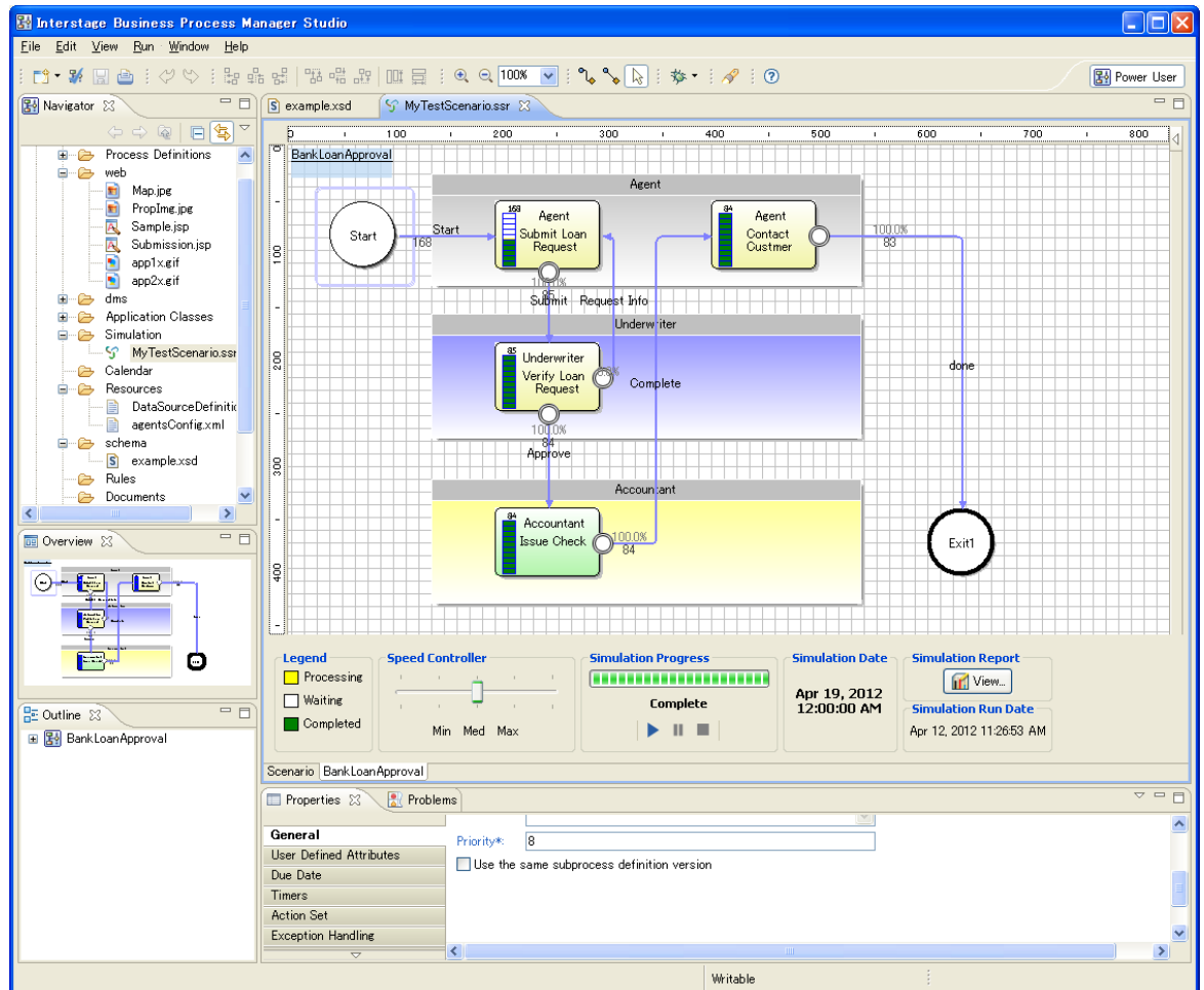
Figure 243: Simulating a process definition
