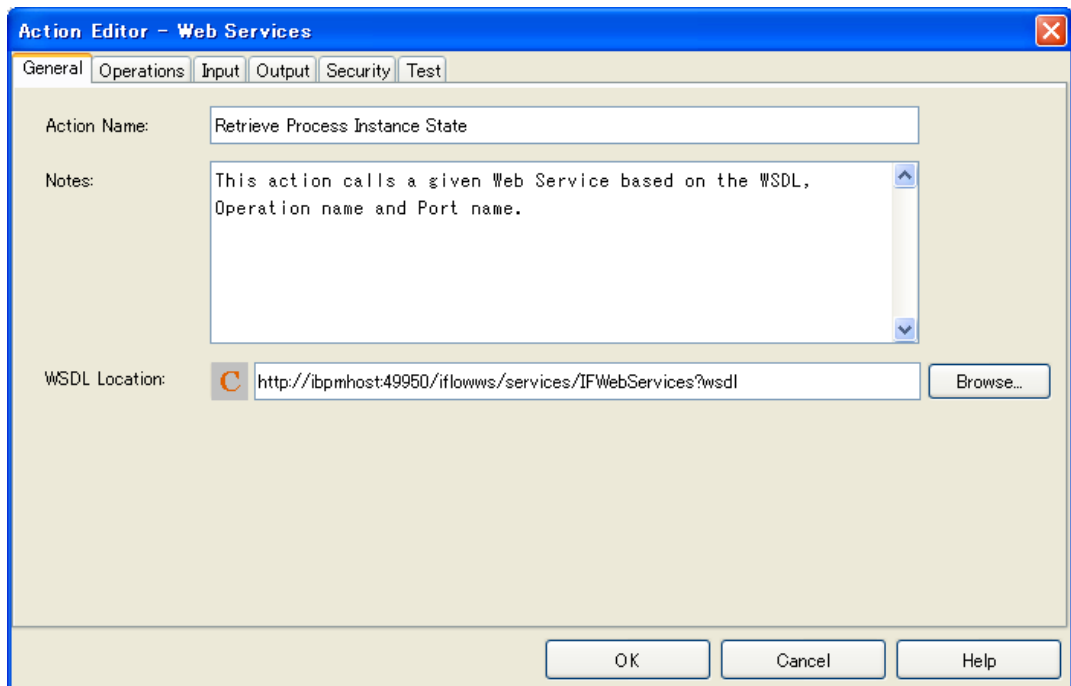
Figure 205: Specifying the Location of the WSDL Document
