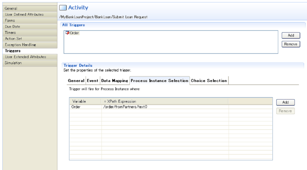
Figure 223: Filtering on process instances
