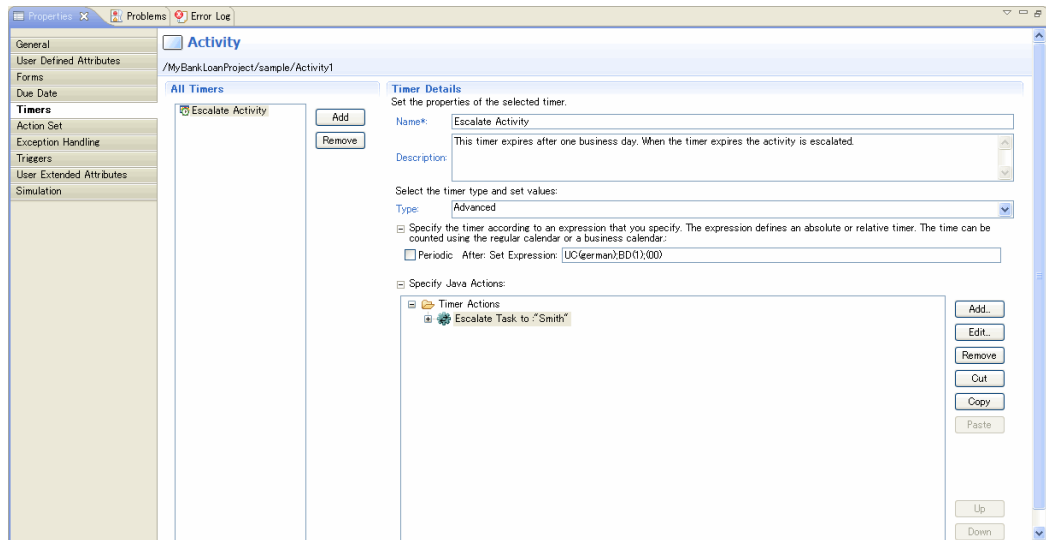
Figure 116: Assigning a Business Calendar to a Timer
