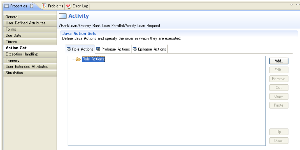
Figure 159: Action Set Tab for Activity Nodes
