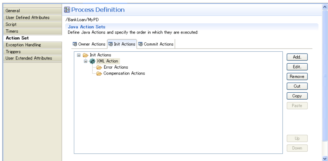
Figure 160: Action Set Tab for Process Definitions
