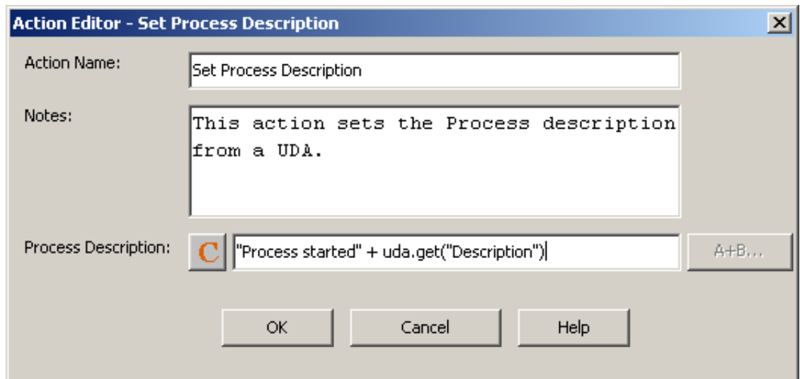
Figure 180: Setting the Process Instance Description
