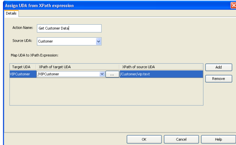
Figure 184: Extracting Data from an XML String - XPath of target UDA
