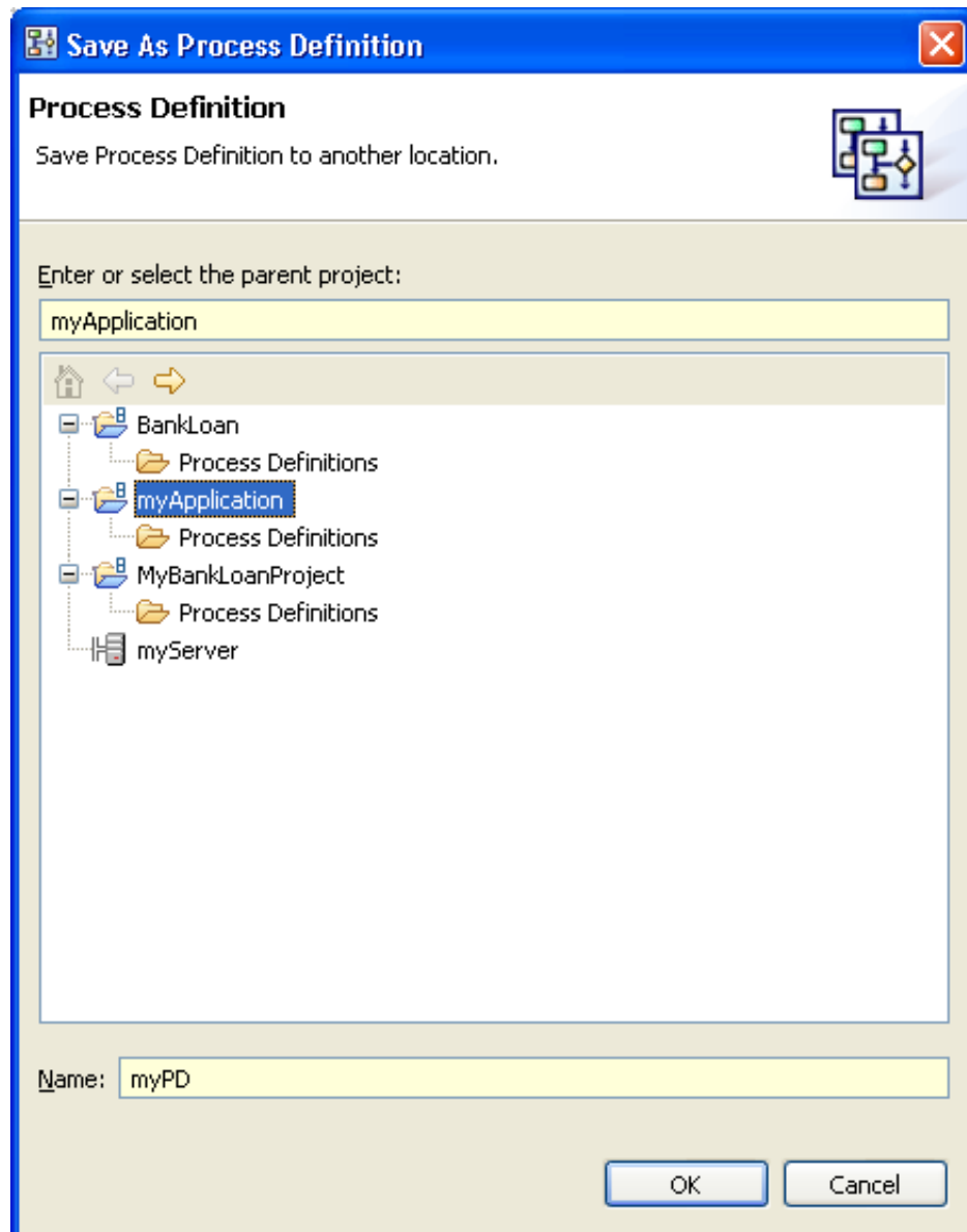
Figure 80: Saving a Process Definition to a Different Name or Project
