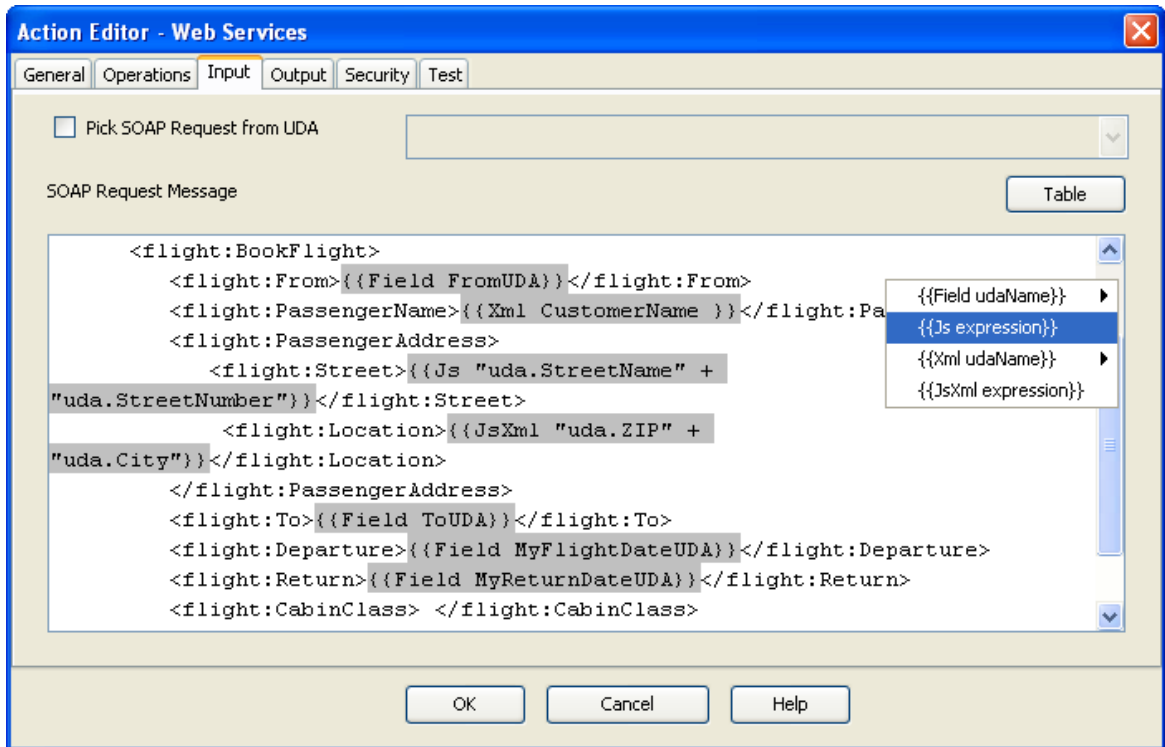
Figure 213: Adding Special Tags for SOAP Request Messages
