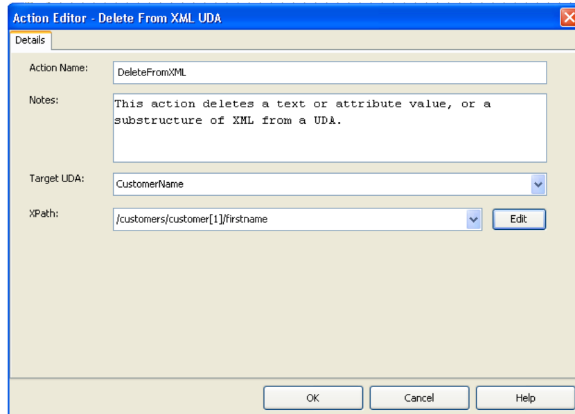
Figure 188: Deleting a substructure
