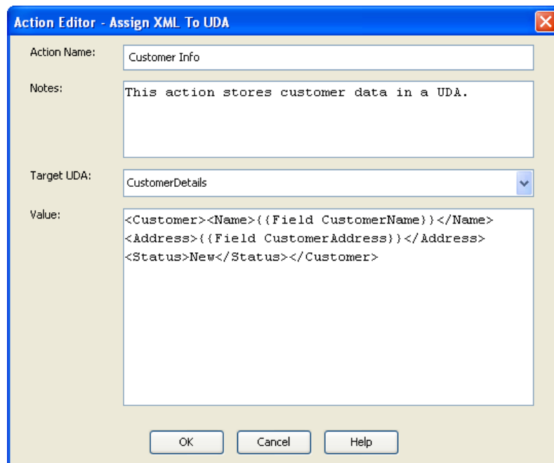
Figure 186: Assigning an XML String to a UDA
