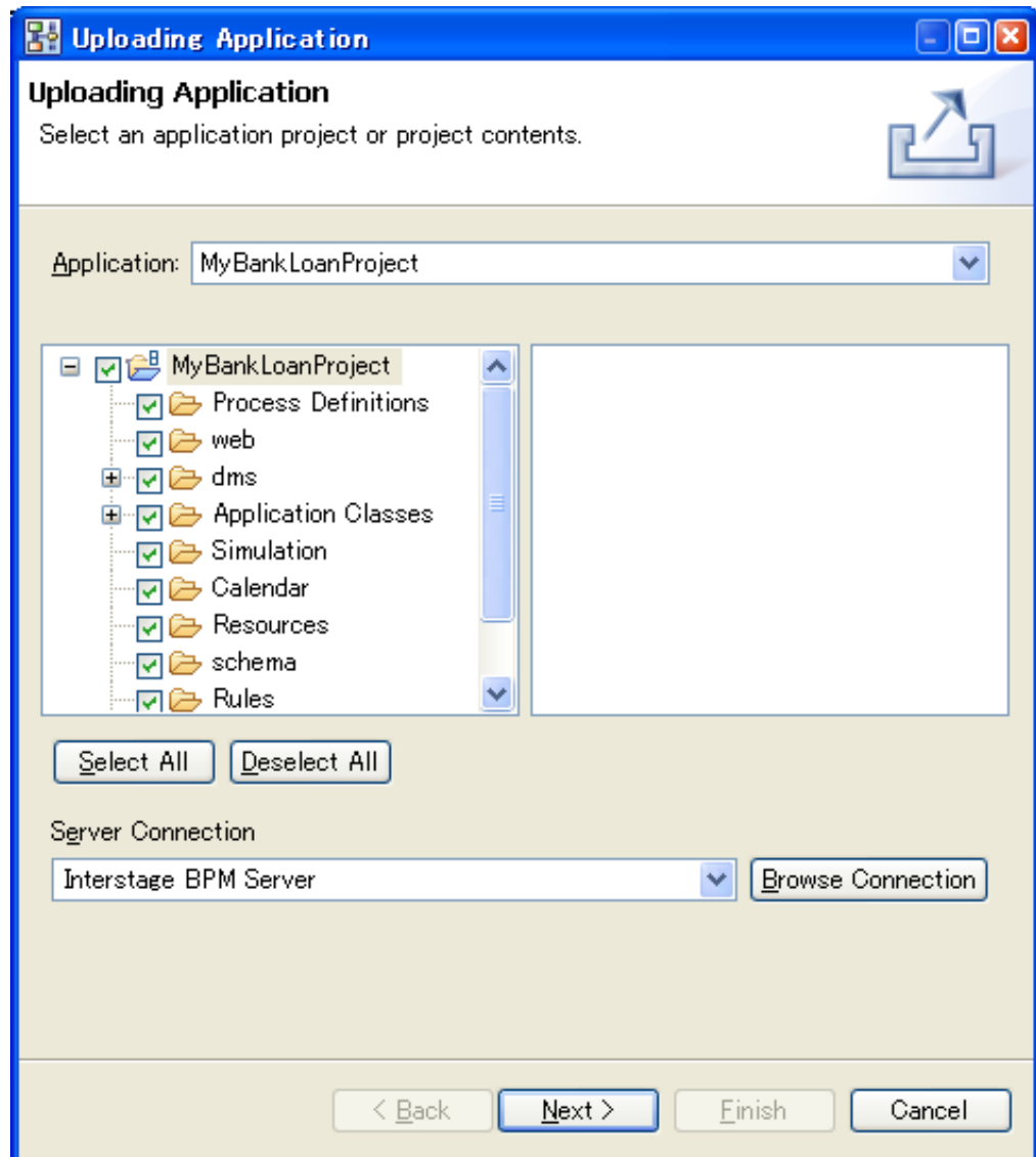
Figure 70: Selecting project components and server
