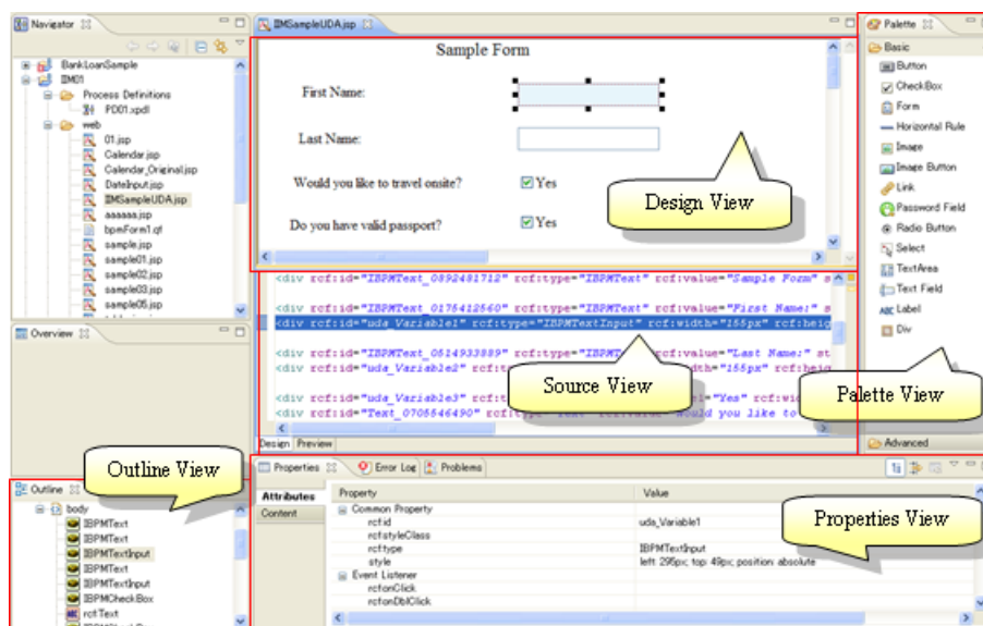
Figure 126: Views of Ajax Page Editor
