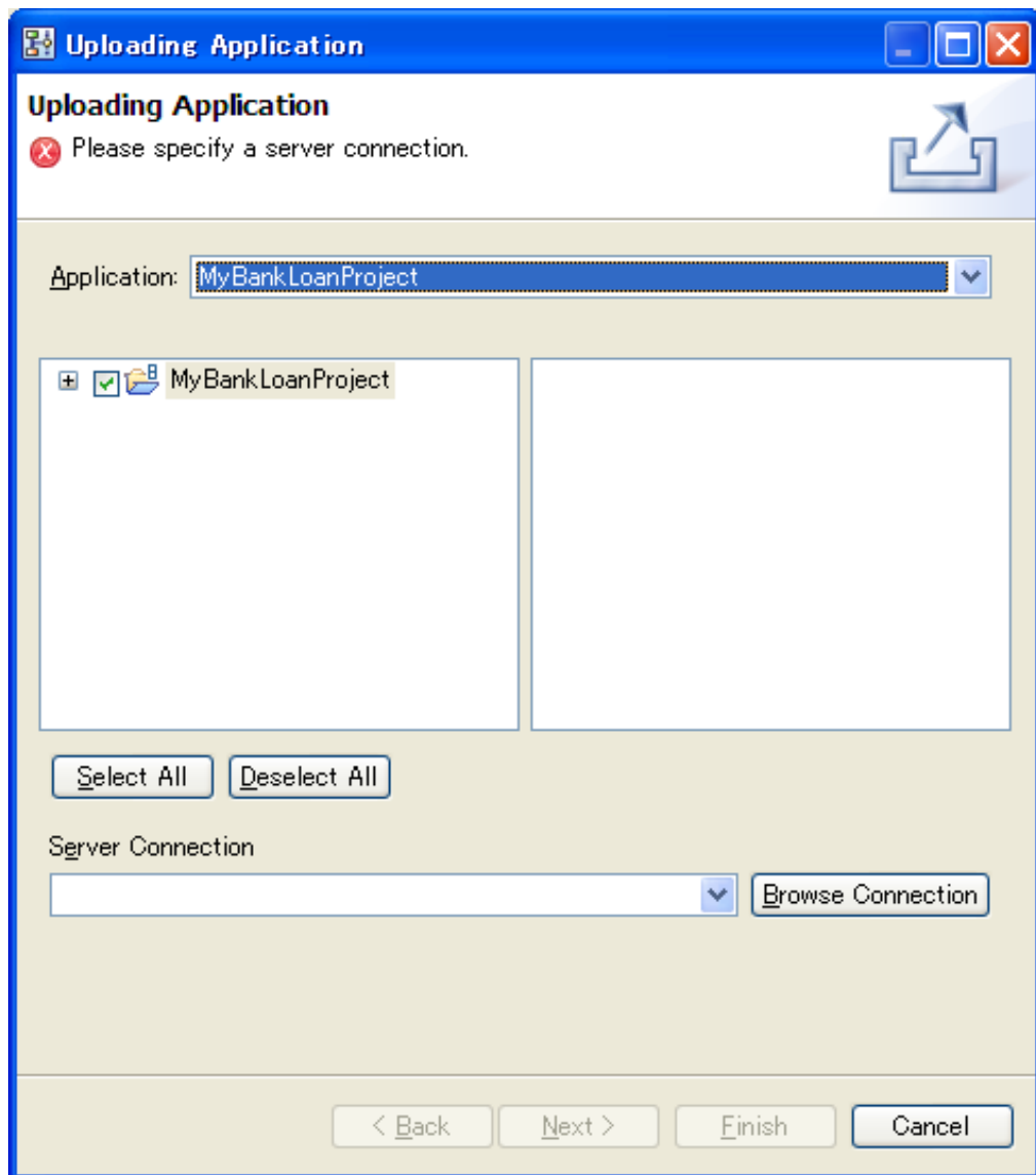
Figure 69: Displaying the Uploading application dialog
