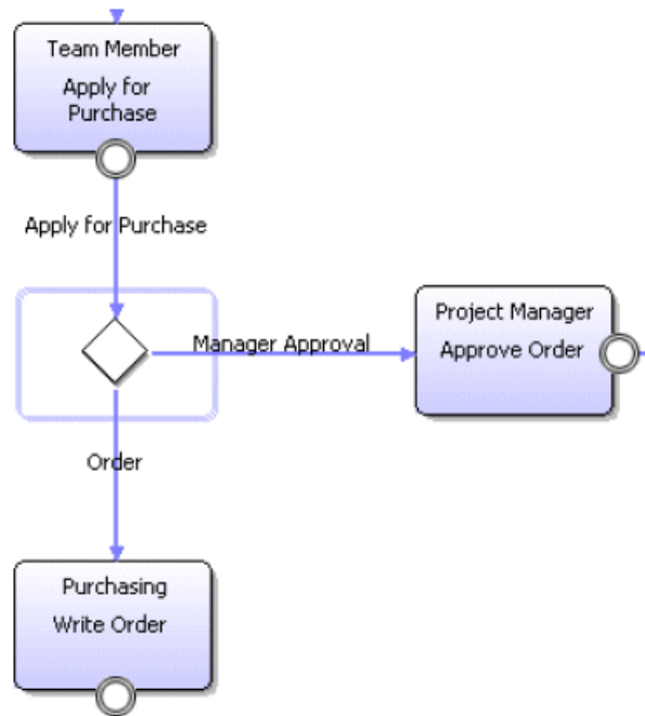
Figure 121: Using Conditional Nodes
