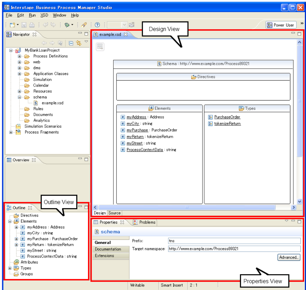
Figure 135: XML Schema Editor
