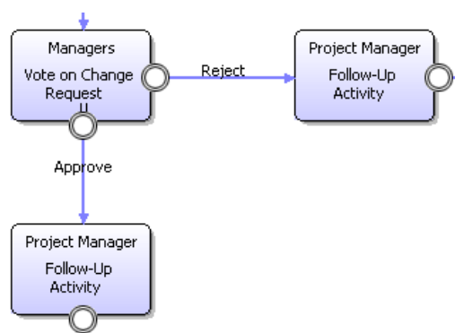
Figure 117: Voting on a Change Request
