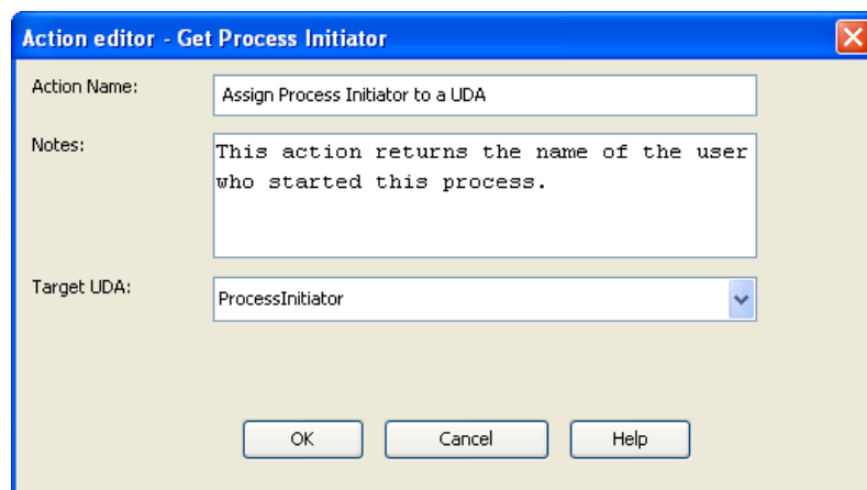
Figure 176: Assigning the Initiator 's Name to a UDA
