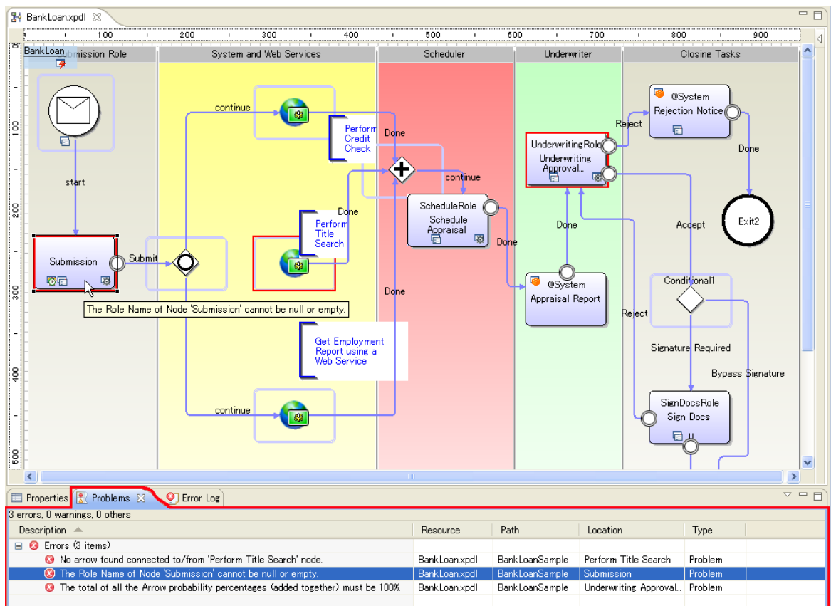
Figure 29: Problems View for a Process Definition
